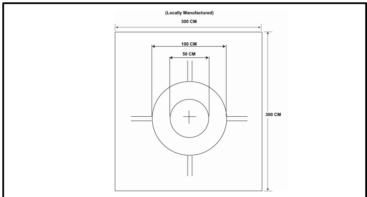
Figure B-17. Zero and bore sight panel
