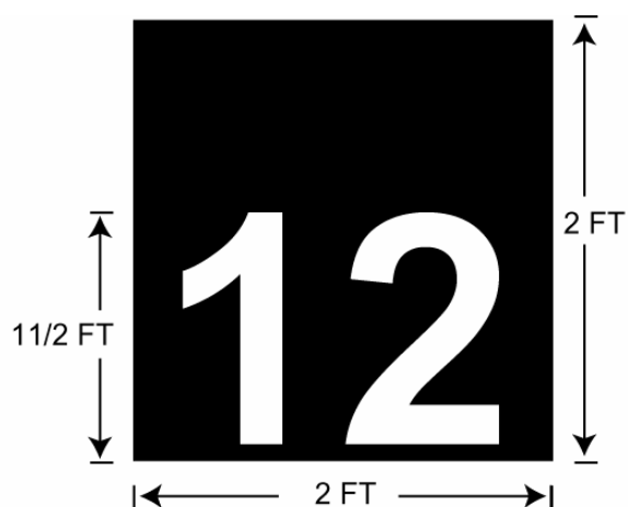
RANGE LANE MARKER UP TO 300 METERS
