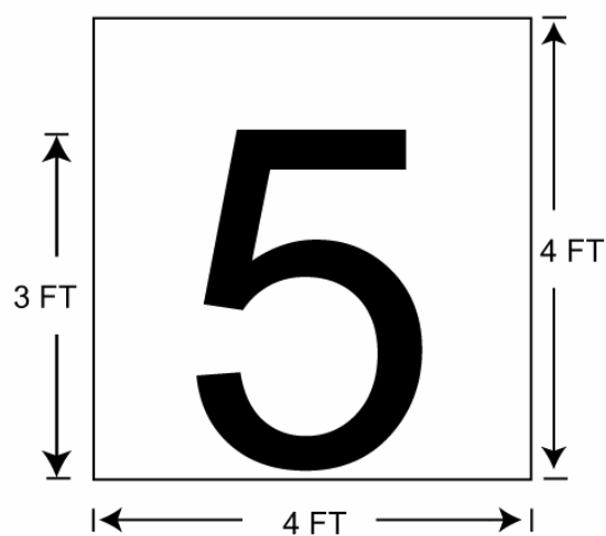
RANGE LANE MARKER UP TO 300 METERS
