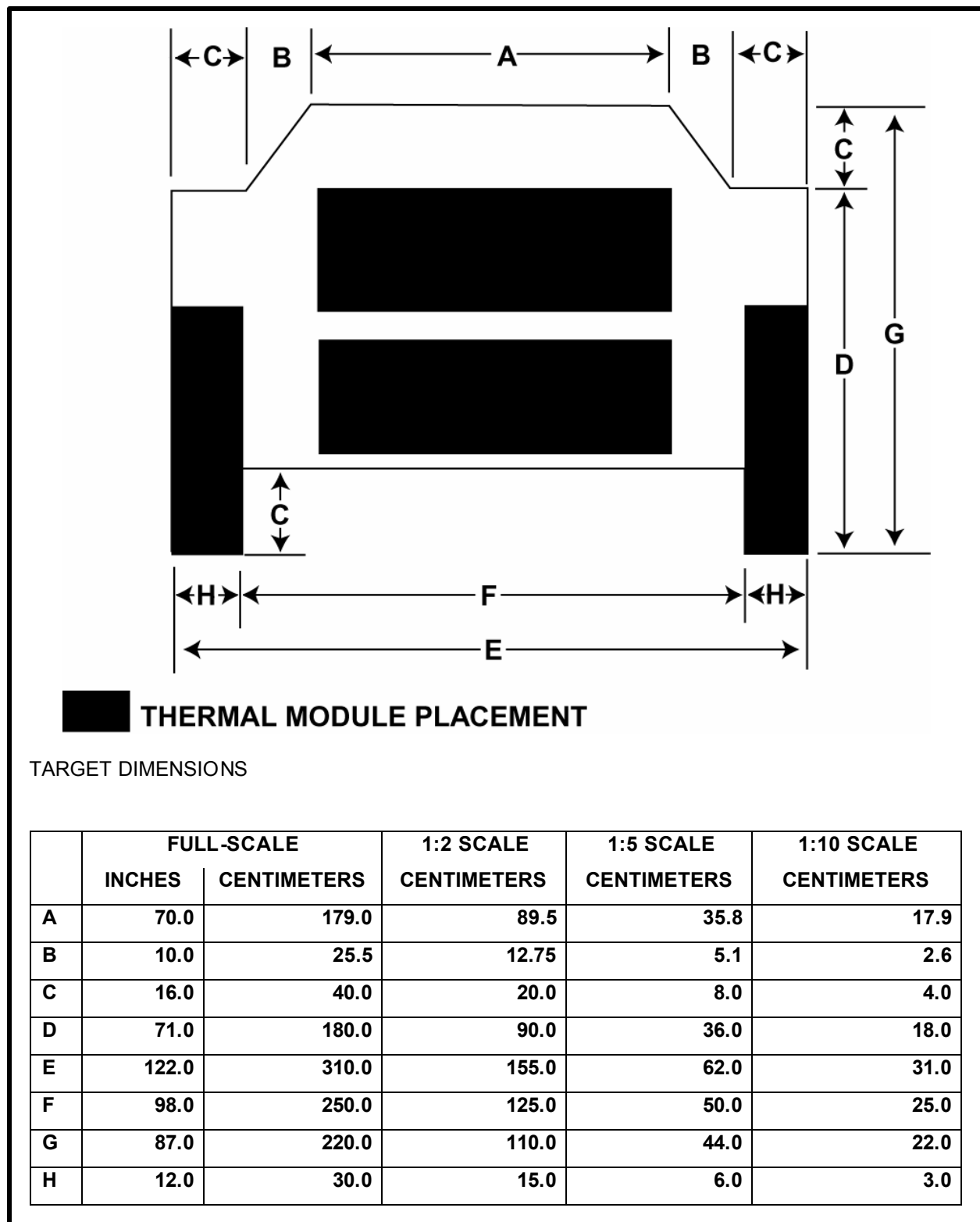
Figure B-31. BMP 1981 front target
