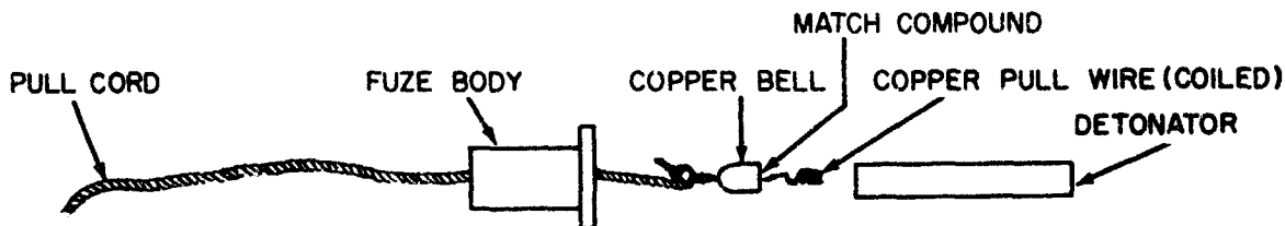
FUZE COMPONENTS
