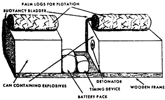
Figure 2-53. Twin can floating mine.
