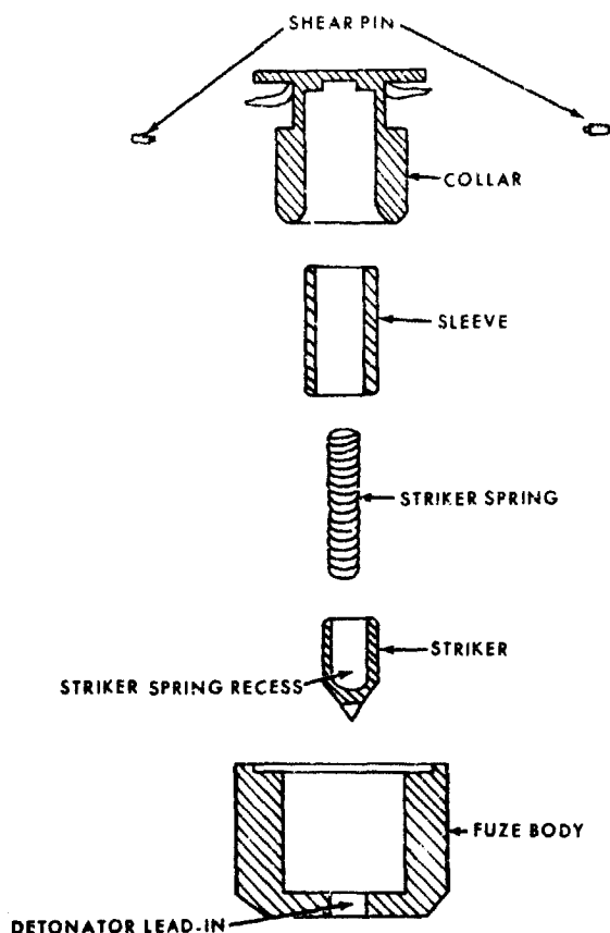
Figure 3-6. Chinese Communist pressure/pull fuze.
