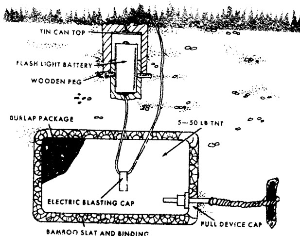
Figure 2-10. Typical locally fabricated VC mine (electrical detonation).
