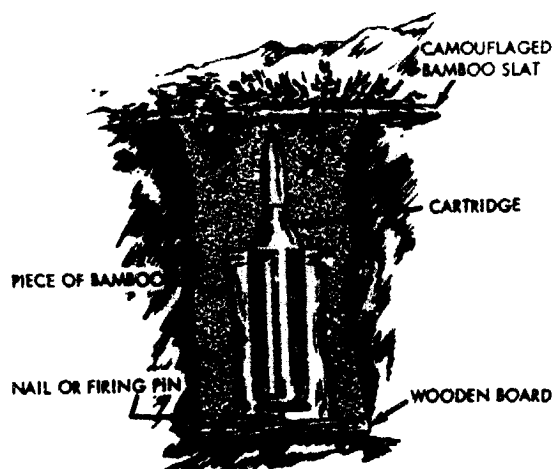
Figure 4-23. Cartridge trap.
