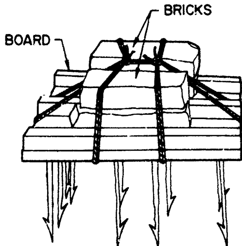
Figure 4-54. Suspended spikes.
