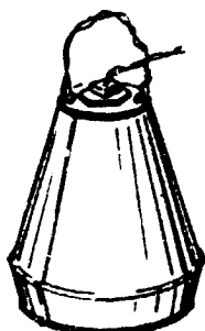
Figure 2-39. Viet Cong small shaped charge mine.
