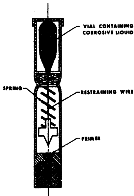
Figure 3-2. Chemical fuze.
