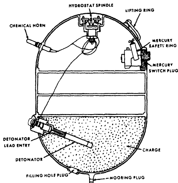
Figure 2-51. Soviet MKB chemical horn contact mine (section view).
