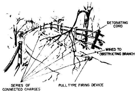
Figure 4-35. Roadside boobytrap.
