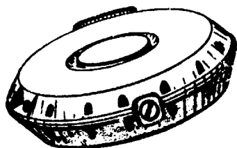
Figure 2-12. Plastic antitank mine PM 60.
