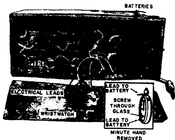
Figure 3-10. Wristwatch firing device.
