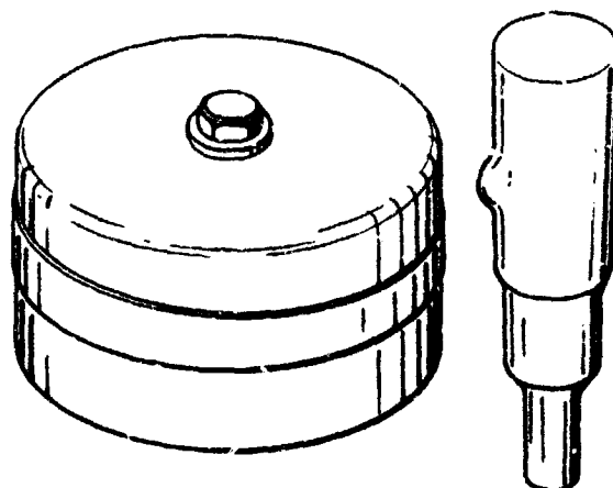
Figure 2-1. Soviet model TMB-2 antitank mine and MV5 fuze.
