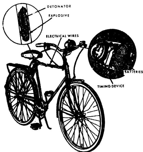
Figure 4-24. Bicycle mine.
