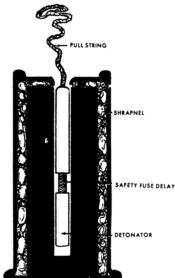
Figure 4-15. Fragmentation explosive device.
