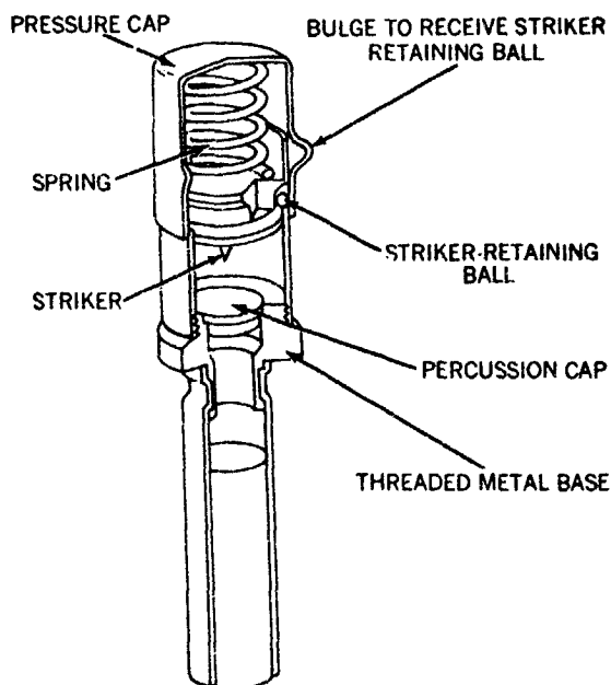
Figure 3-3. Soviet pressure fuze MV-6.
