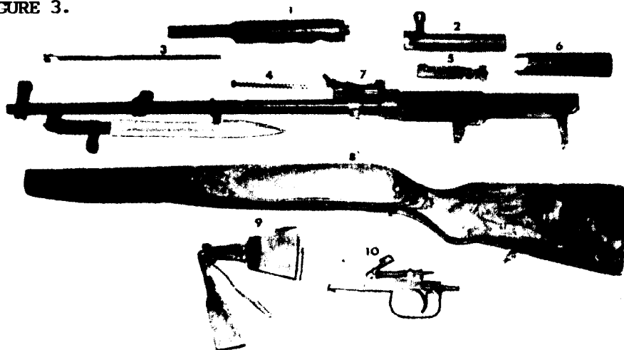
Rifle SKS Soviet
