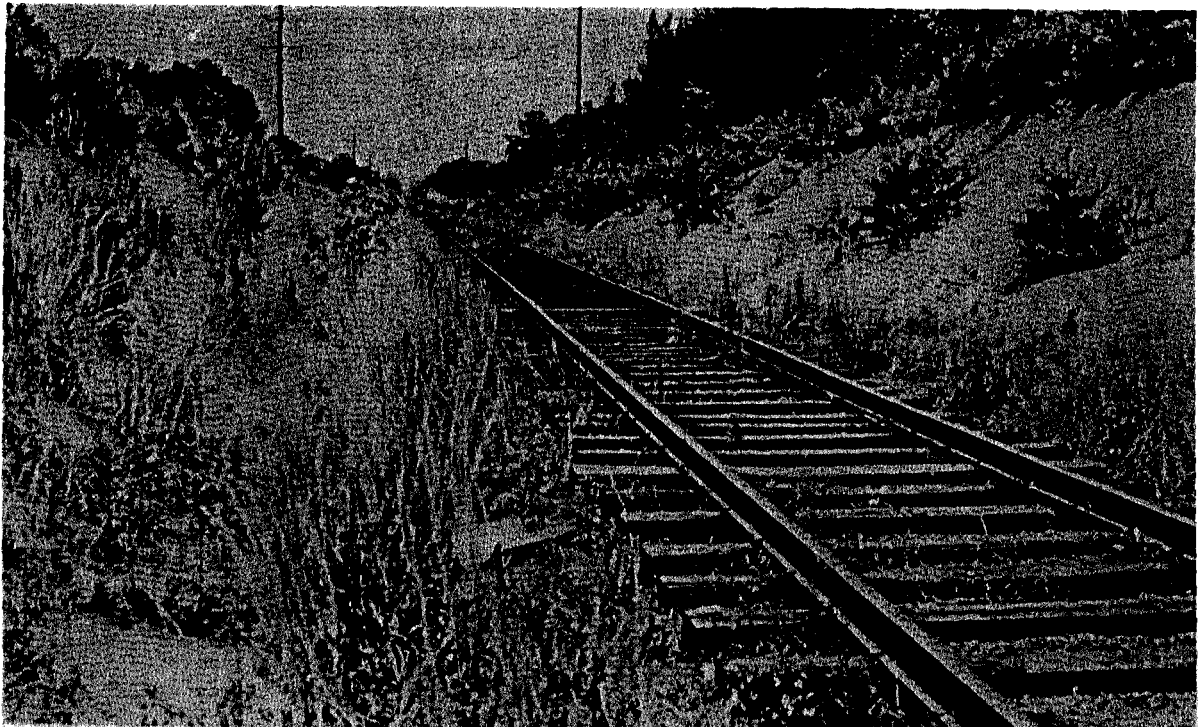
Figure 4-27. Ditches fouled by silt and vegetation.
