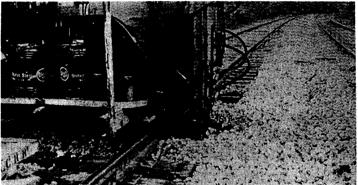
Figure 3-40. Power driven spike driver.
