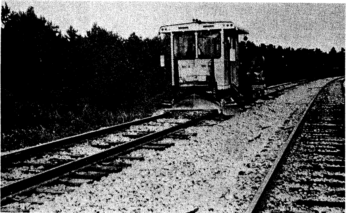
Figure 3-5. Ballast plow.
