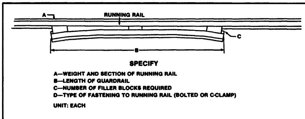
Figure 2-6. Guardrail details
