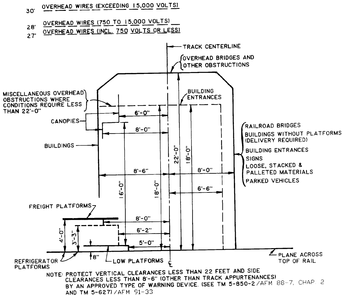
Figure 13-1. Minimum clearances for tangent track.
