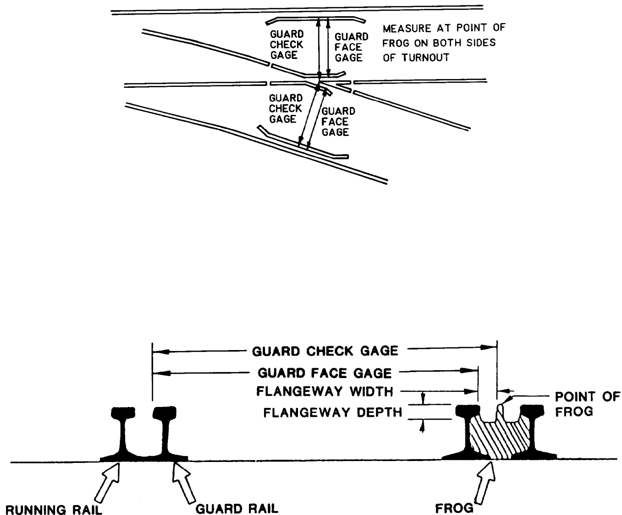
Figure 8-7. Measurement of flangeway width, flangeway depth, guard check gage, and guard face gage.
