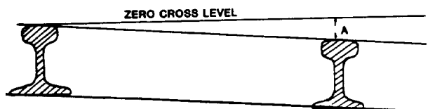
Figure 12-3. Crosslevel measurement.
