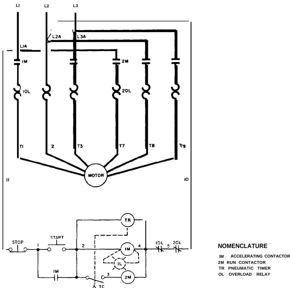
Figure 5-7. Part-winding starter.
