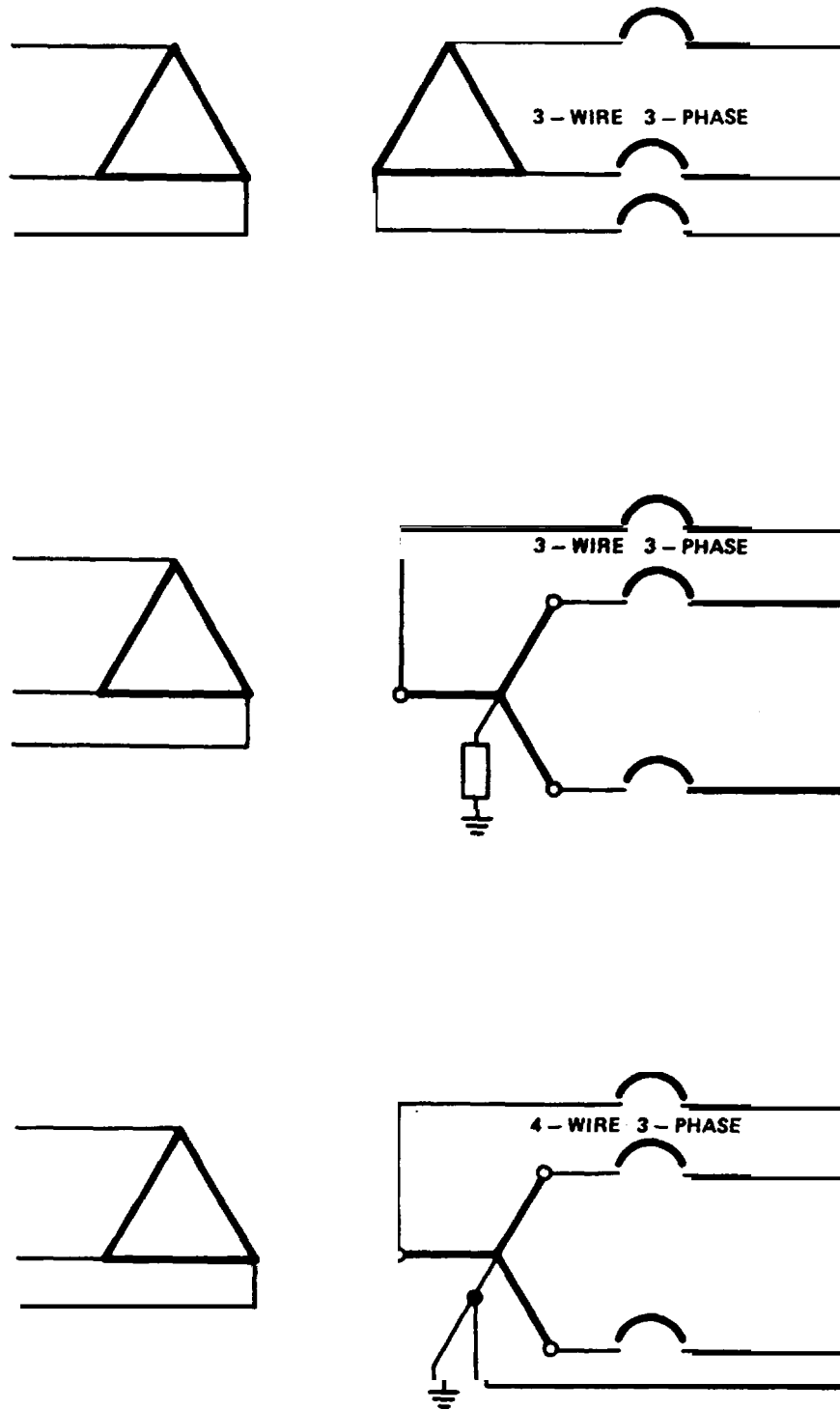
Figure 8-3. Methods of System Grounding: a) Ungrounded, b) High resistance grounded. 480/277V system with 45-50 \Omega resistor rated 1,800 watts continuously, c) Solidly grounded.
