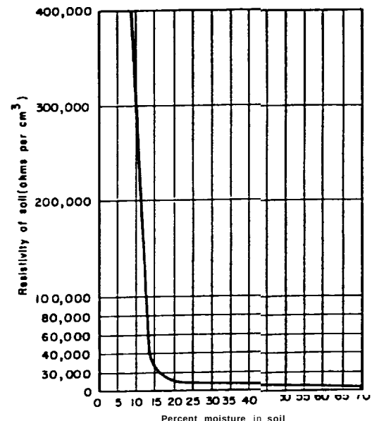
Figure 14-5. Soil resistivity vs. moisture content of red clay soil.
