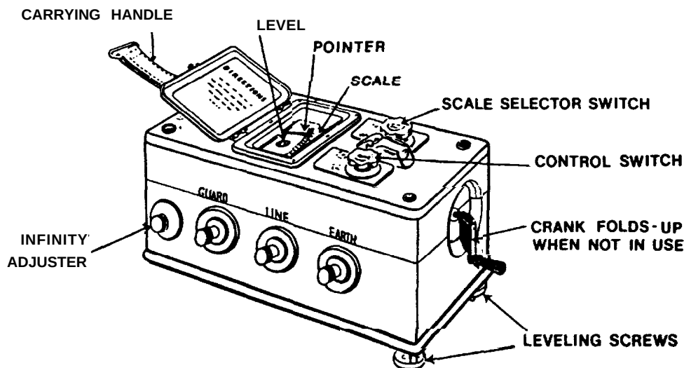
Figure 13-4. Megohmmeter.
