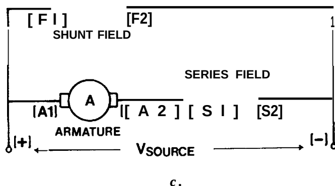
Figure 4-11. Main Types and Connections of DC Motors: a) Shunt motor b) Series motor c) Compound motor
