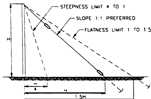
Figure 4-18. Steepness and flatness limits for guy strands
