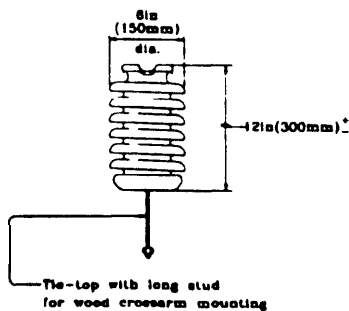
LINE POST, CLASS 57-2L
