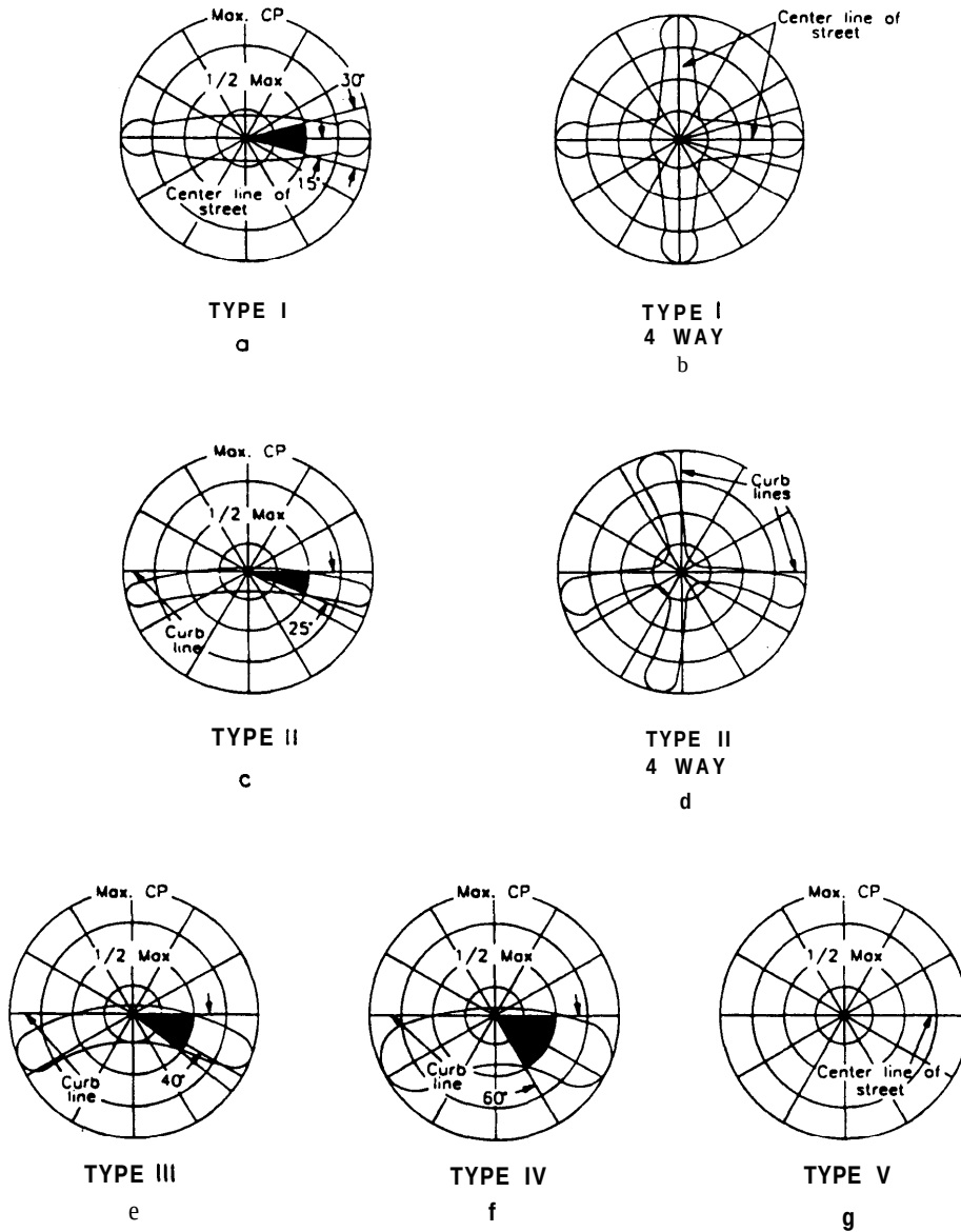
Figure 6-l. Light distribution patterns for roadway lighting
