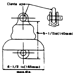
SUSPENSION, CLASS 52 -2
