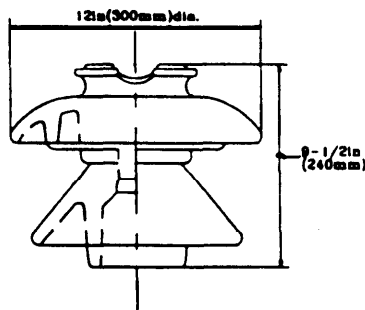
PIN, CLASS 56-4
