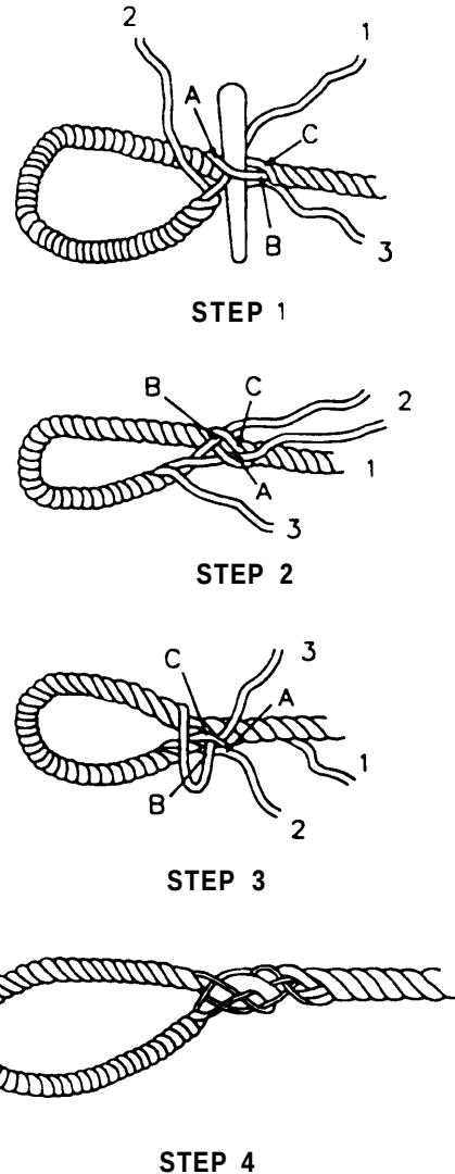
Figure 15-2. Making an eye splice
