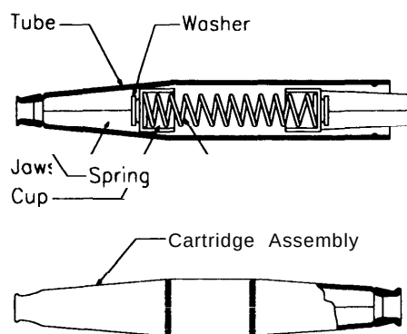
Figure 4-14. Automatic tension splice
