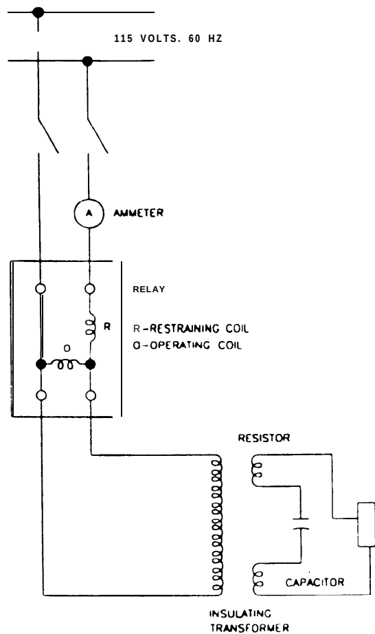
Figure 11-5. Typical test connection for a pilot wire relay
