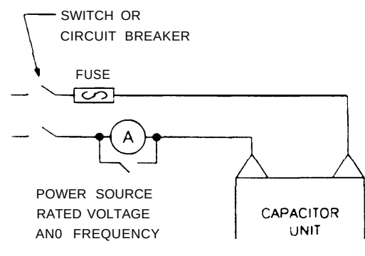
Figure 13-1. Terminal-to-terminal voltage test circuit.
