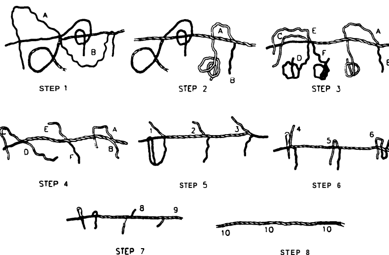
Figure 15-4. Making a long splice
