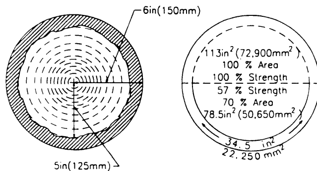
Decay has reduced 12-inches (300 millimeter) pole to 10 inches (250 millimeter) pole with only 70% of cross section (load supporting ability) and 57% of strength (resistance to bending) remaining
