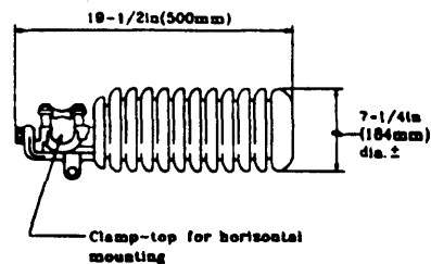
LINE POST SIMILAR TO CLASS 57-14
