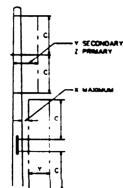
VERTICAL DIMENSIONS OF CLIMBING SPACE COLUMN
