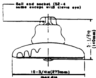
SUSPENSION, CLASS 52-3
