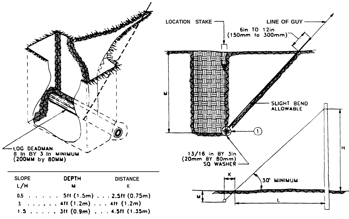
Figure 4-20. Log anchor
