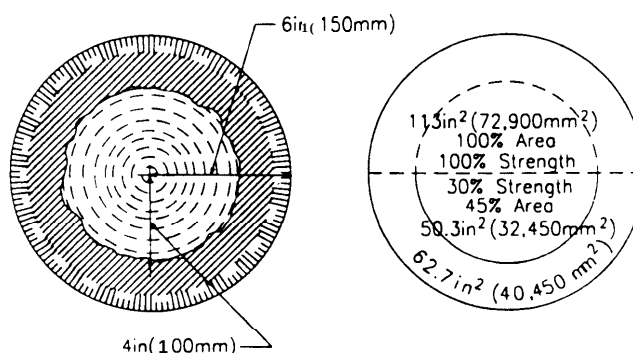
Decay has reduced 12-inch (300 millimeter) pole to 8-inch (200 millimeter) pole with only 45% of cross section (load supporting ability) and 30% of strength (resistance of bending) remaining
