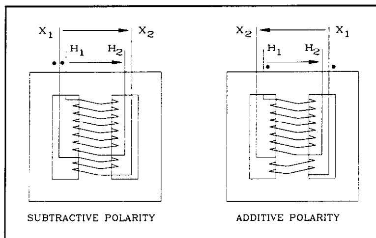
Figure 3-3. Physical transformer polarity.
