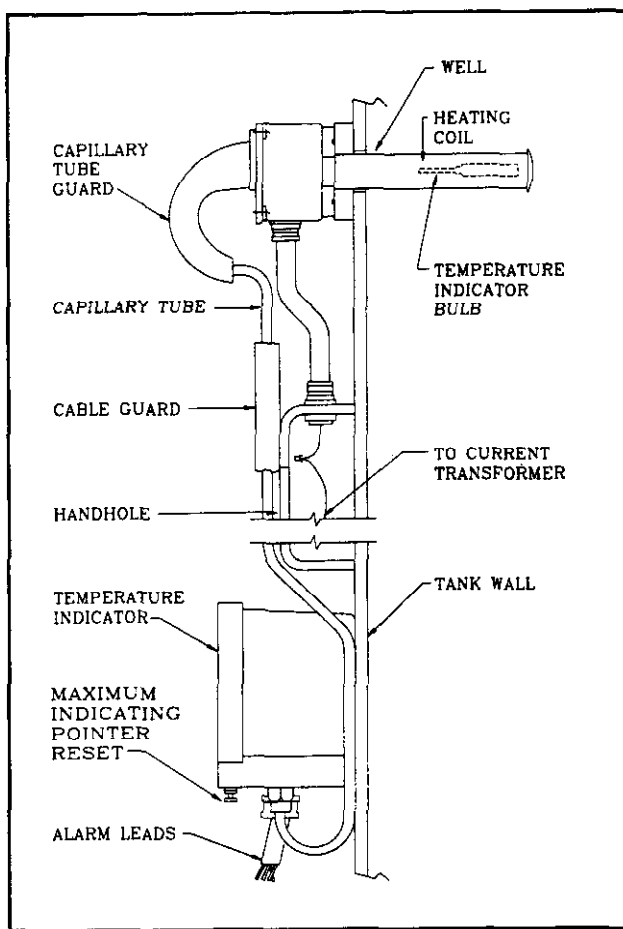
Figure 8-4. Temperature gauge.
