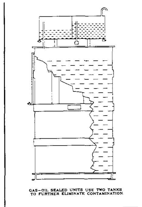
Figure 4-2. Gas-oil sealed transformers.
