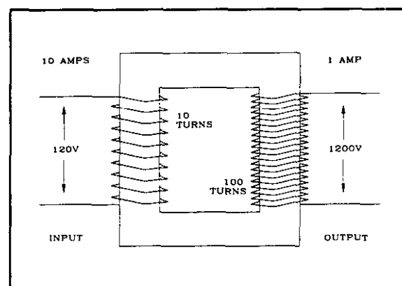
Figure 2-5. Transformer 1:10 turns ratio.
