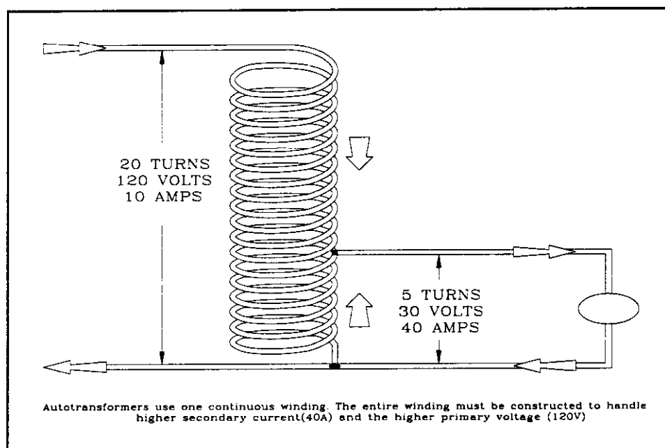
Figure 3-7. Autotransformer.
