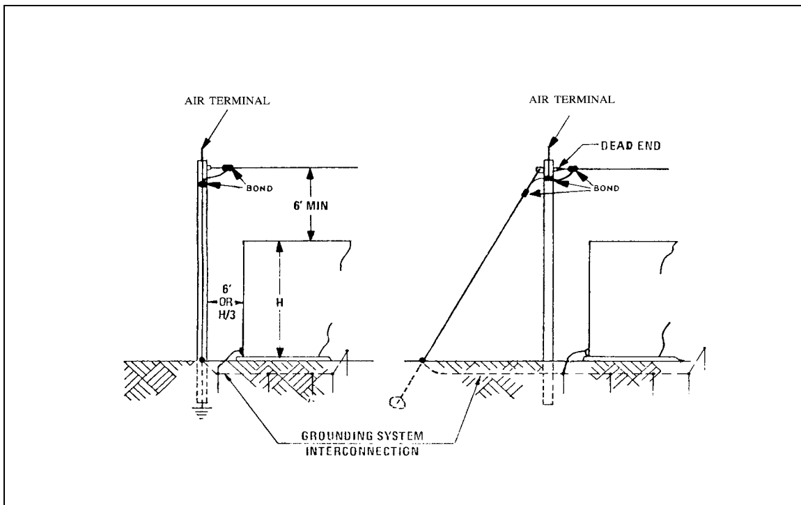
Figure 3-24. Overhead ground wire lightning protection system
