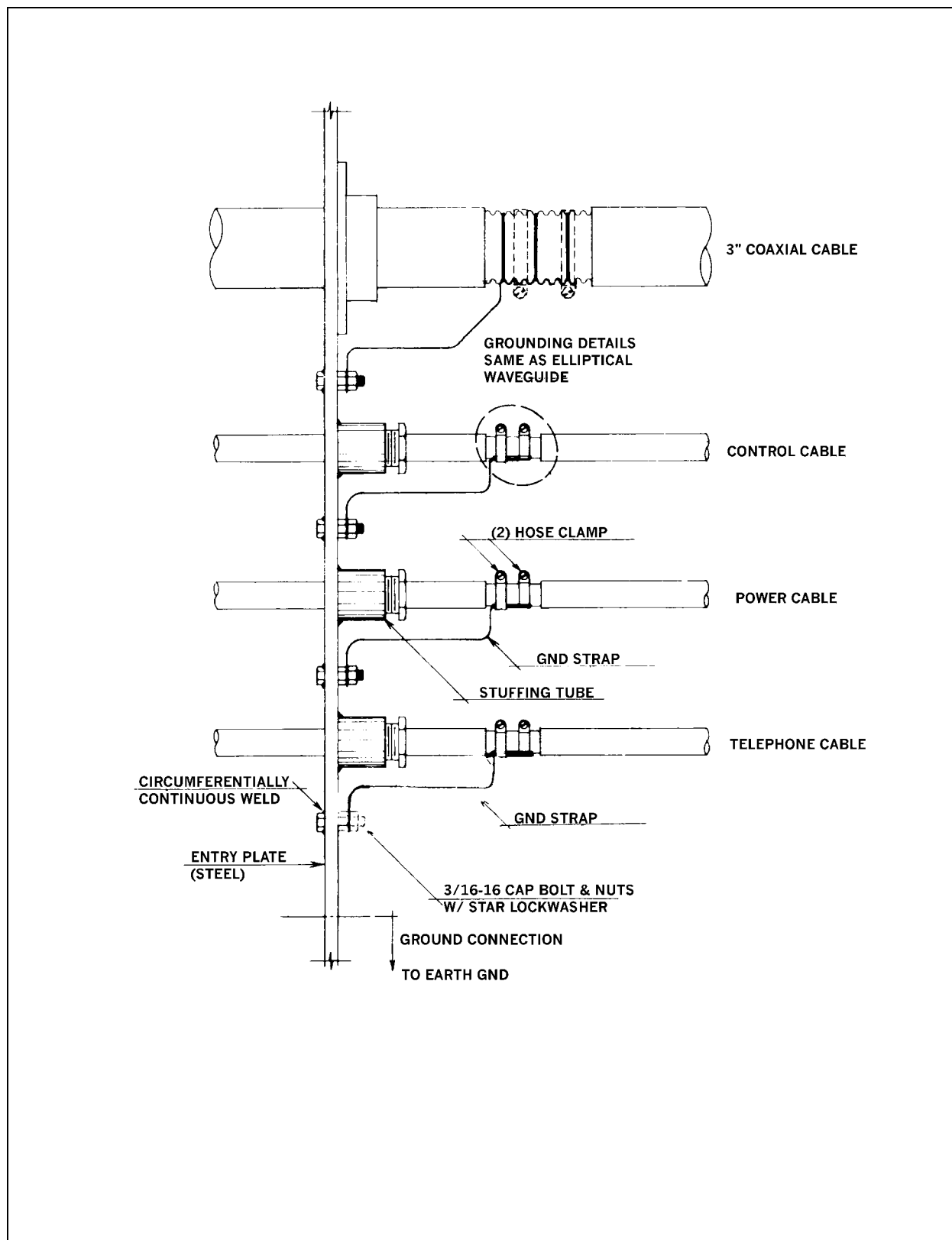
Figure 3-28. Communication cable entry installation
