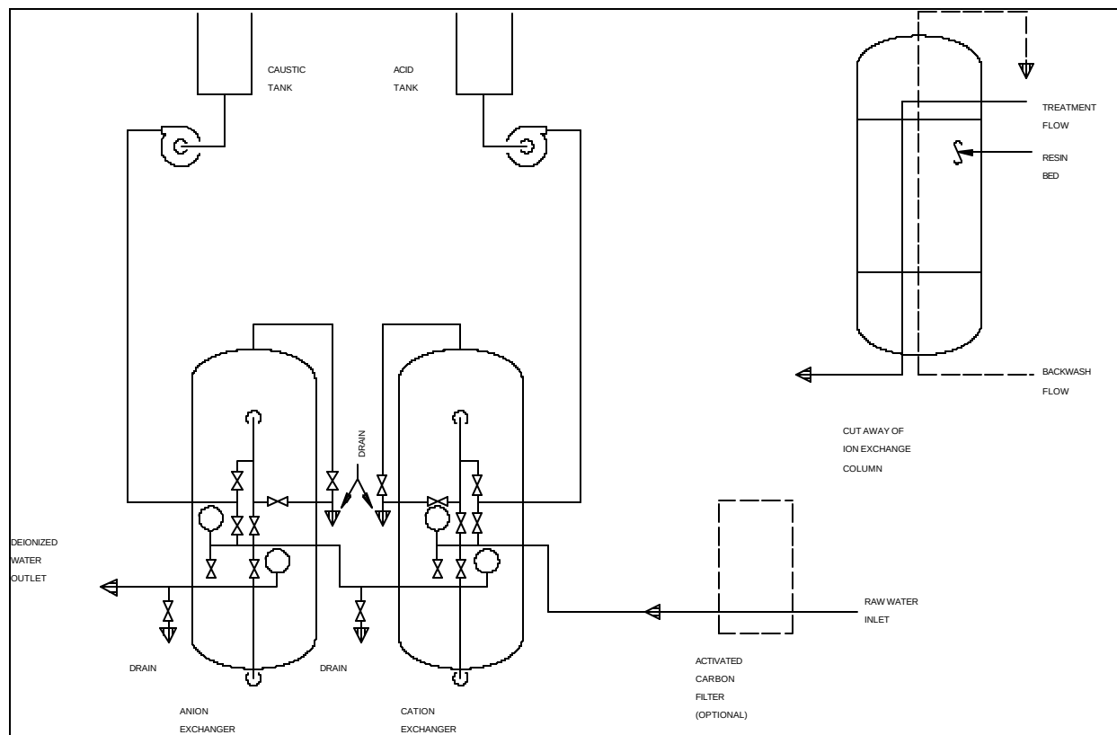
Figure 13-6. Basic ion exchange unit
