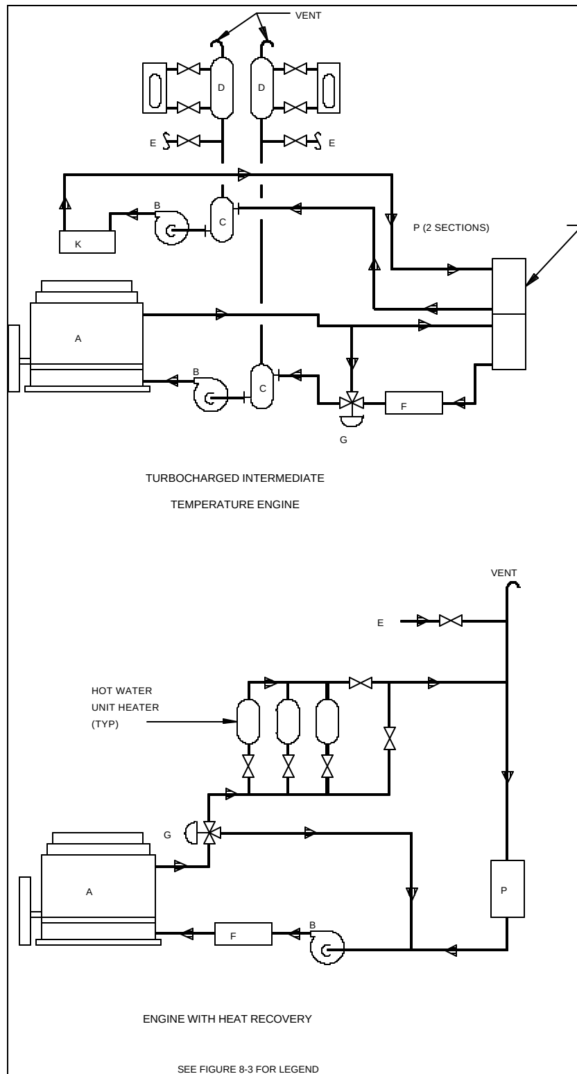
Figure 8-2. Examples of engine cooling systems(2)
