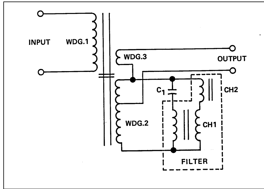
Figure 2 -17. Ferroresonant transformer
