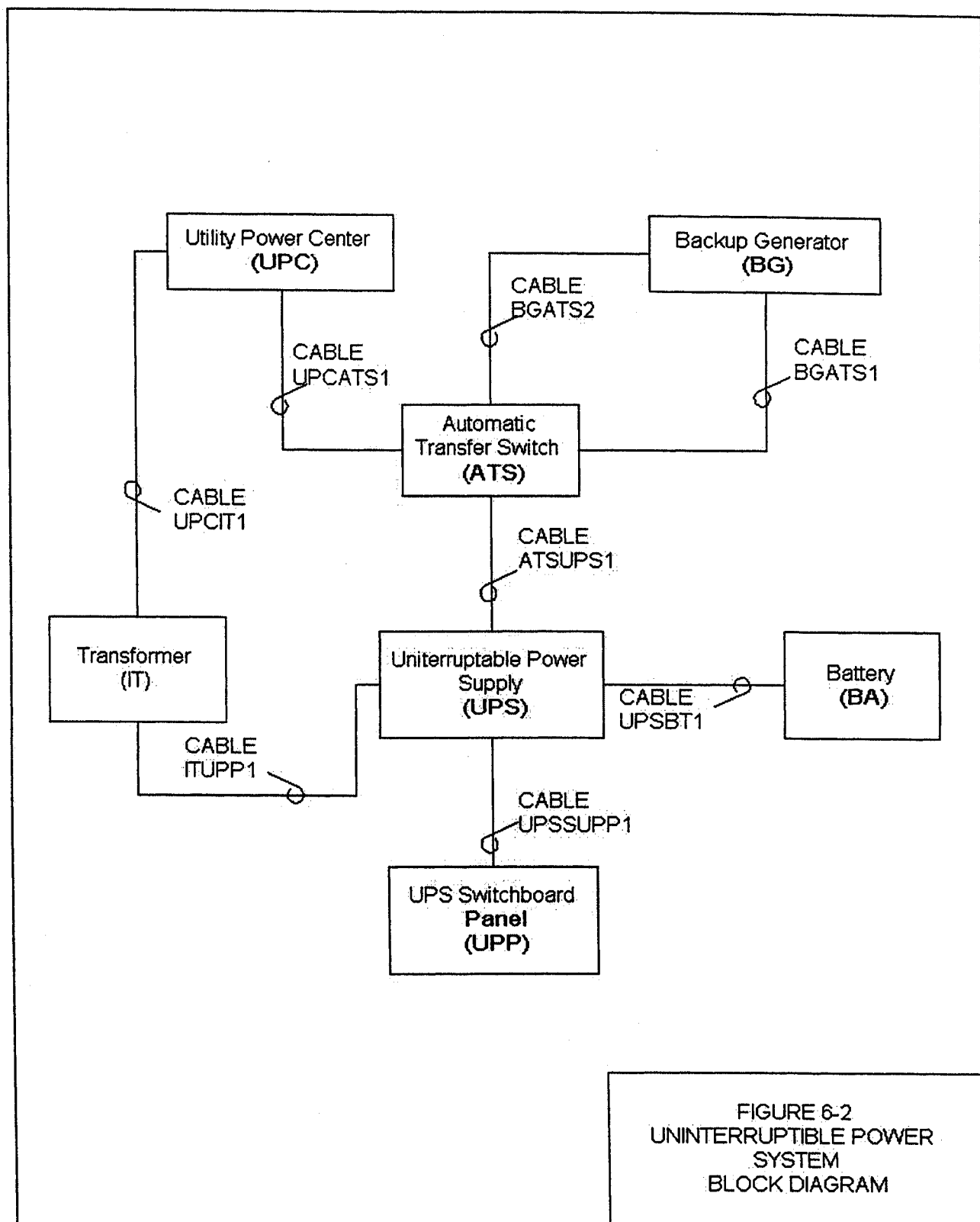
Figure 6-2. Uninterruptible power supply system block diagram
