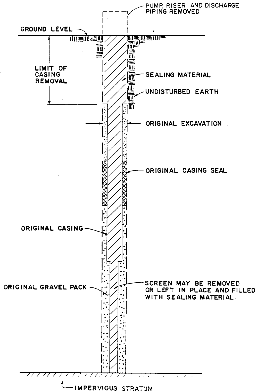
Figure 5-8. Sealed well.
