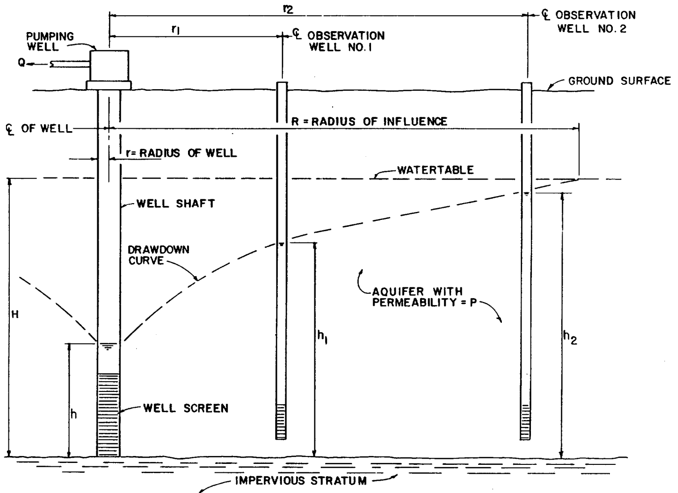
Figure 5-4. Diagram of water table well.
