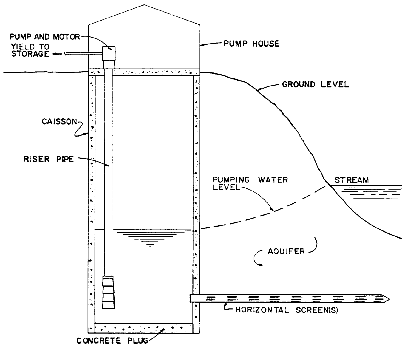
Figure 5-2. Driven well.
