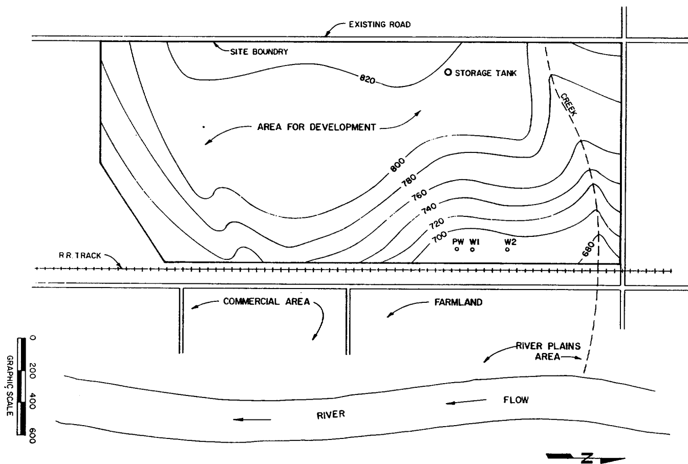
Figure B-1. Plan of proposed site.
