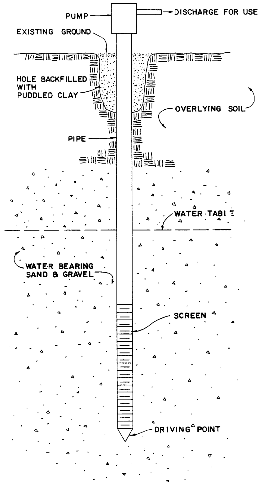
Figure 5-1. Water availability evaluation.
