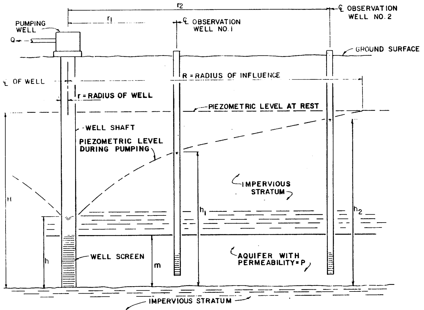
Figure 5-5. Diagram of well in artesian aquifer.
