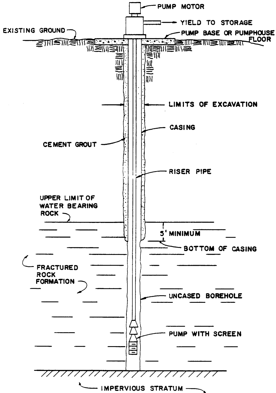
Figure 5-7. Well in rock formation.
