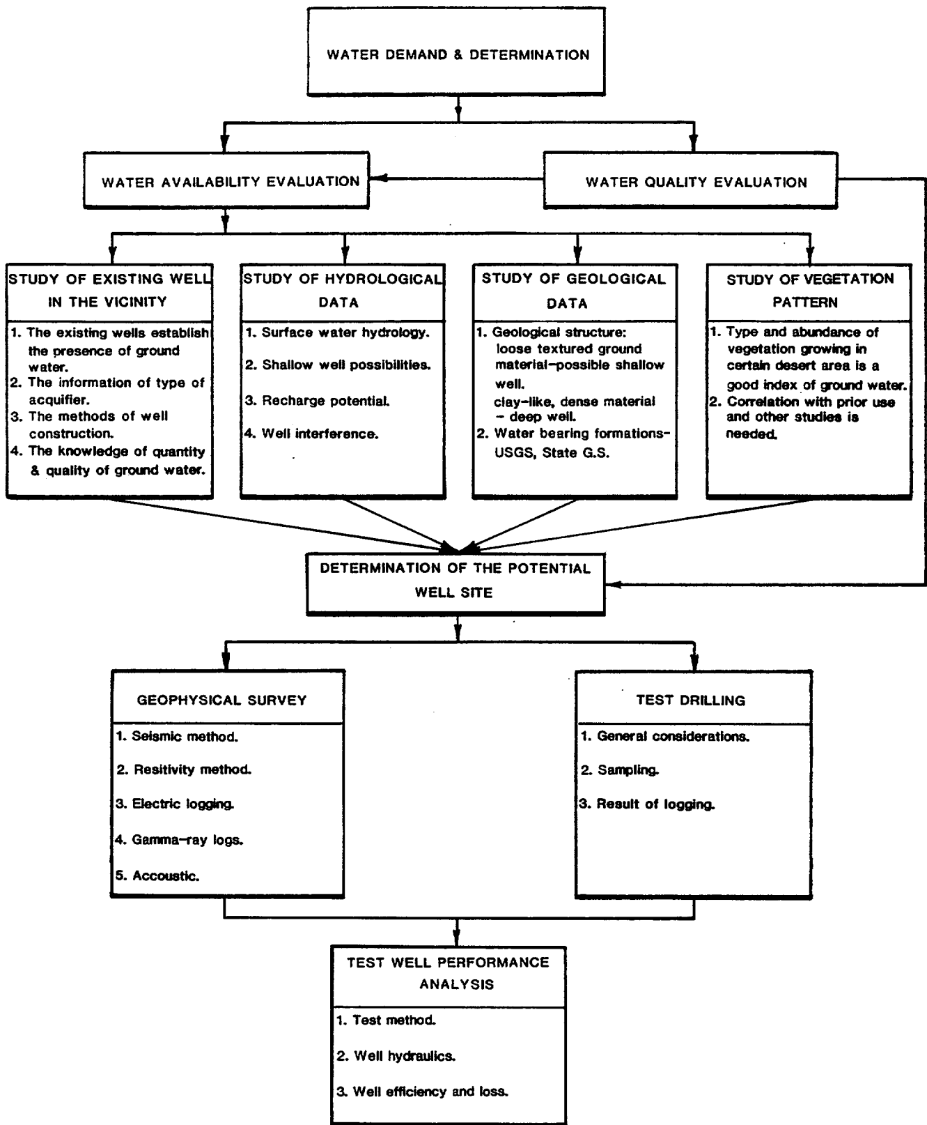
Figure 5-3. Collector well.
