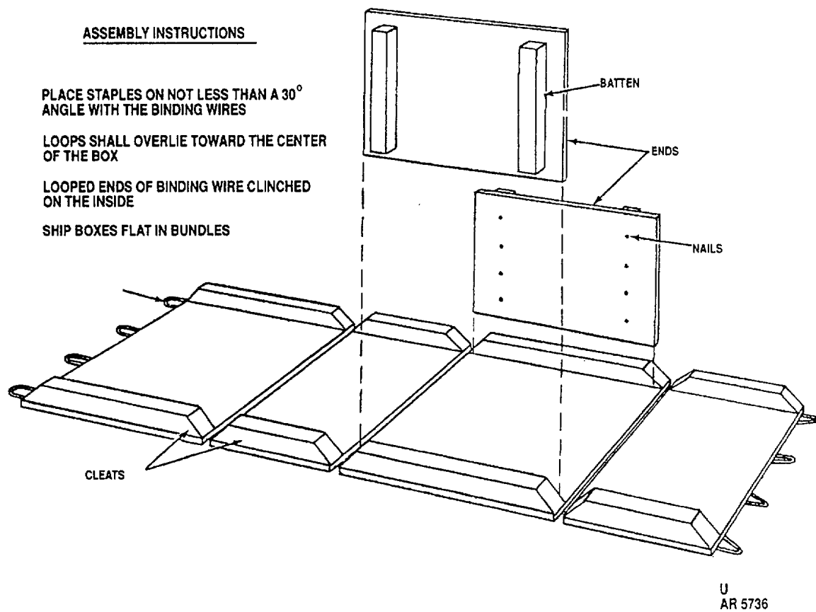
Figure 4-1. Box, wirebound
