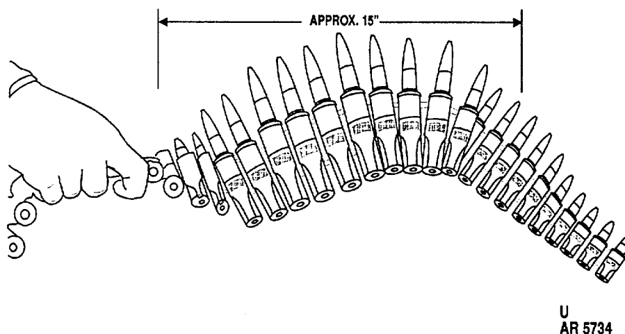
Figure 3-1. Twist inspection.
