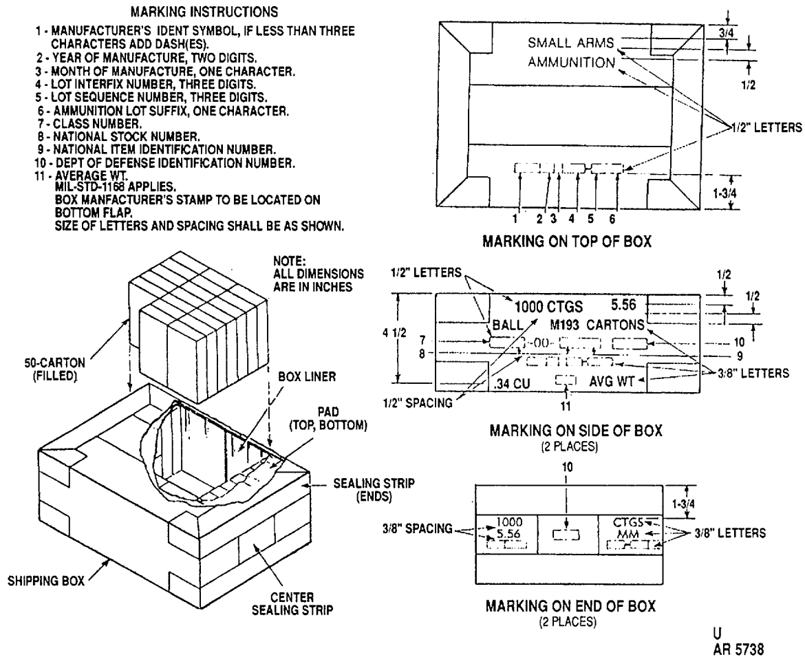
Figure 4-3. Typical packing and marking for 5.56mm ammunition box.
