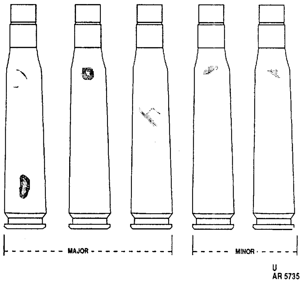
Figure 3-2. Case defects.
