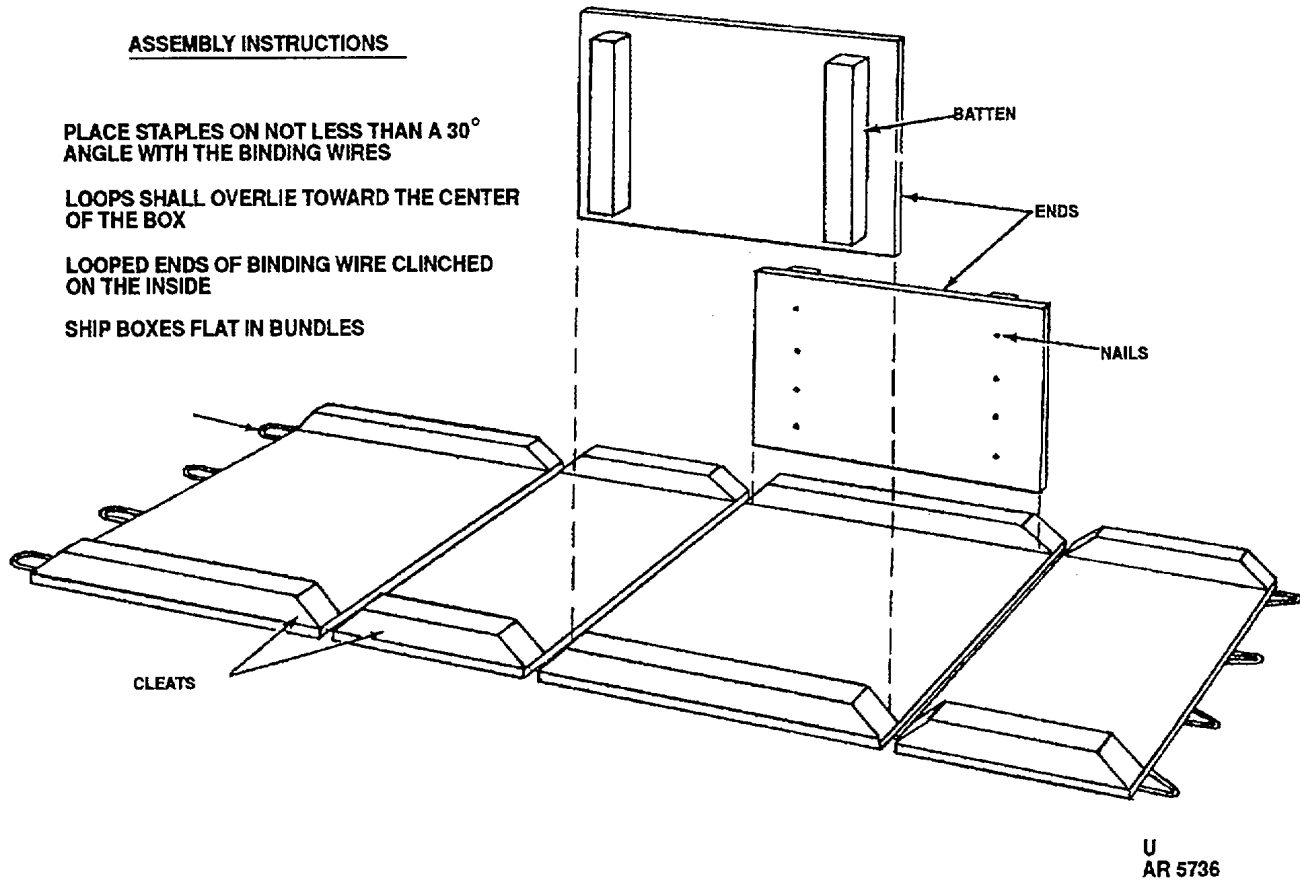
Figure 4-1. Box, wirebound.
