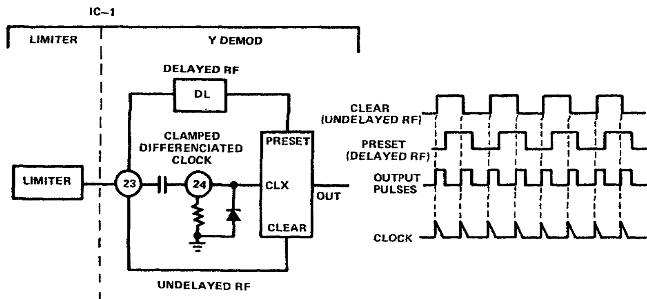
Figure 4-3. Y-FM demodulator
