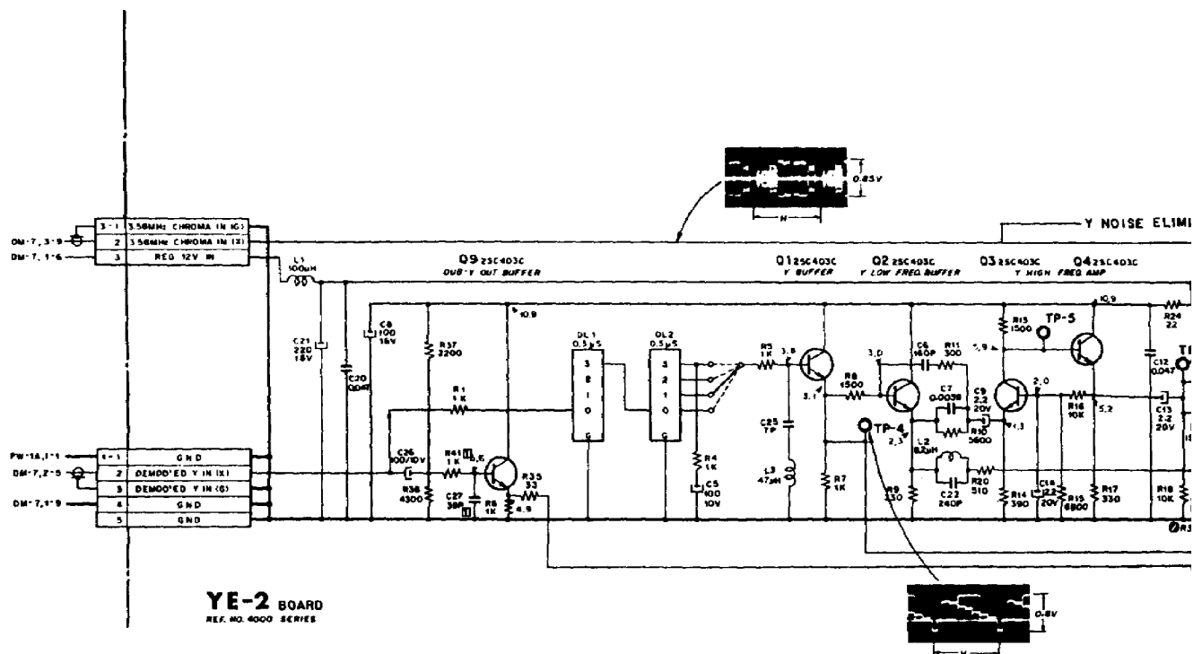
Figure (fo) 4-4. (YE-2) Y noise eliminator, Y/C mixer, and video output amplifier
