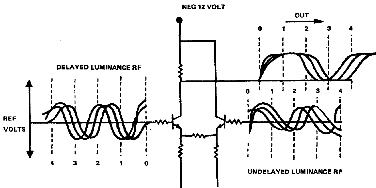
Figure 4-1. Cosine equalizer
