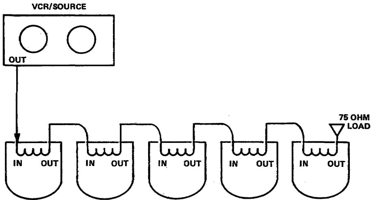
Figure 1-7. Loop-through connection
