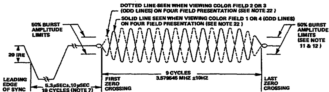
Figure 3-2. Amplitude limits
