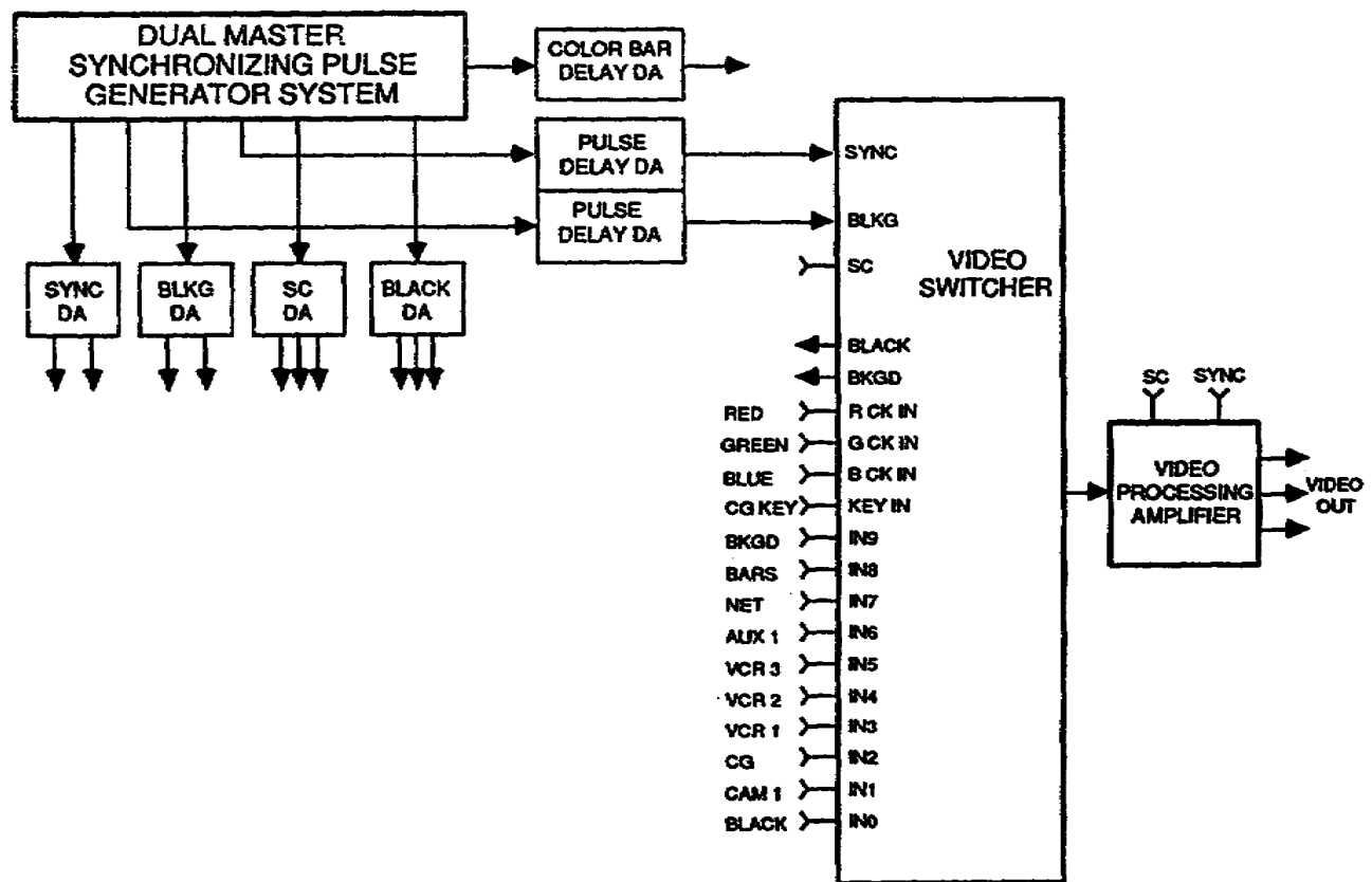
Figure 1-8. Example of rooting switcher system
