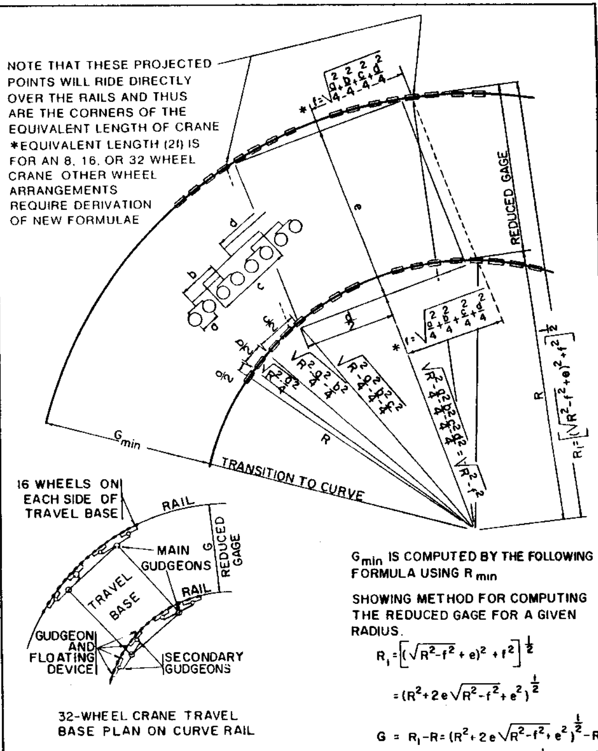
Figure 4 Gage Reduction Diagram (32-Wheel Crane)
