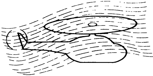
Figure 3.10. Airflow with Translational Lift in Forward Flight.
