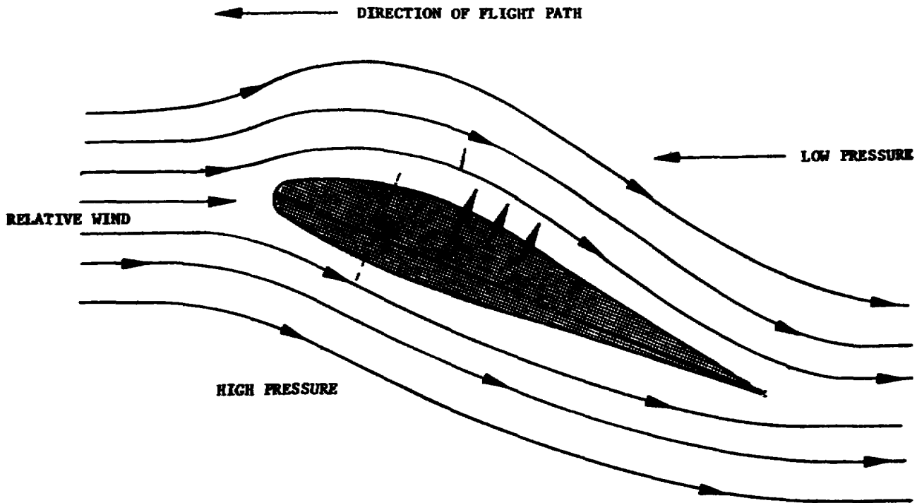
Figure 2.4. Relative Wind.
