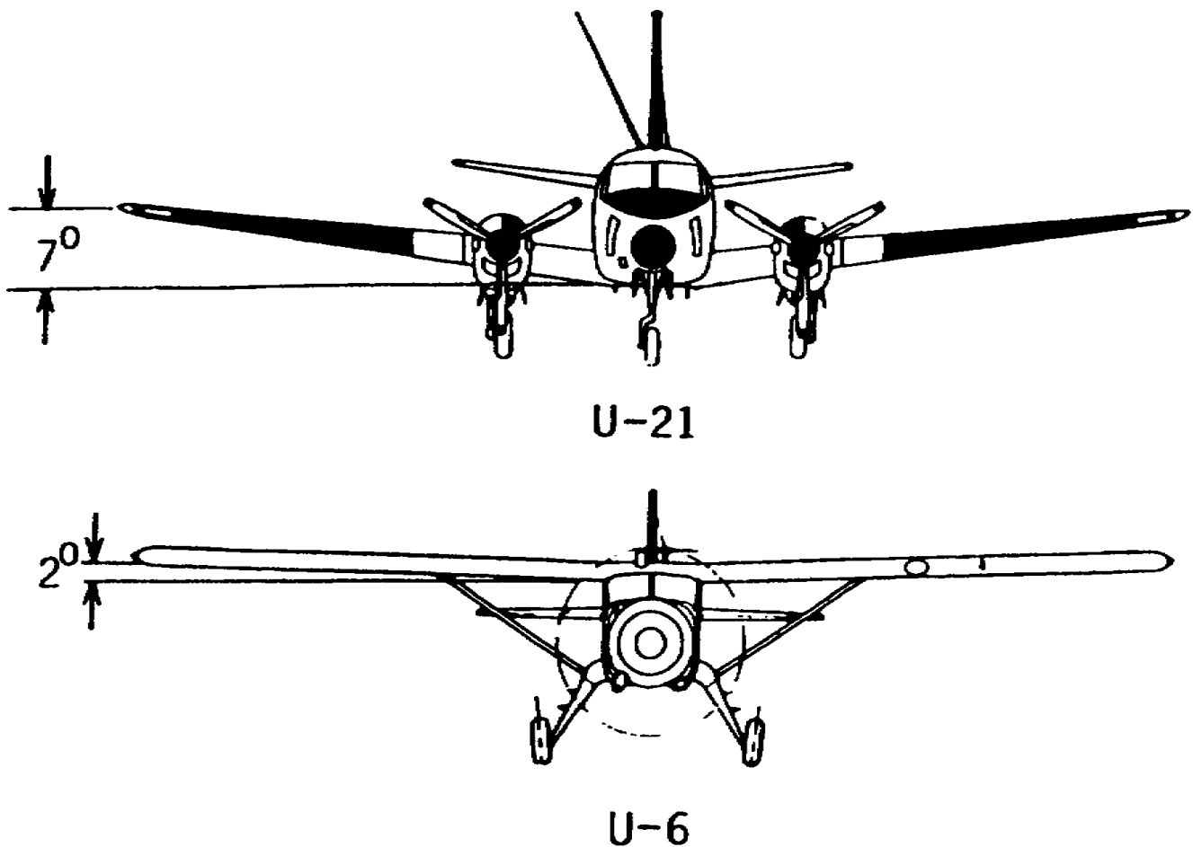
Figure 2.10. Wing Dihedral.
