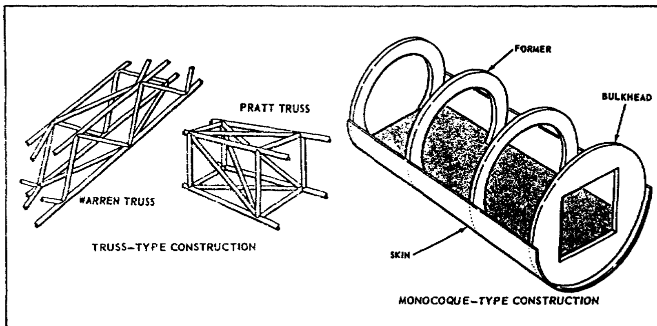
Figure 1-3. Fuselage Construction.
