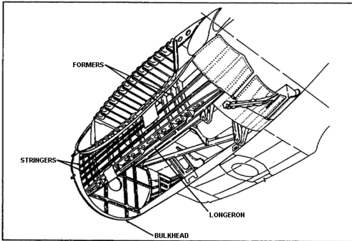
Figure 1-6. Nacelle Construction.
