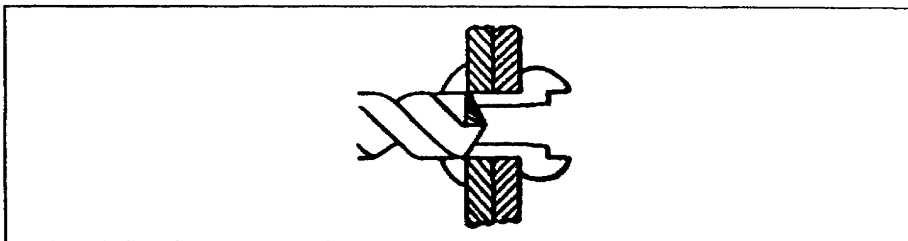
Figure 1-12d. Rivet Removal.
