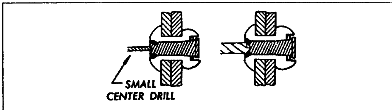
Figure 1-12b. Rivet Removal.
