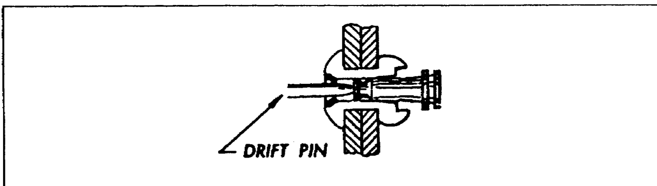
Figure 1-12c. Rivet Removal.
