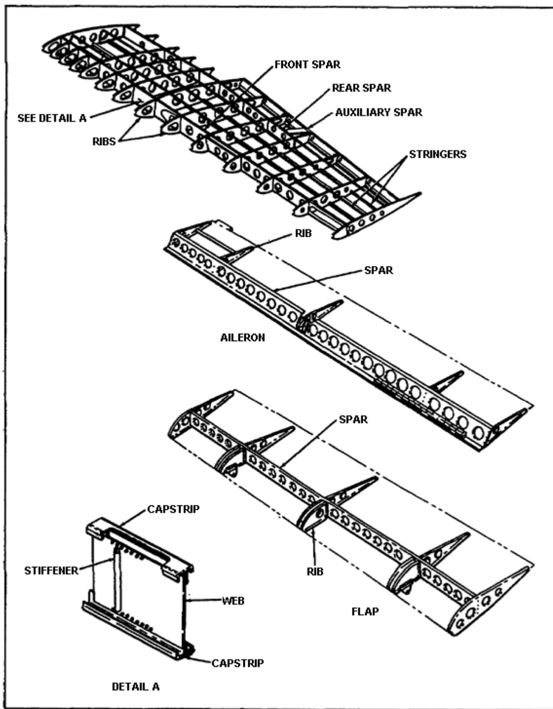
Figure 1-7. Wing Construction.
