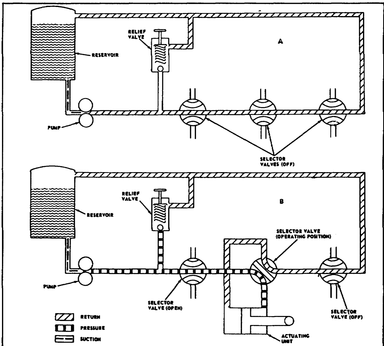
Figure 2-7. Basic Open-Center Hydraulic System.
