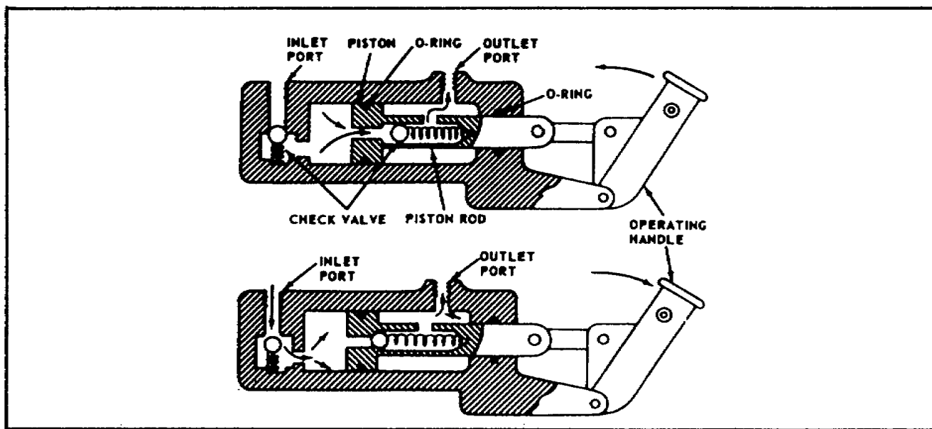
Figure 1-4. Double-Action Hand Pump.
