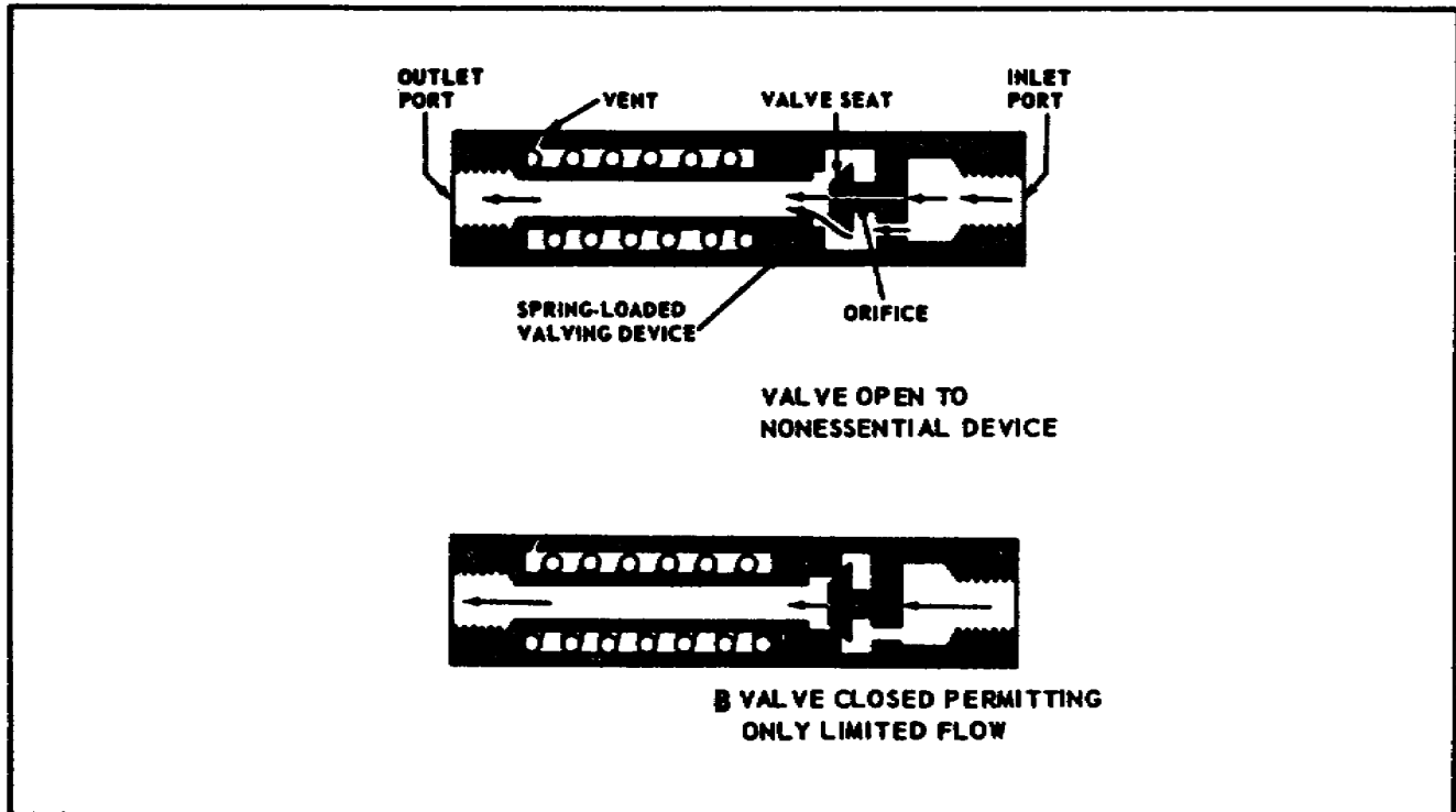
Figure 2-15. Typical Priority Valve.
