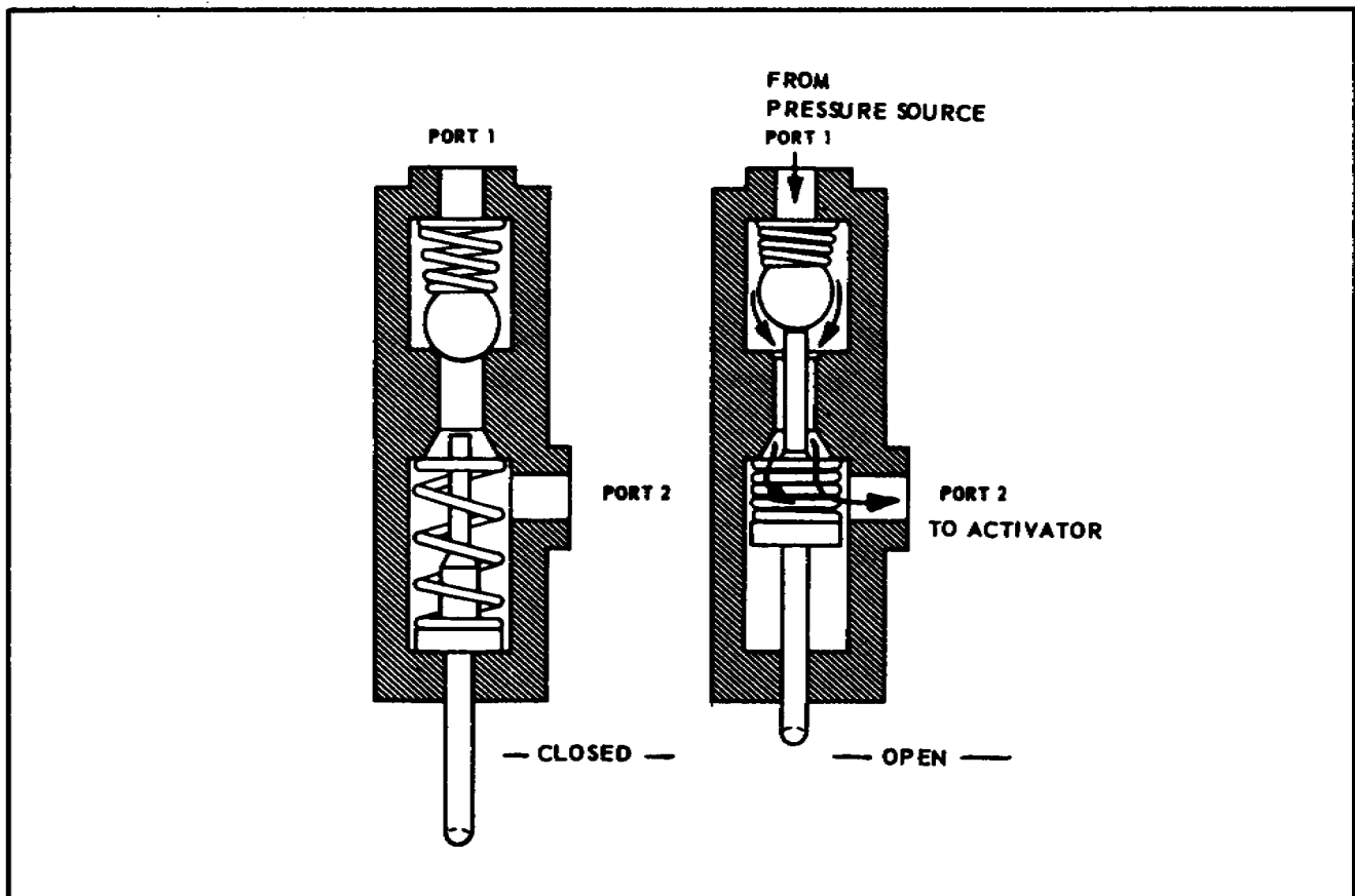
Figure 2-14. Mechanically Actuated Sequence Valve.
