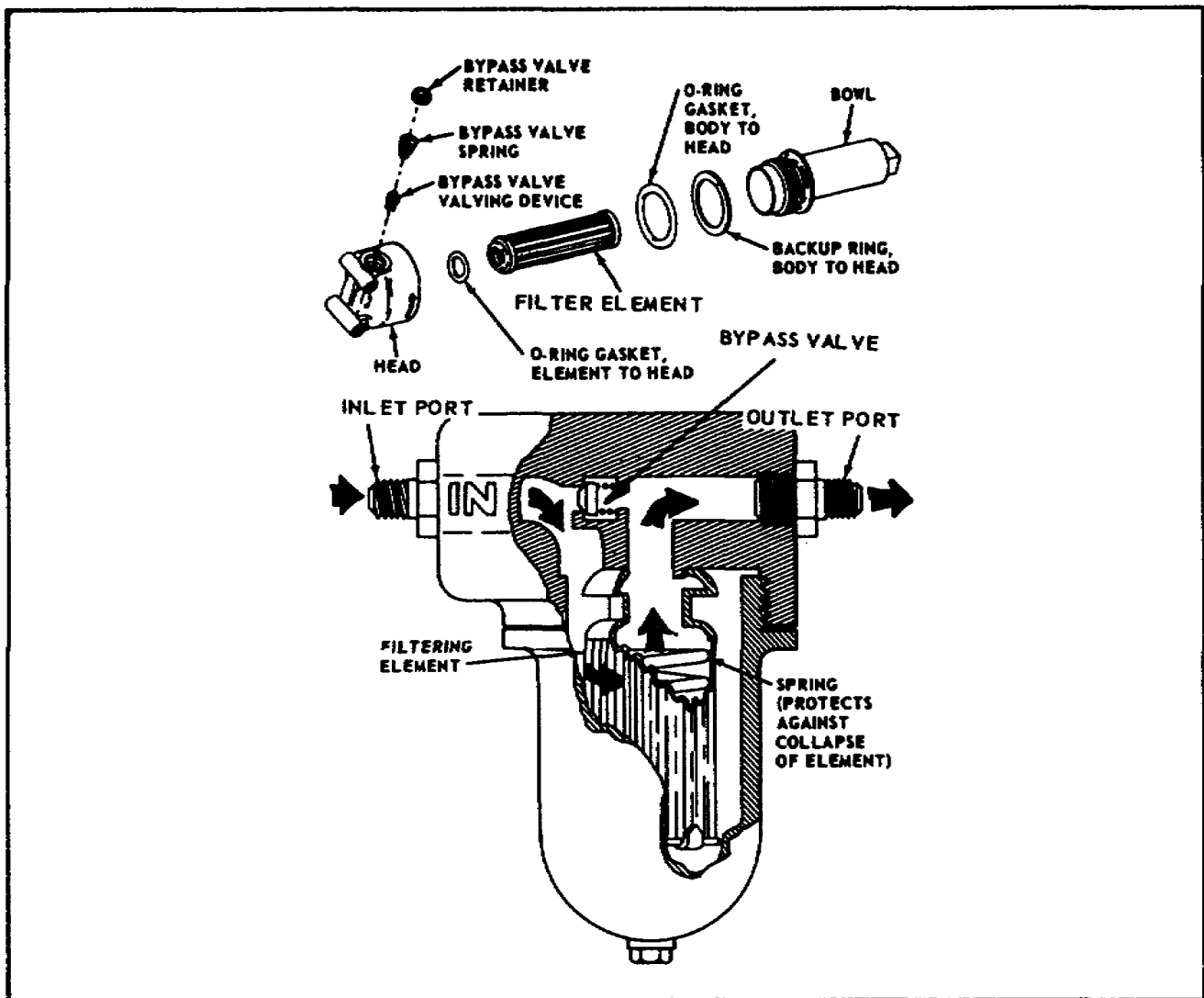
Figure 1-3. Typical Line Filter Assembly.
