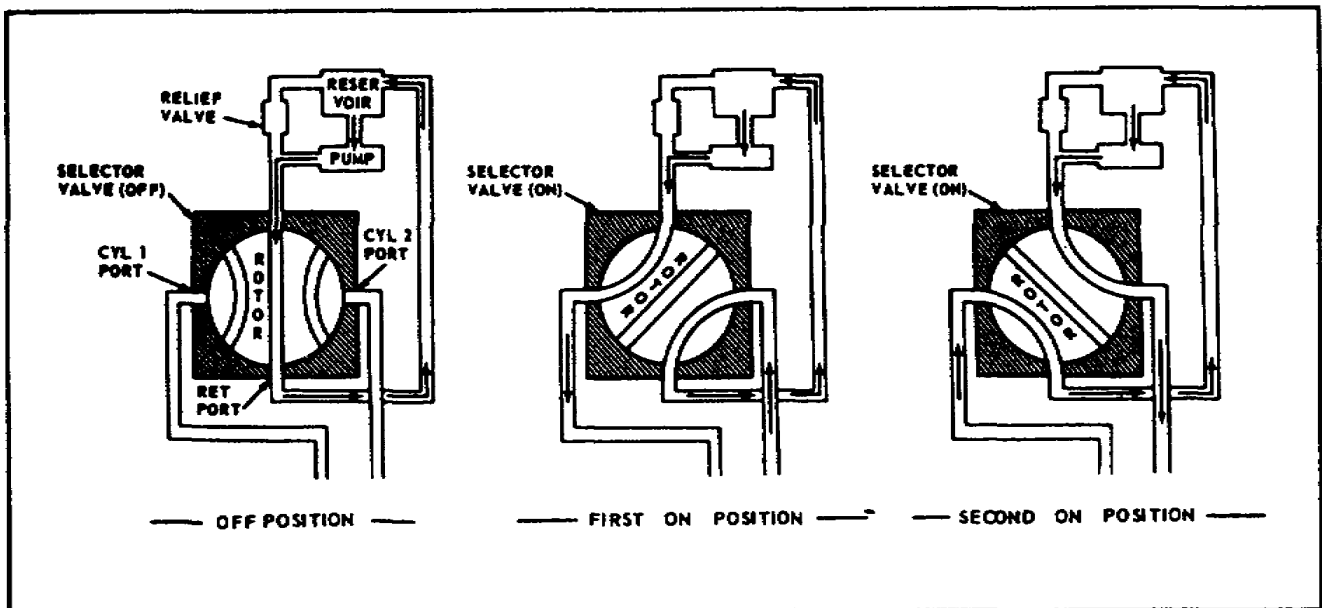
Figure 2-5. Typical Open-Center Rotor Selector Valve.
