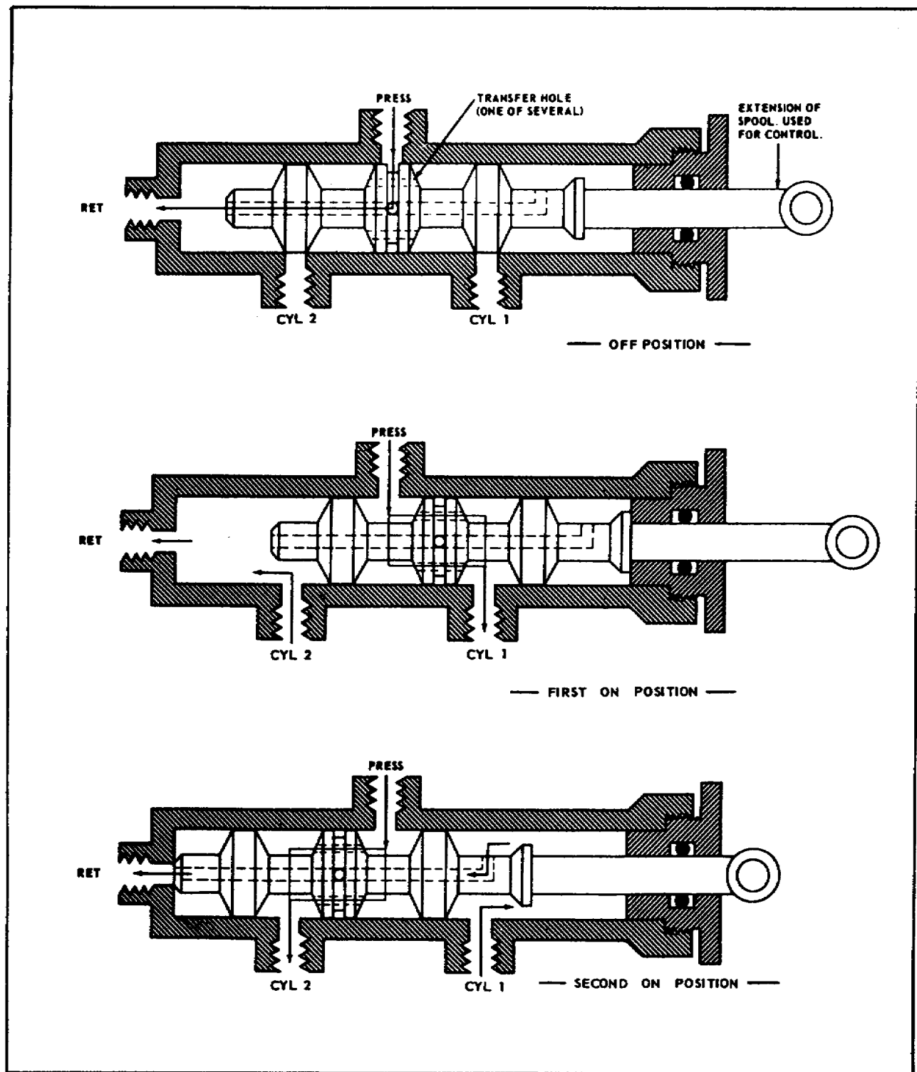
Figure 2-6. Typical Open-Center Spool Selector Valve.
