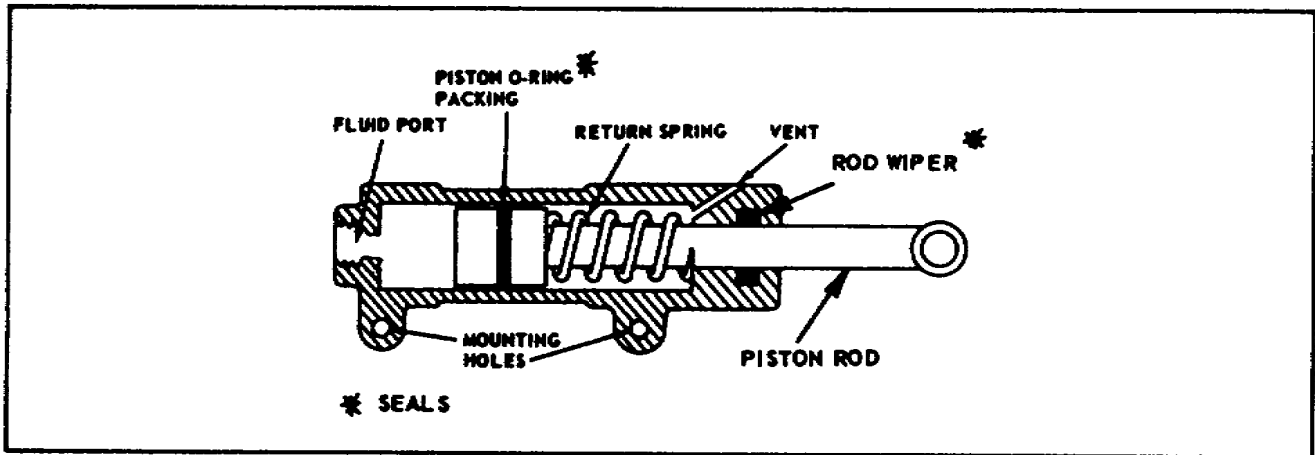
Figure 2-1. Single-Action Actuating Cylinder.
