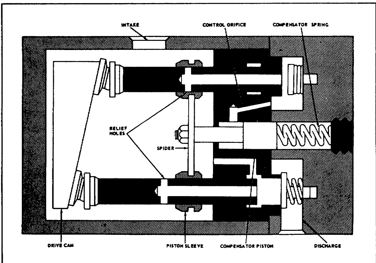
Figure 1-8. Variable-Delivery Demand-Principle Cam Pump.
