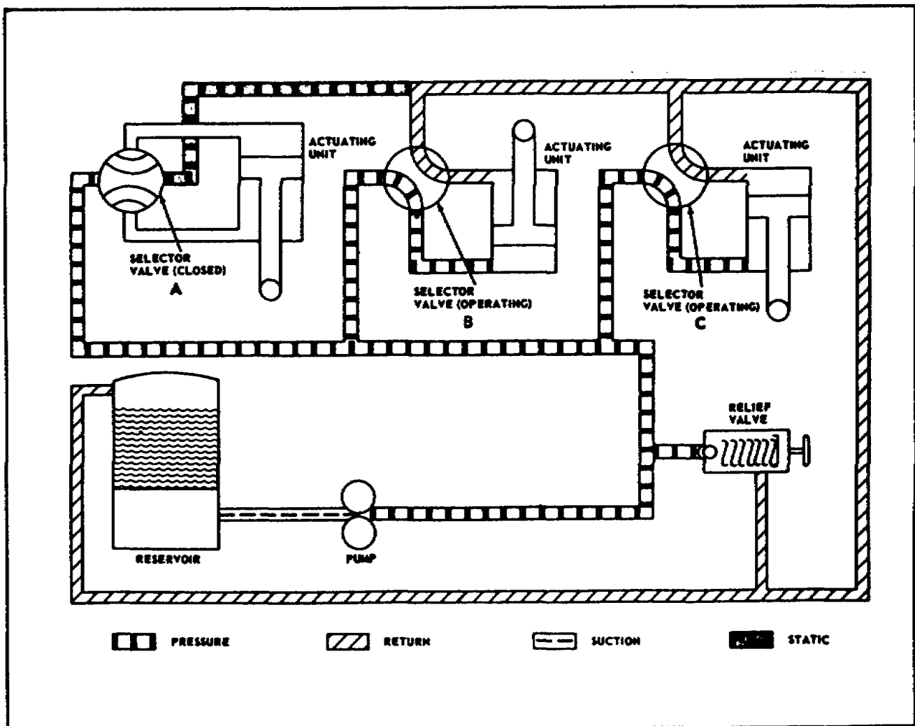
Figure 2-8. Basic Closed-Center System.
