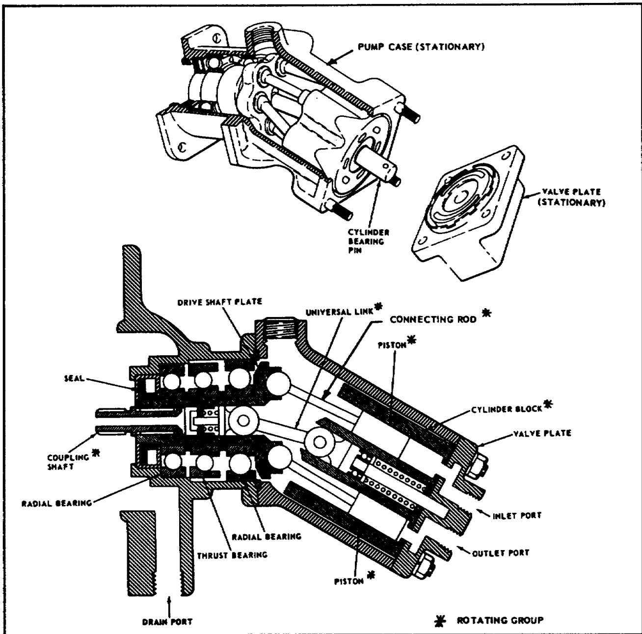
Figure 1-6. Typical Angular Piston Pump.
