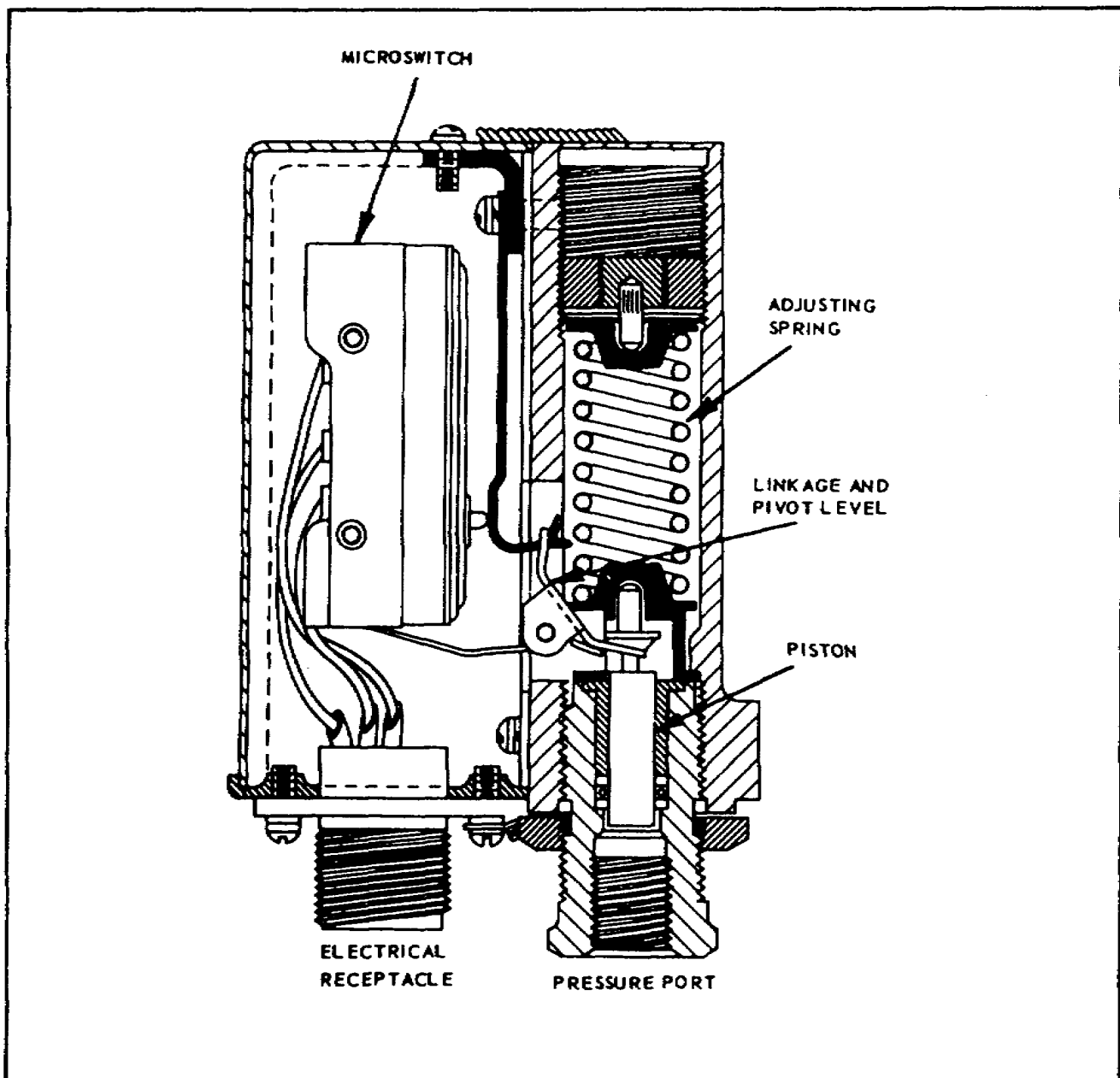
Figure 3-3. Piston Pressure Switch.
