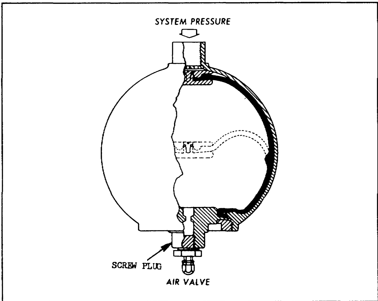
Figure 1-11. Bladder Accumulator.
