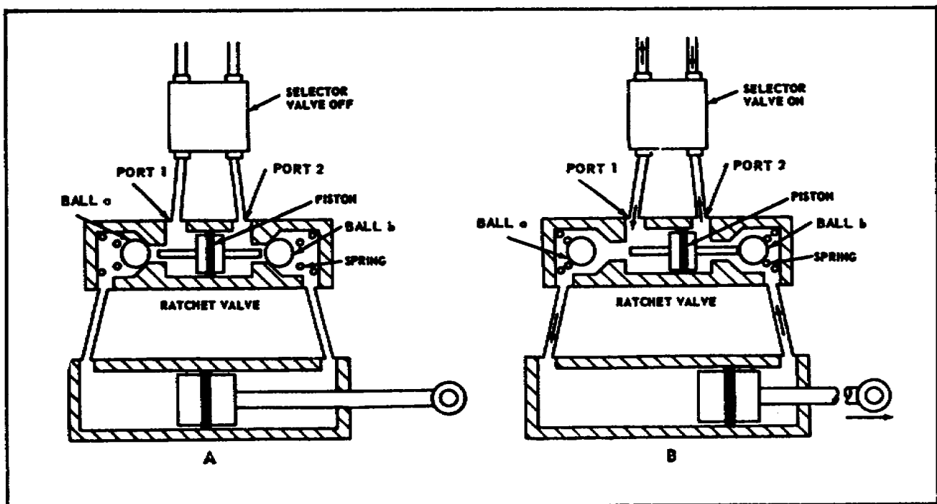
Figure 2-11. Typical Application of Ratchet Valve.
