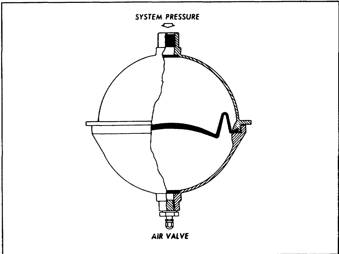
Figure 1-10. Diaphragm Accumulator.
