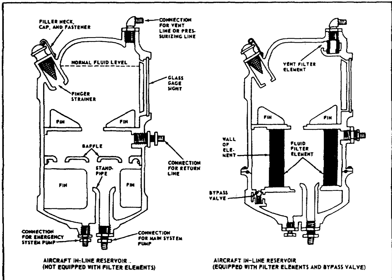
Figure 1-1. Typical Hydraulic Reservoirs.
