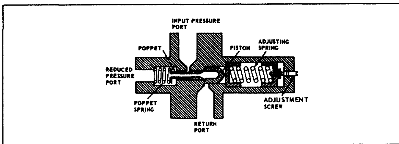
Figure 3-2. Pressure Reducer.
