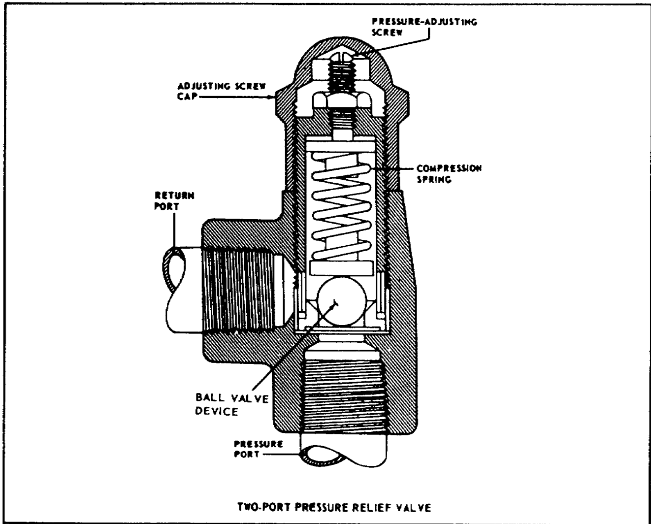
Figure 3-1. Pressure Relief Valve.
