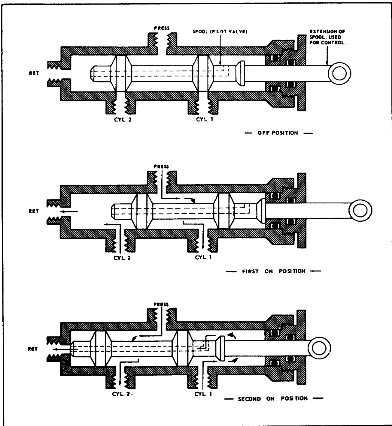
Figure 2-4. Typical Spool Closed-Center Selector Valve.
