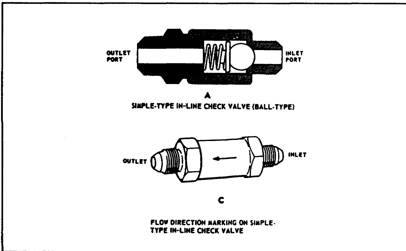
Figure 2-12. Simple In-Line Check Valve.
