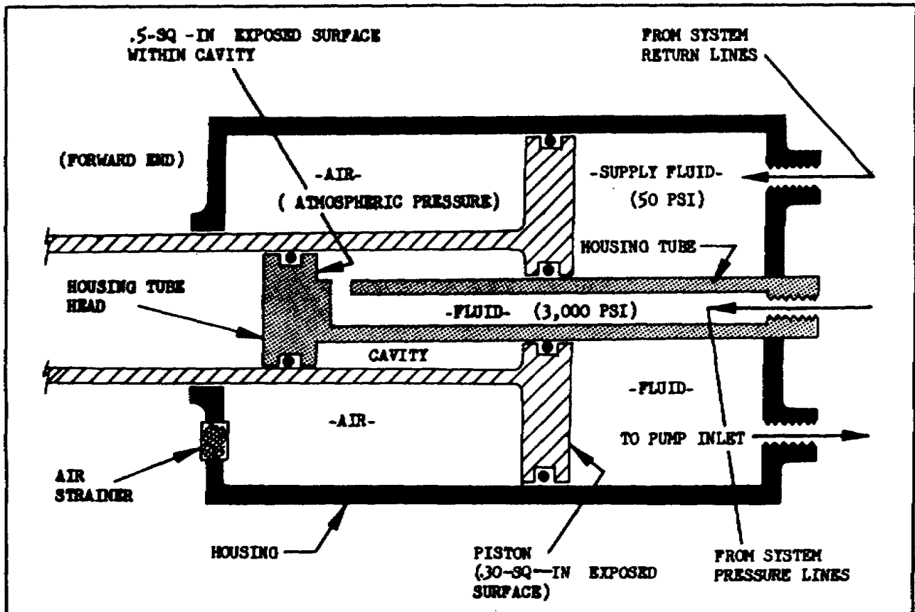
Figure 1-2. Hydraulic Reservoir Pressurized With Hydraulic Fluid.
