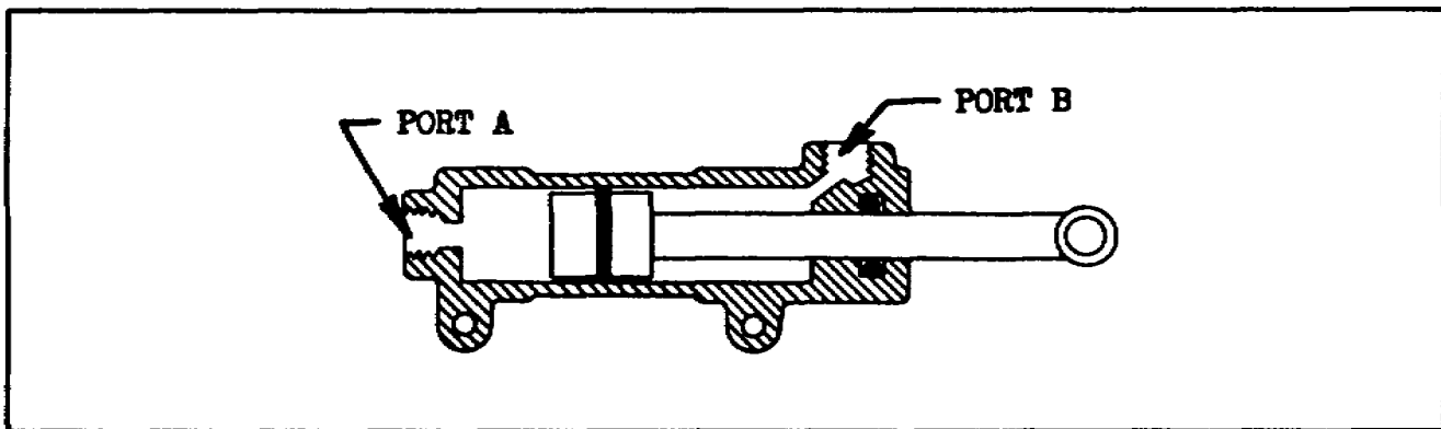
Figure 2-2. Double-Action Actuating Cylinder.
