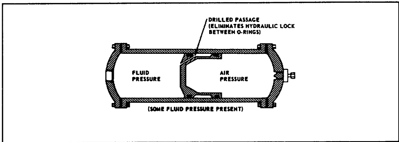
Figure 1-12. Piston Accumulator.
