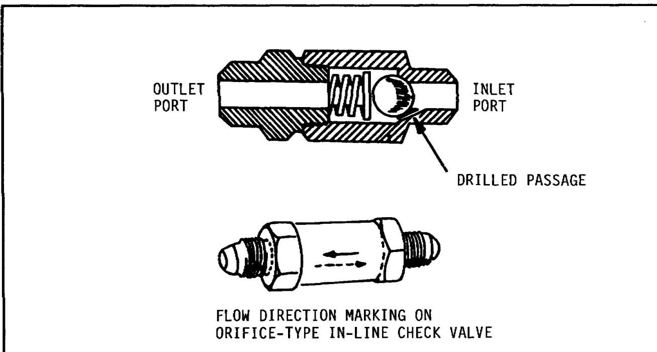
Figure 2-13. Orifice In-Line Check Valve.
