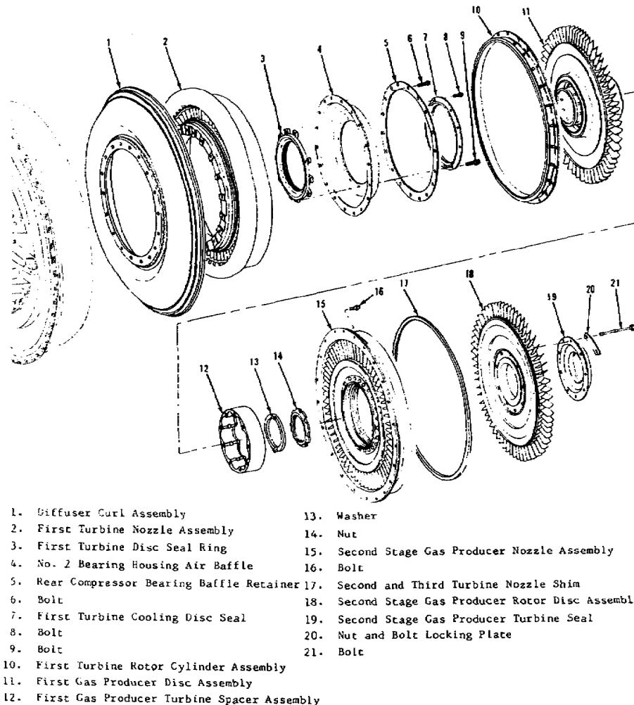
Figure 5.10. Gas Producer Assembly.
