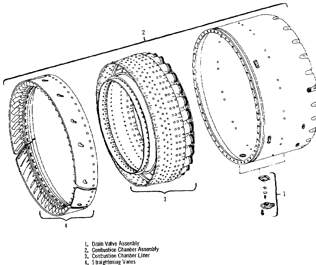
Figure 5.9. Combustion Chamber Housing Assembly.
