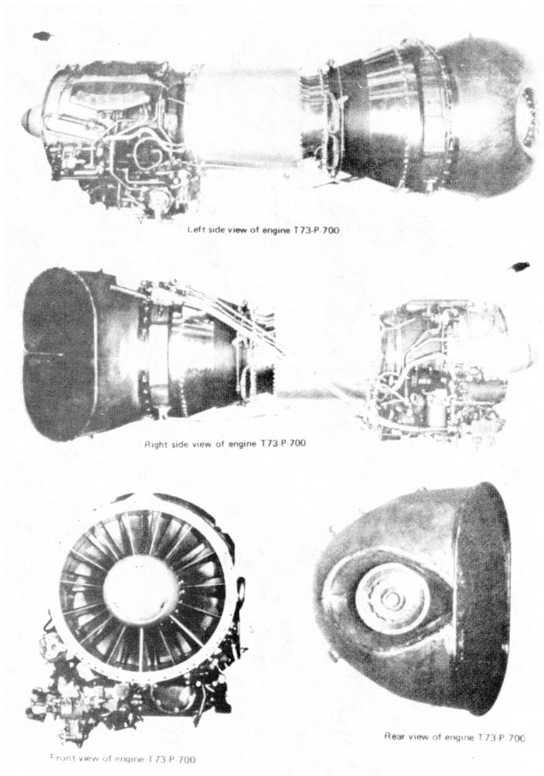
Figure 8-1. T73-P-700 Gas Turbine Engine.
