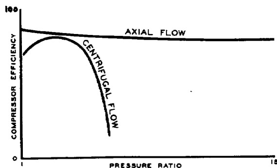
Figure 1.14. Compressor Efficiencies and Pressure Ratios .
