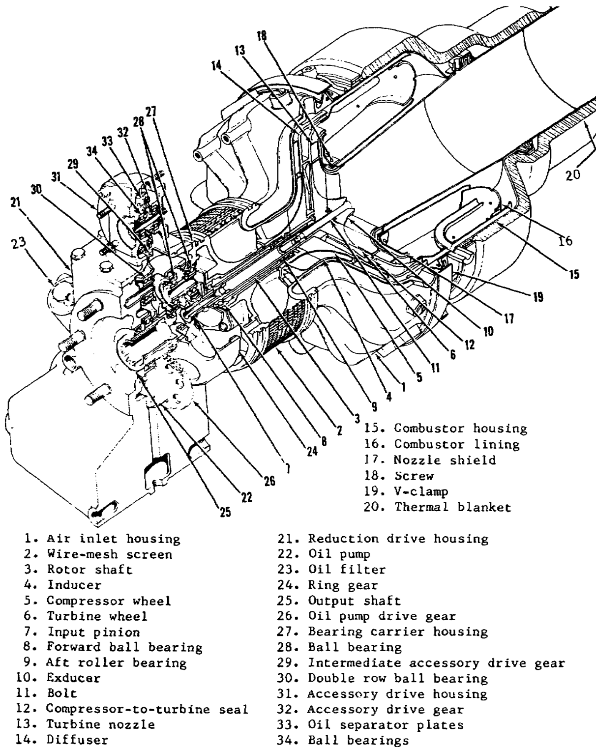
Figure 6.3. T62T-2A Cutaway Engine Assembly.
