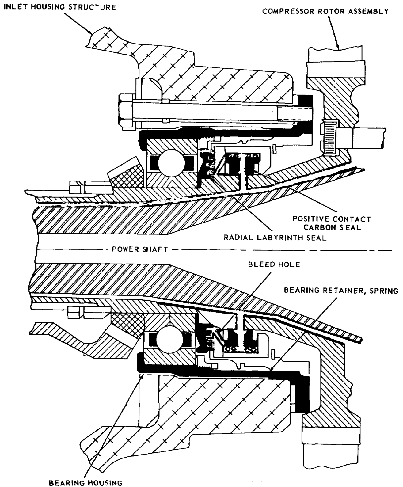
Figure 4.6. No. 1 Bearing and Seal Area.
