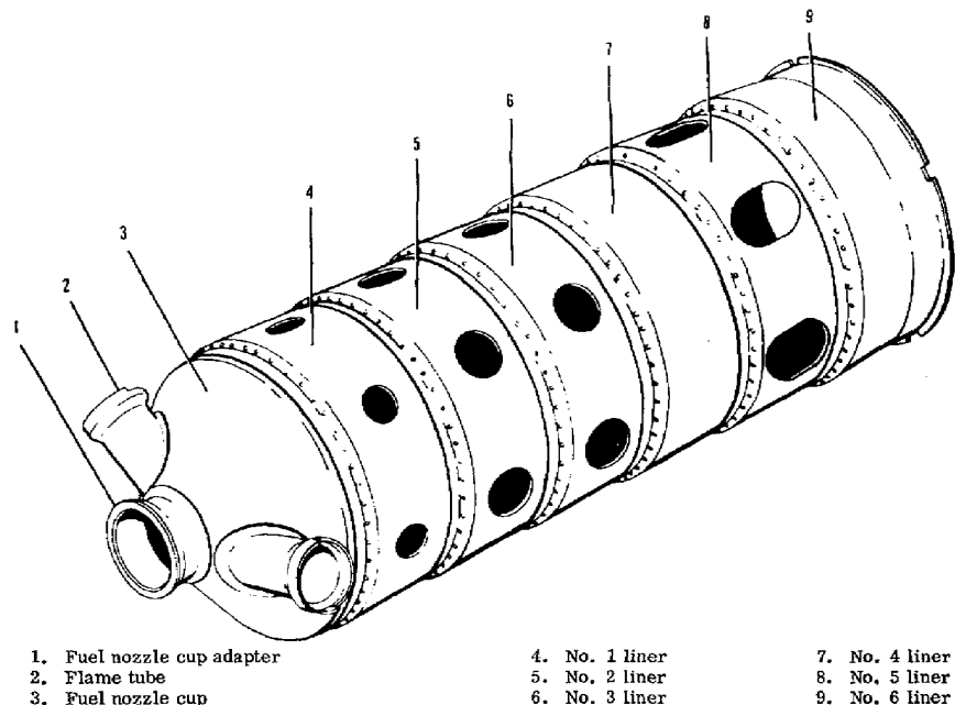
Figure 8.7. Combustion Chamber.
