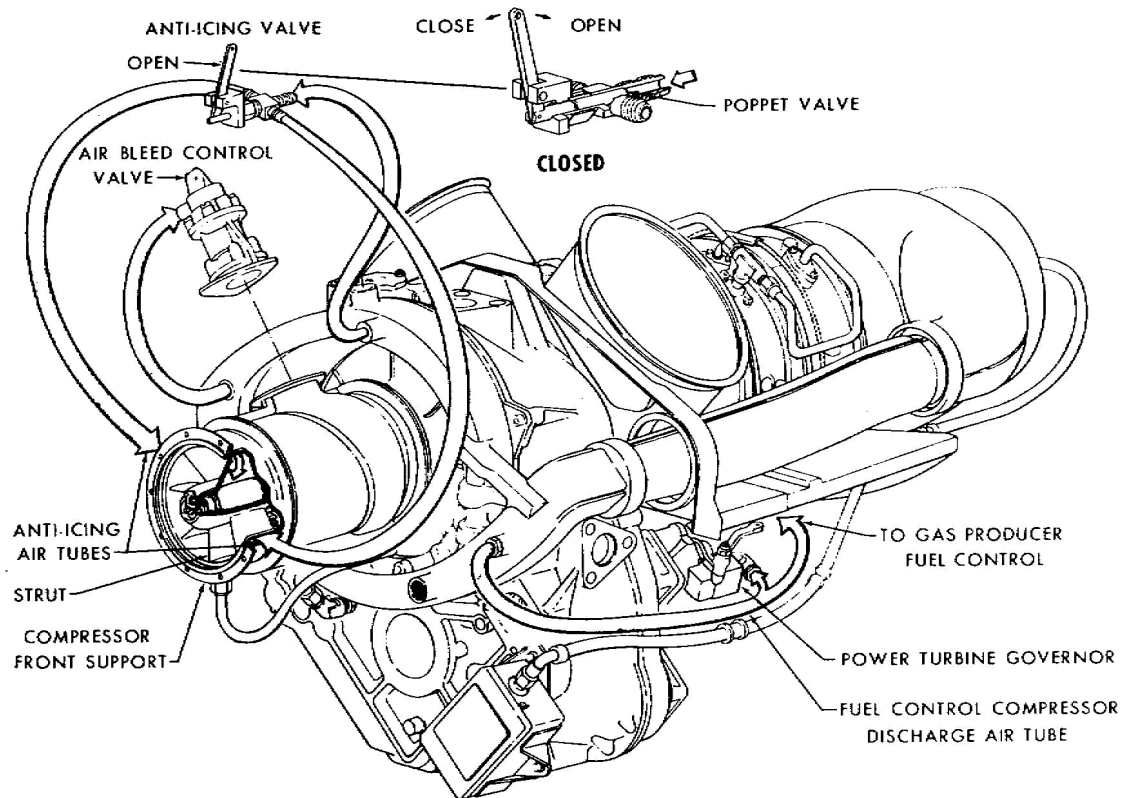
Figure 7.15. Air Bleed and Anti-Icing System.
