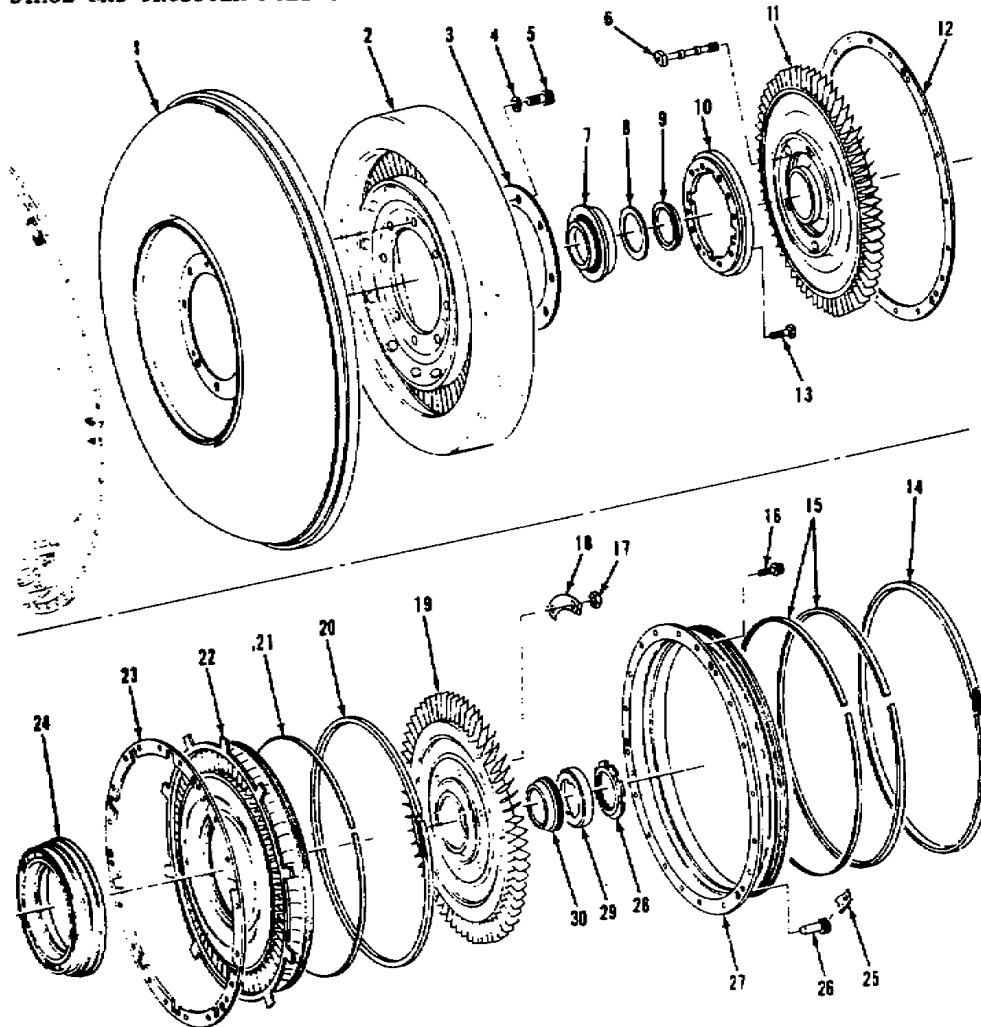
Figure 4.16. Gas Producer Assembly, N 1 .
