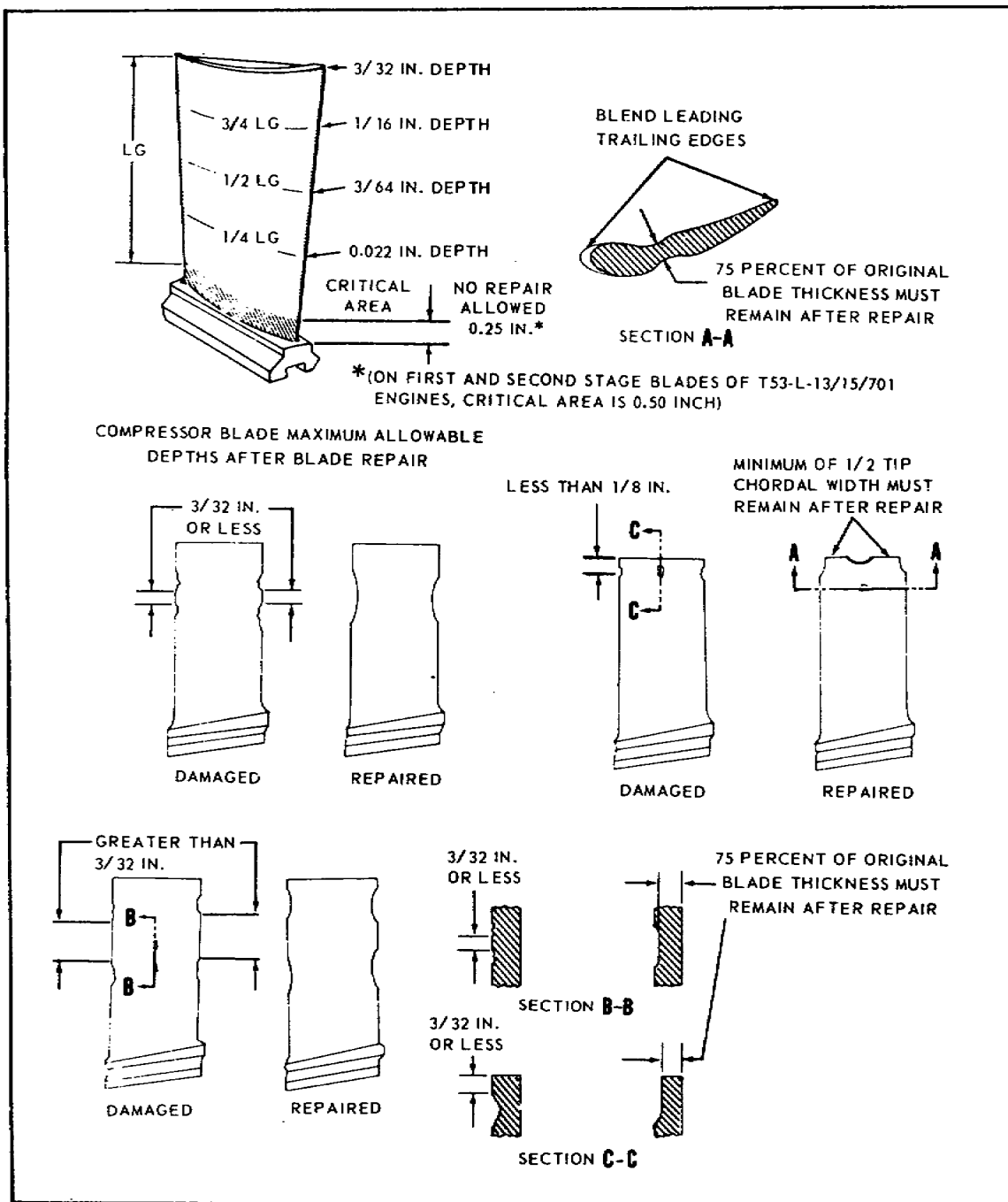
Figure 3.9. Compressor Rotor Blade Damage Before and After Repair.
