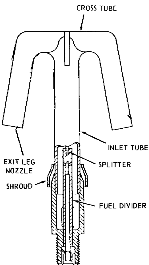
Figure 2.8. Vaporizing Tube.
