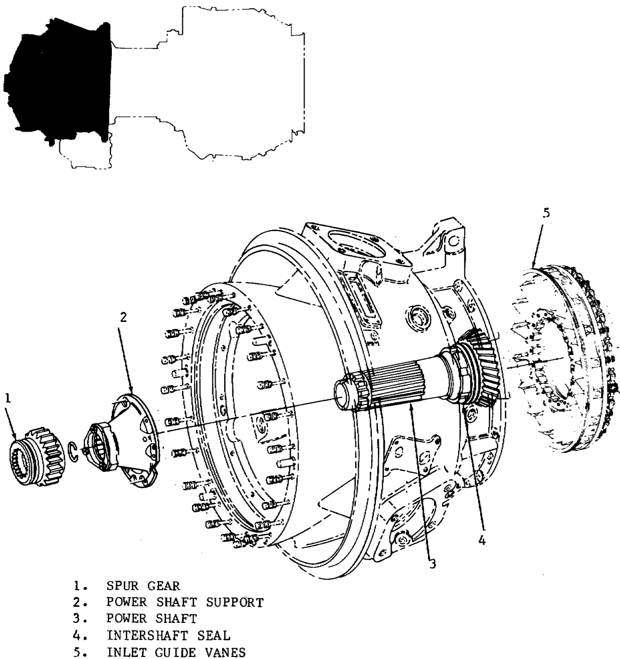
Figure 4.5. Inlet Housing.
