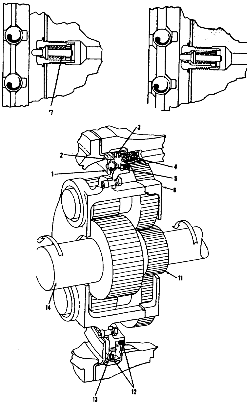
Figure 4.32. Torquemeter Diagram.
