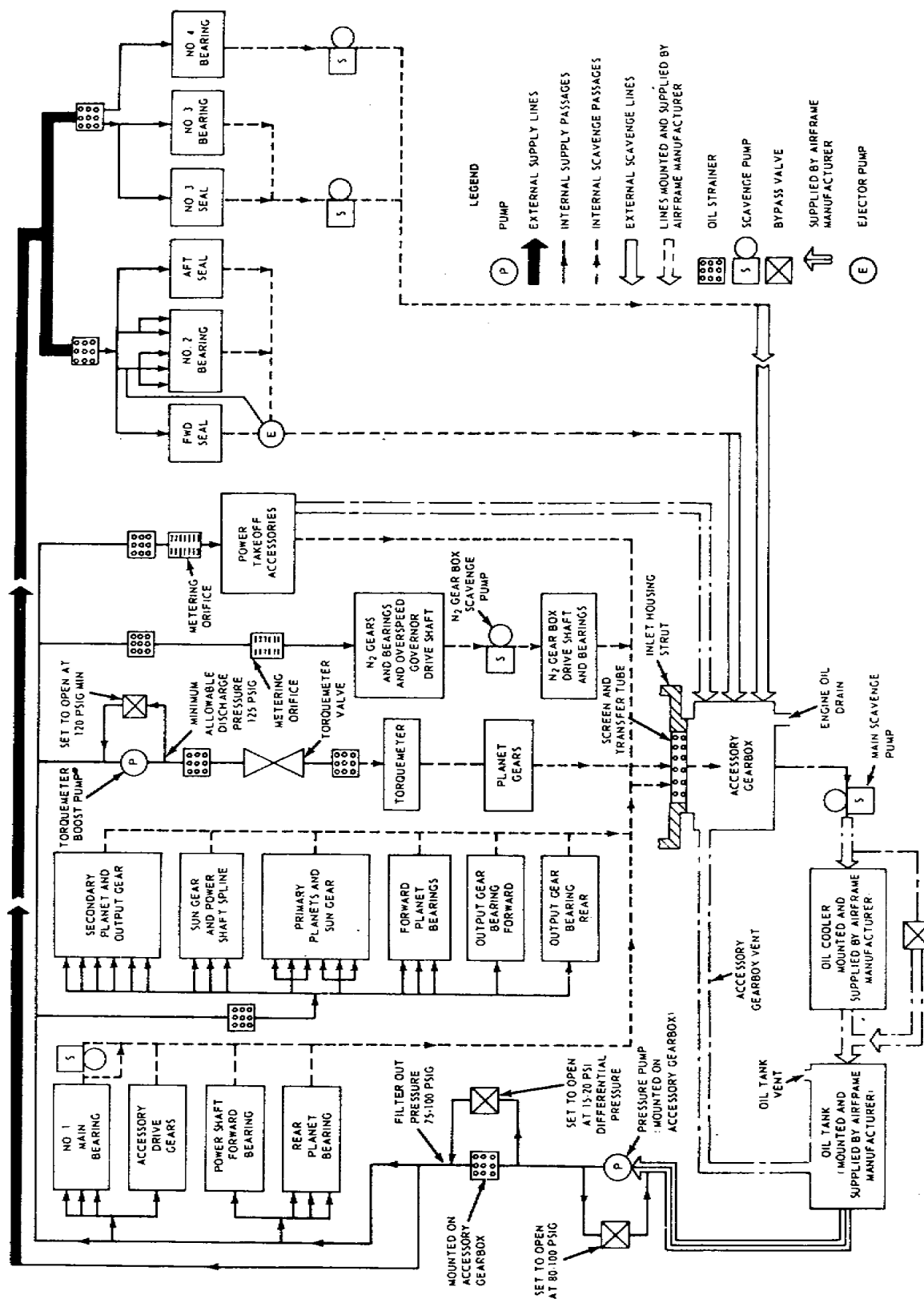
Figure 4.30. Internal Lubrication (T53-L-13).
