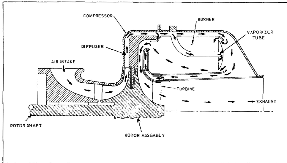
Figure 6.5. Airflow Diagram.
