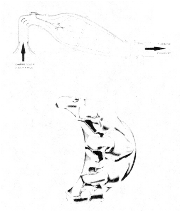
Figure 1.19. Can-type Combustion Chamber (Cutaway).
