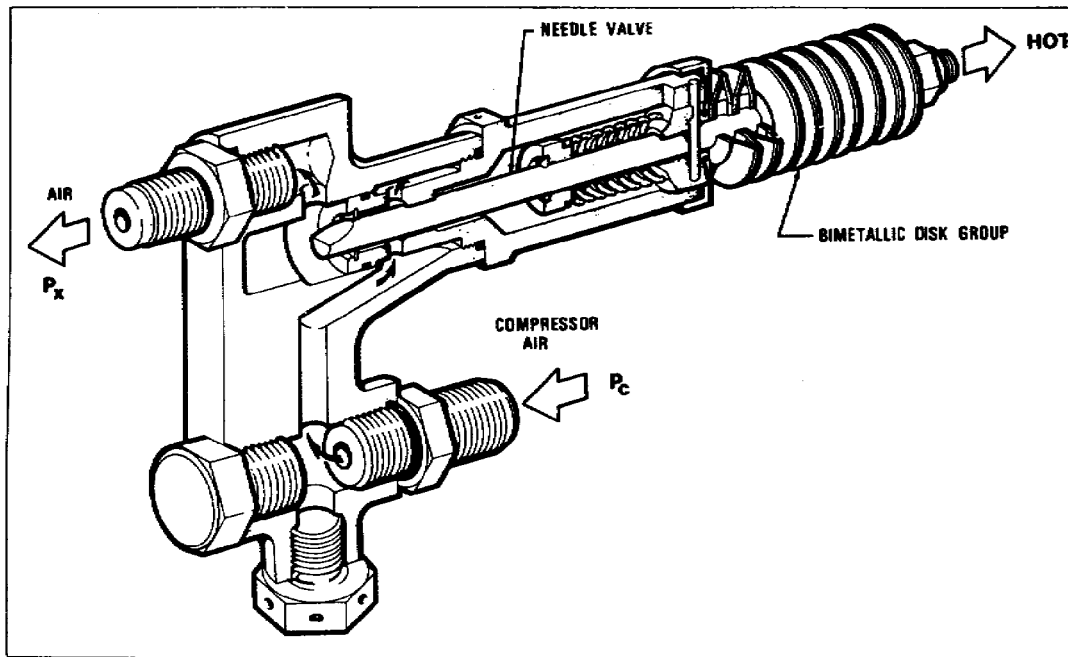
Figure 9.15. Temperature Compensator, -700.
