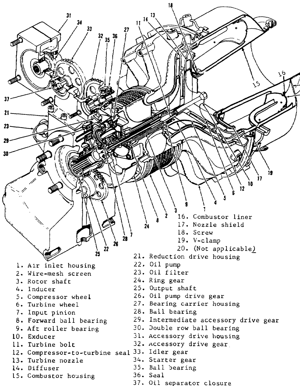
Figure 6.4. T62T-16A Cutaway Engine Assembly.
