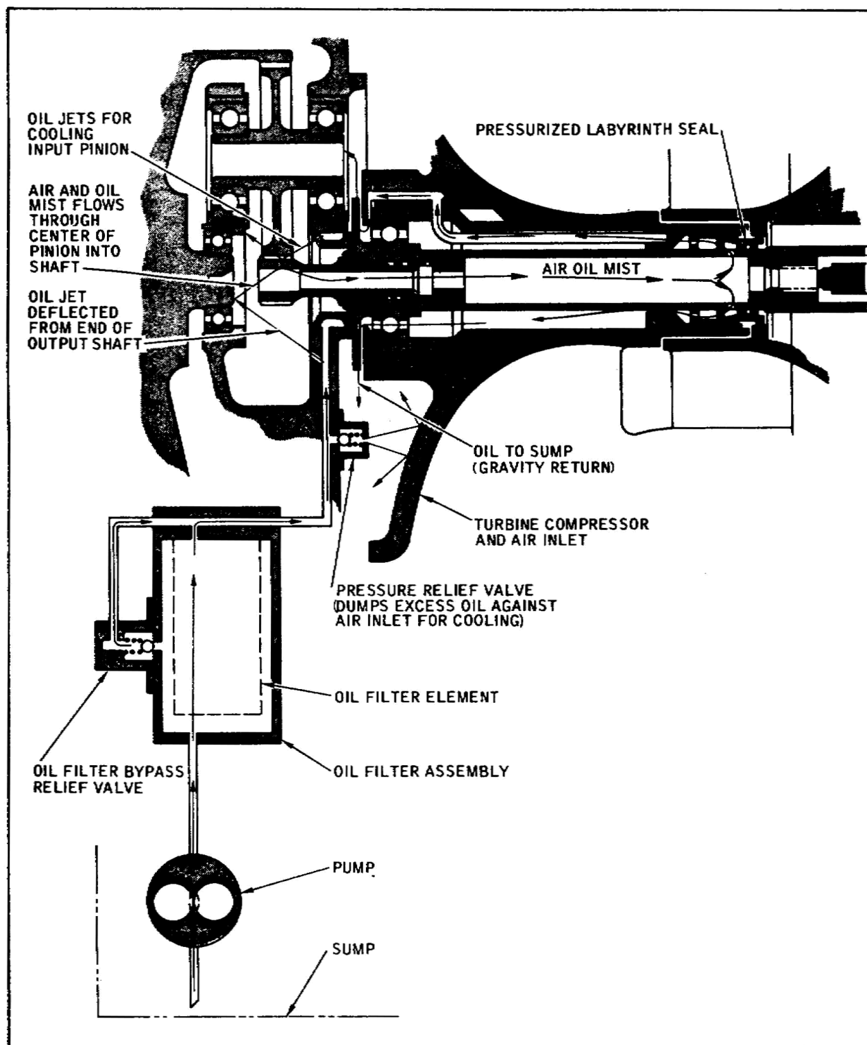
Figure 6.7. Lubrication System Schematic.
