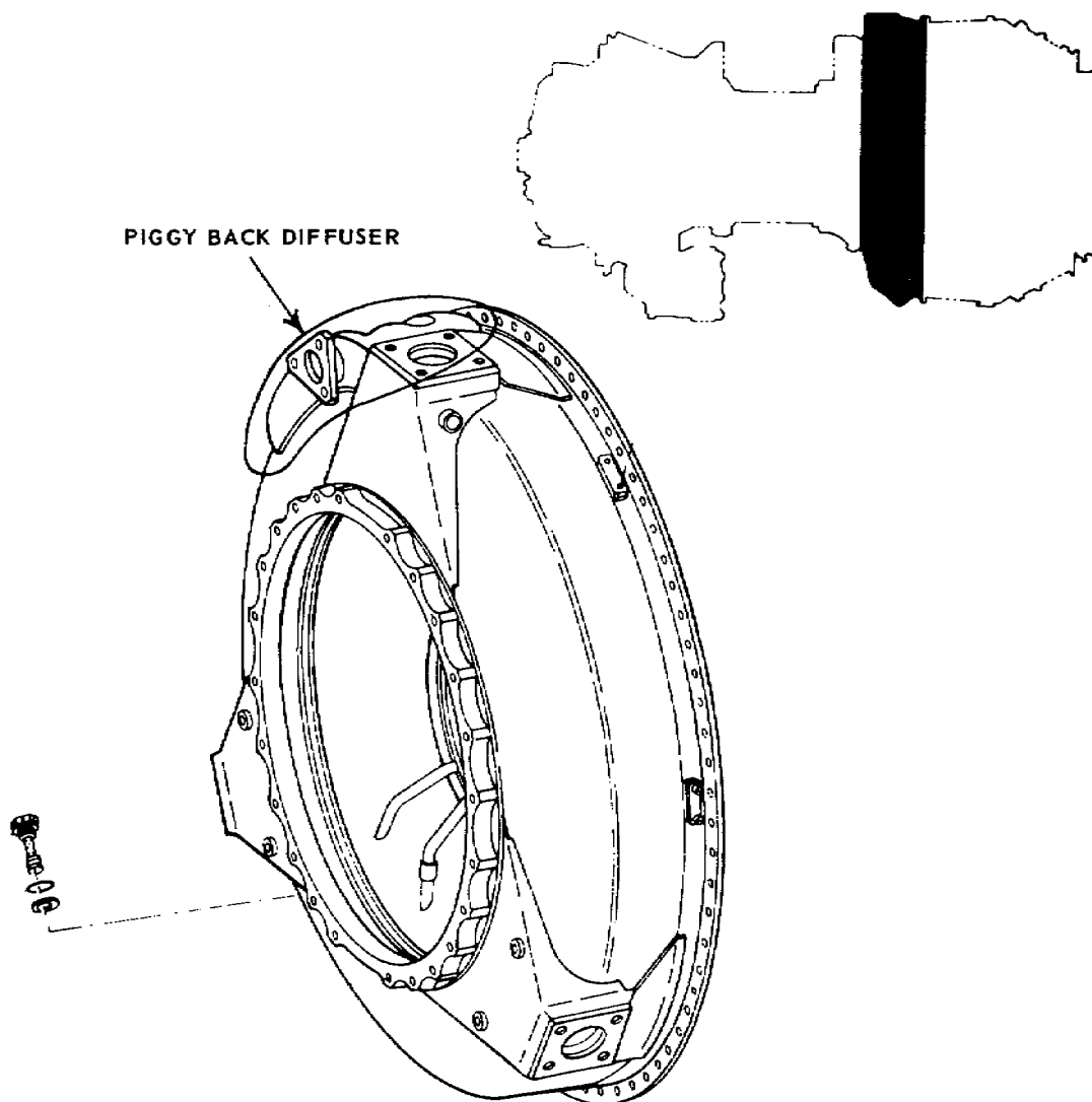
Figure 4.14. Diffuser Housing.
