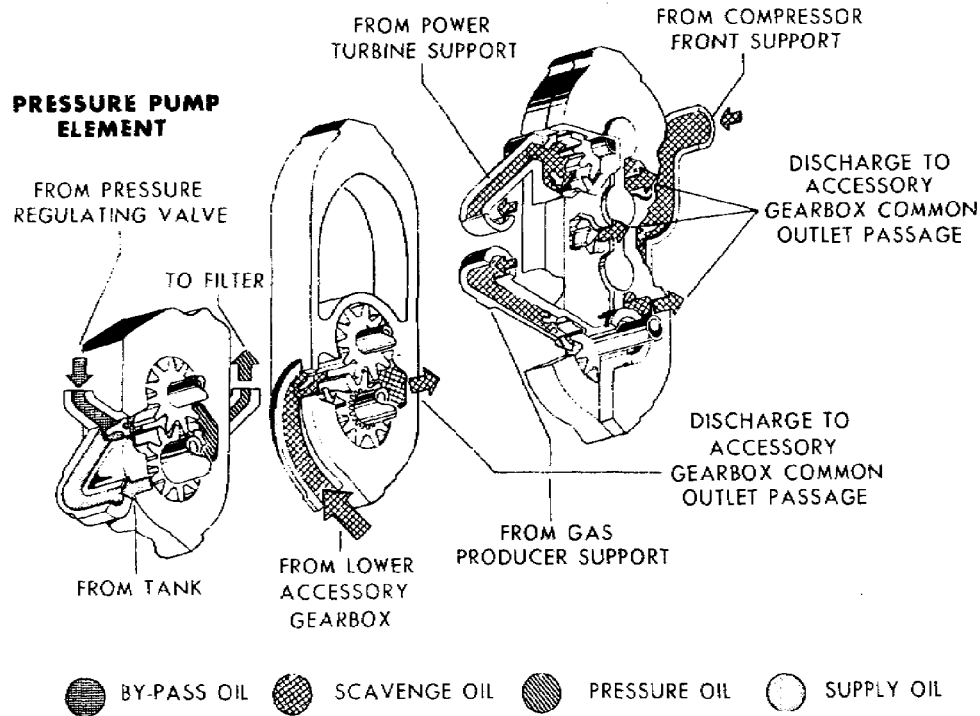
Figure 7.10. Oil Pump.
