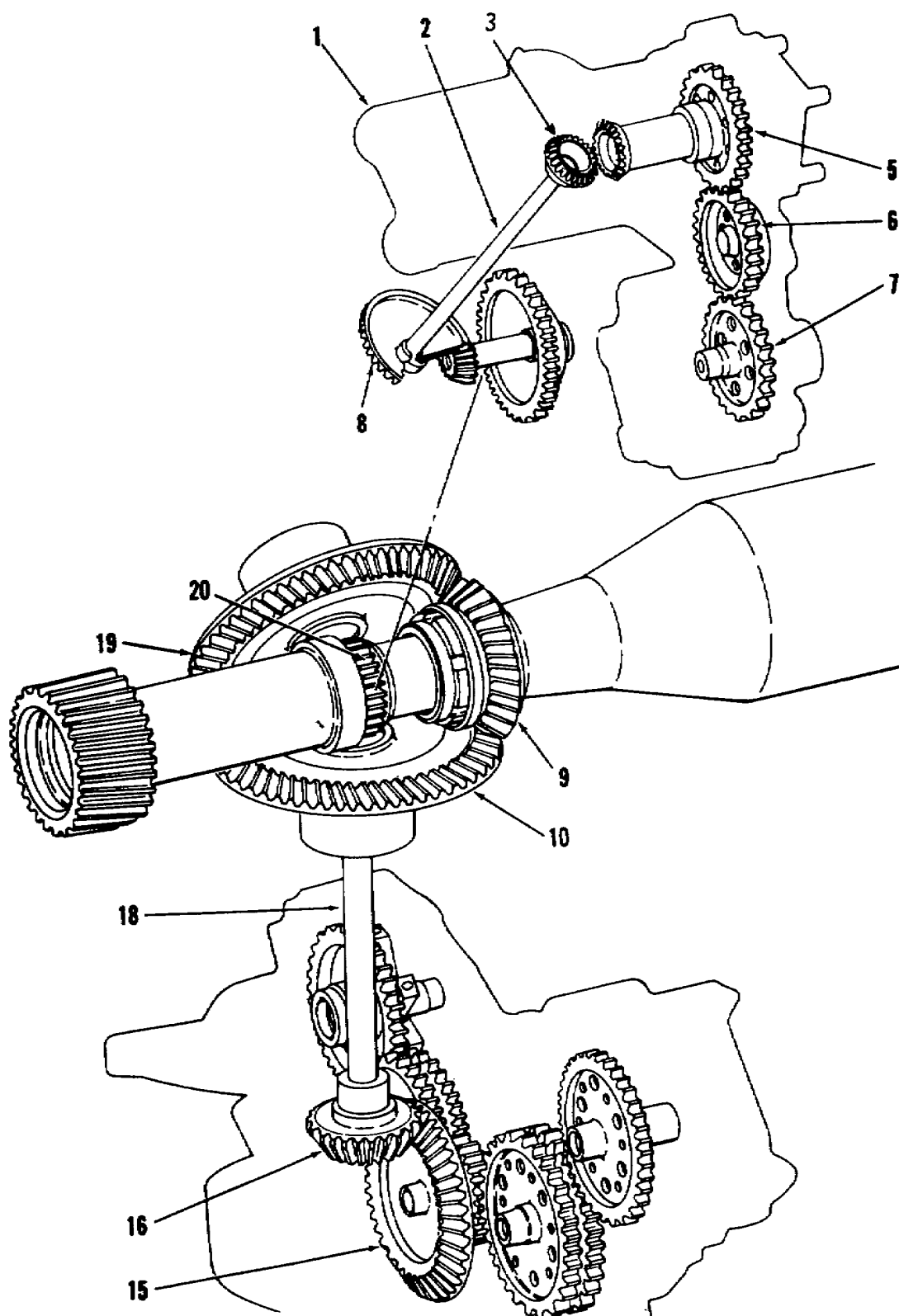
Figure 4.9. Accessory Drives.
