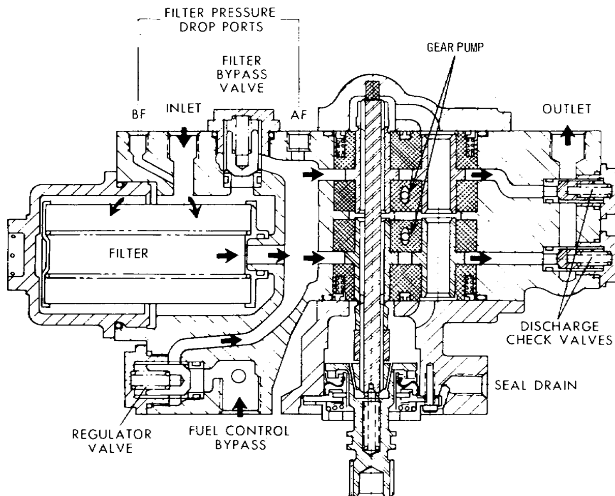
Figure 7.12. Fuel Pump and Filter Assembly.
