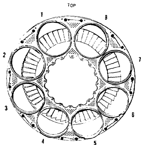
Figure 8.8. Combustion Chamber Outlet Duct and Combustor (Can) Positions.
