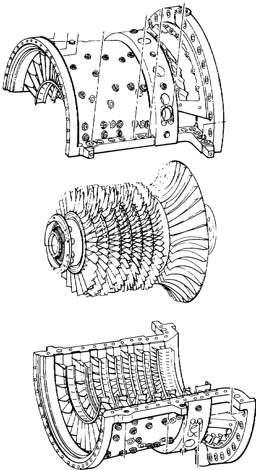
Figure 1.15. Axial-Centrifugal-Flow Compressor.
