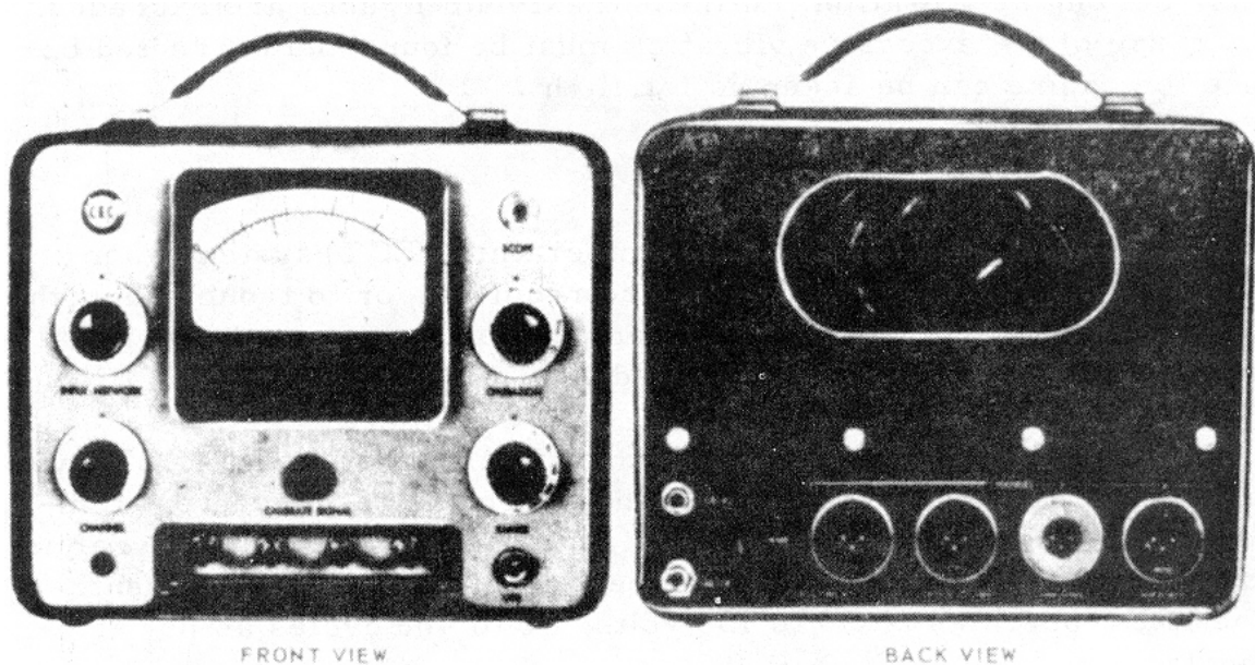
Figure 3.3. Vibration Meter.
