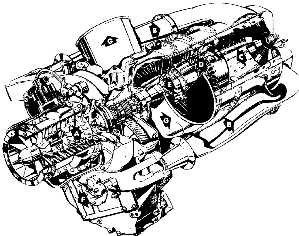
Figure 7.2. Airflow Diagram.
