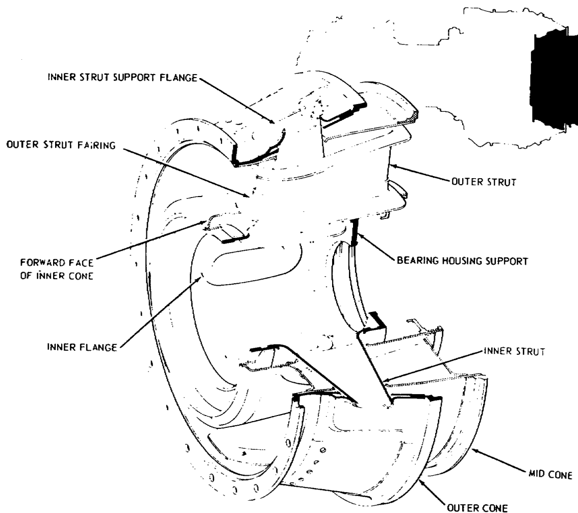
Figure 4.18. Exhaust Diffuser.
