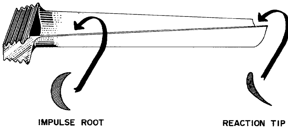
Figure 1.23. Impulse-Reaction Turbine Blade.
