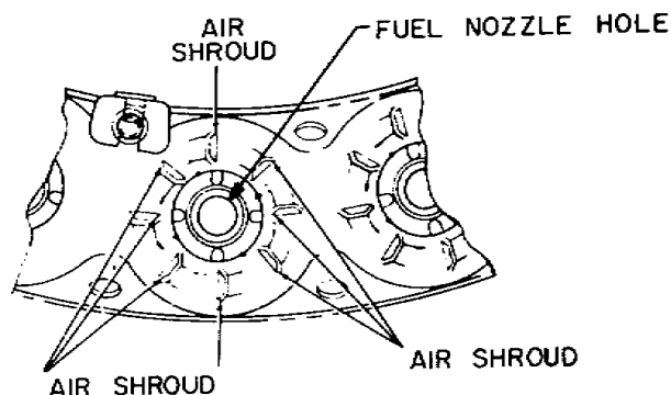
Figure 2.7. Air Shroud.
