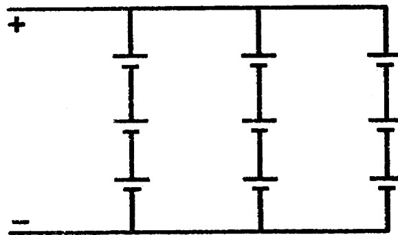
Series-Parallel-connected cells.
