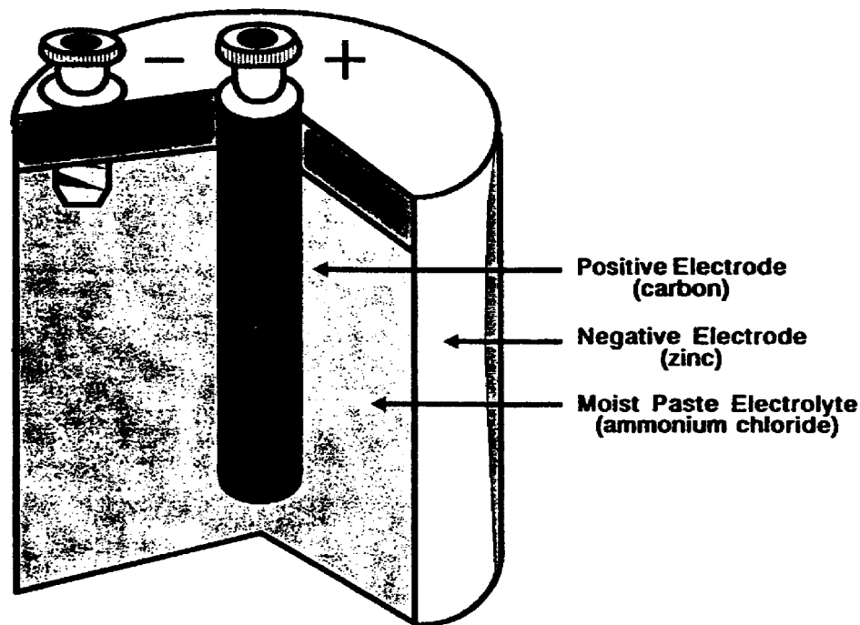
Figure 1-2. Primary Cell.
