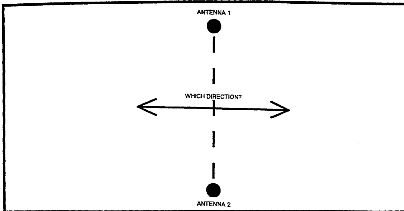
Figure 1-17. Bidirectional ambiguity.
