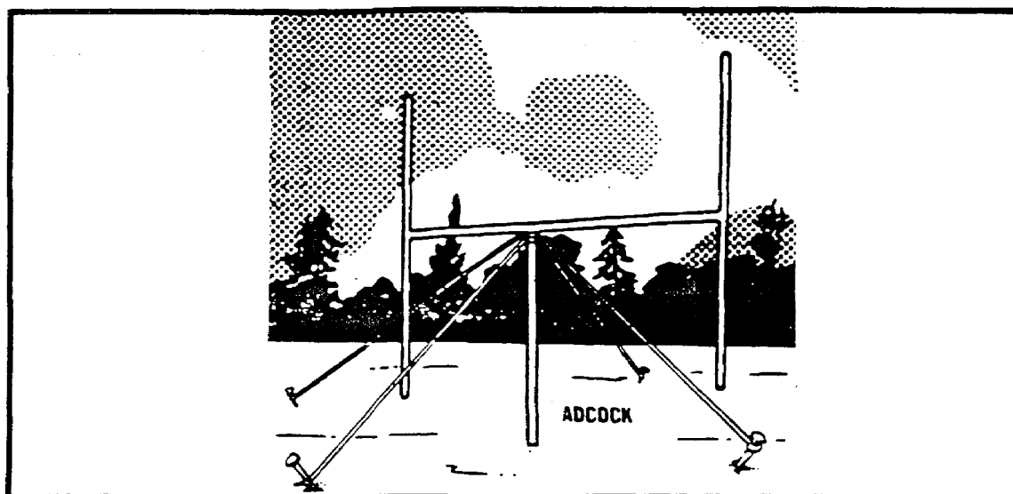
Figure 2-7. Adcock antenna.
