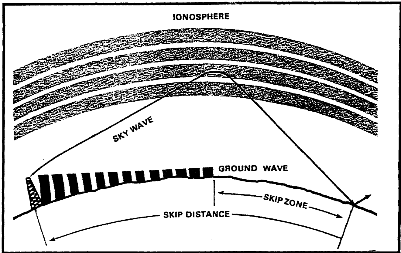
Figure 1-9. Skip zone and distance.
