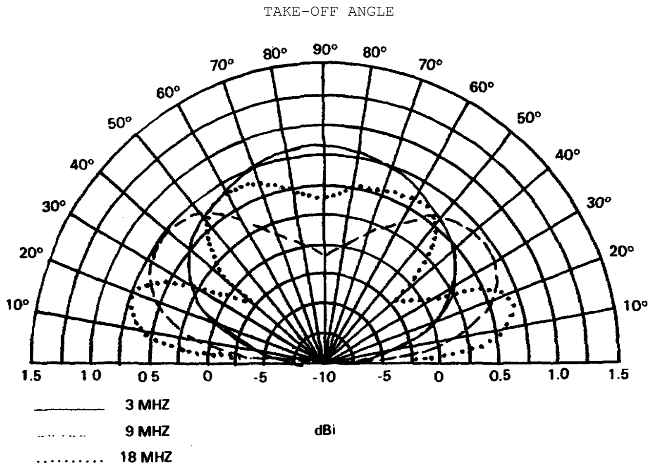
HALF-WAVE DOUBLET ANTENNA VERTICAL PATTERN, HEIGHT 40 FEET
