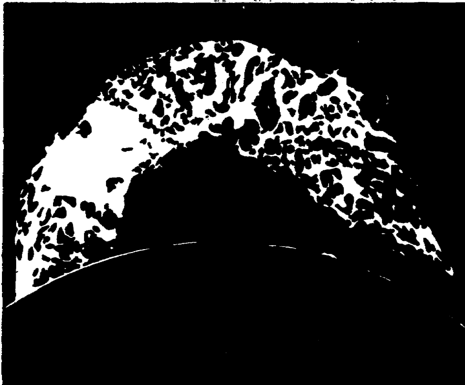
Figure 10. Solar eruption.
