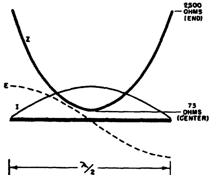
Figure 30. Impedance along half-wave antenna.
