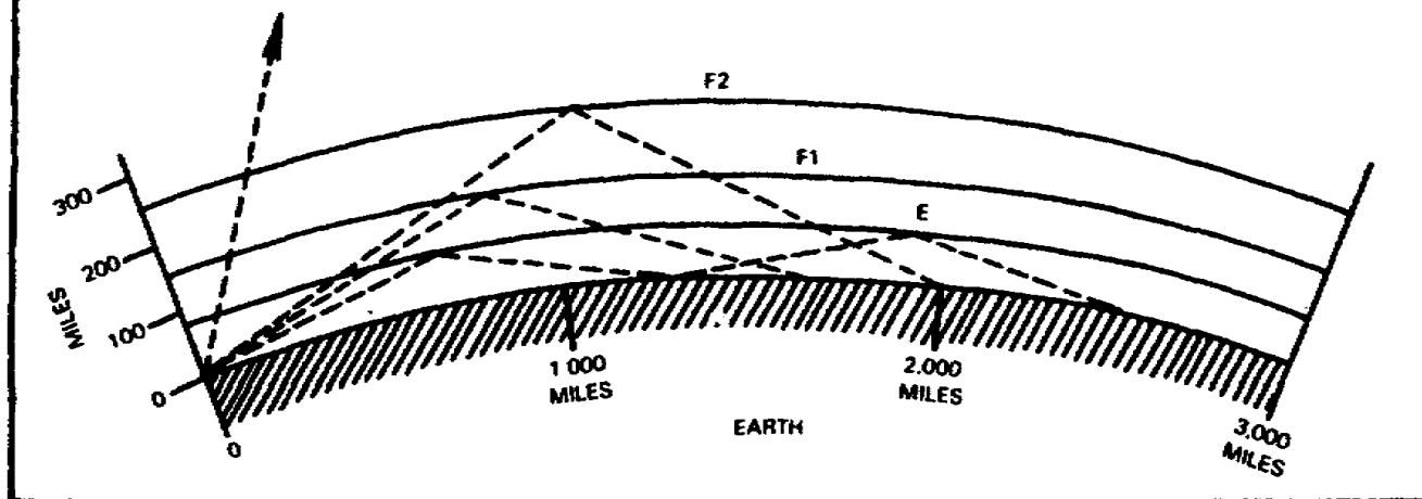
Figure 28. Frequency versus distance for returned waves.
