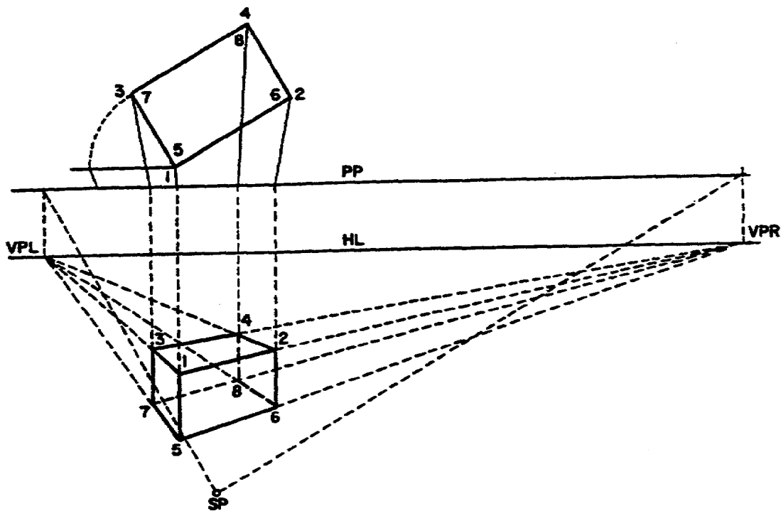
Figure 2-4. Two-point perspective drawing made without using an elevation of the object
