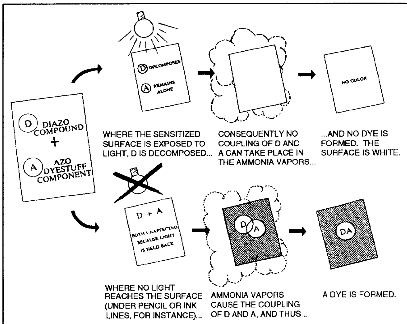
Figure 2-2. Simplified diazo process
