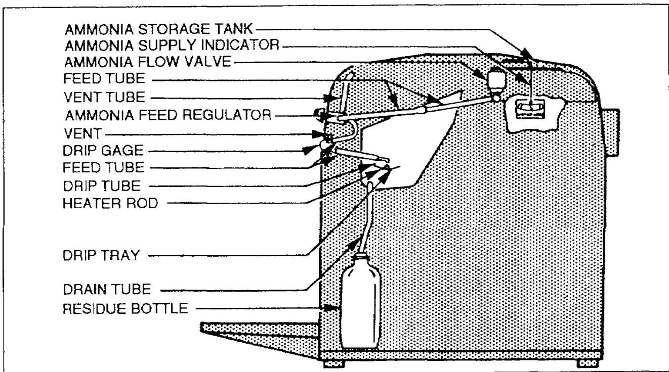
Figure 2-6. Basic ammonia flow system
