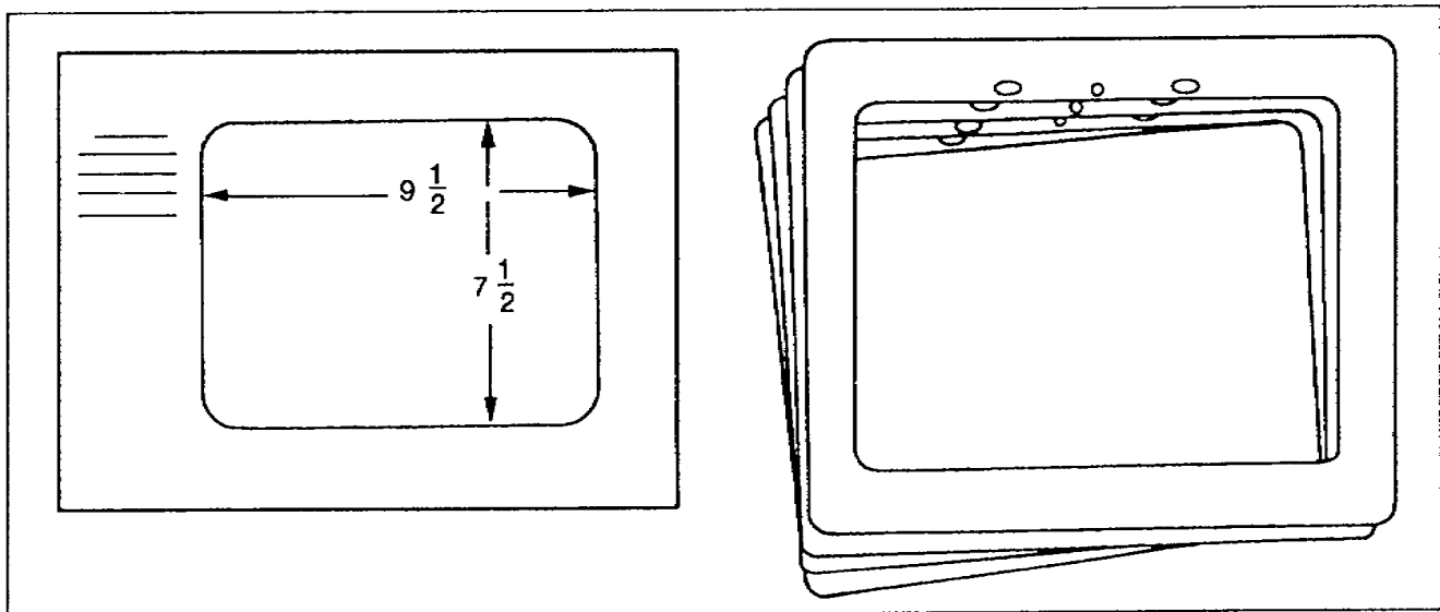
Figure 2-8. VGT mounting frames
