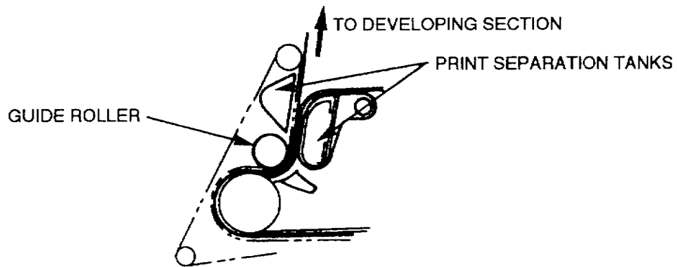
2. SEPARATION PROCESS
