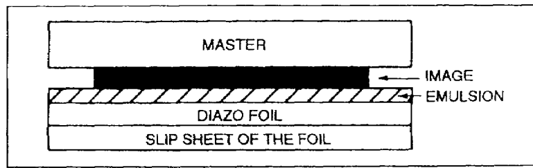
Figure 2-7. Diazo foil with slip sheet
