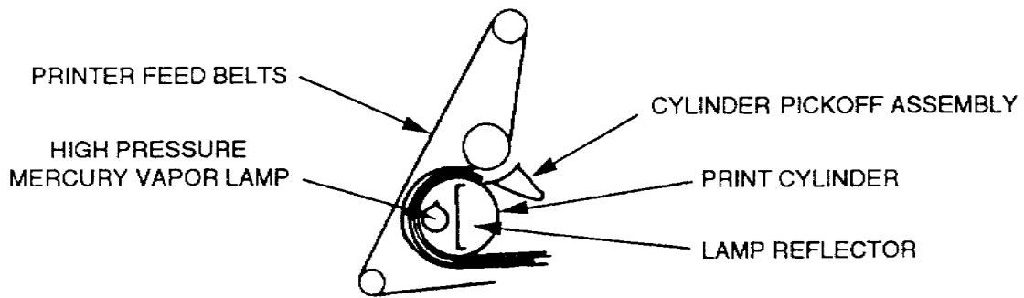
1. PRINTING SECTION
