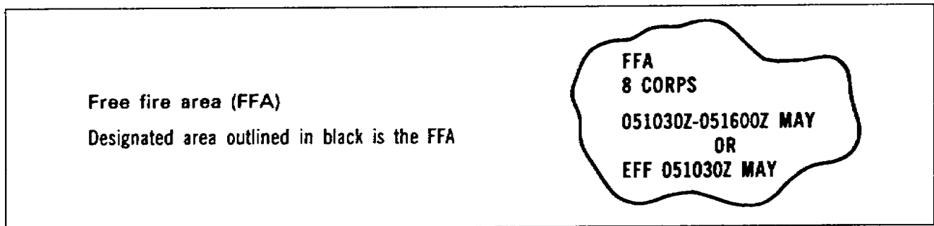
Figure 1-15. Free-fire area
