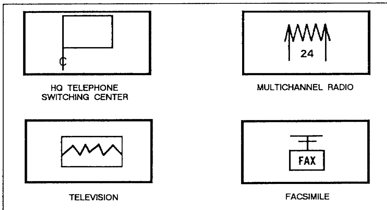
Figure 1-9. C-E emitter symbols
