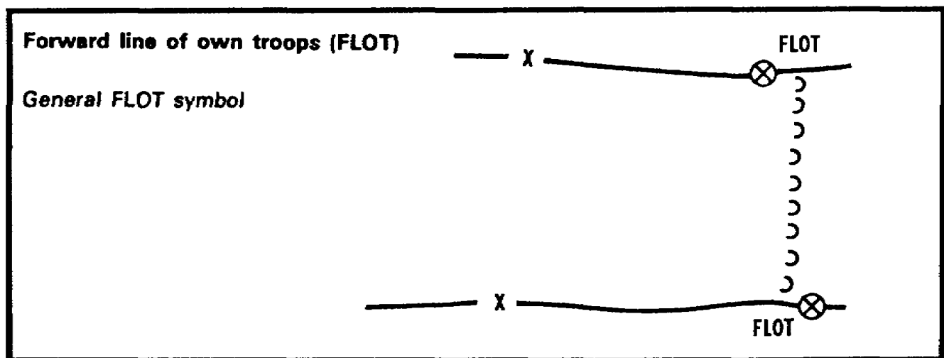
Figure 1-14. FLOT line
