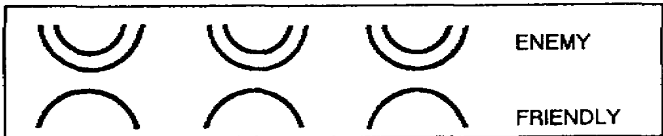
Figure 1-11. Single-color symbols
