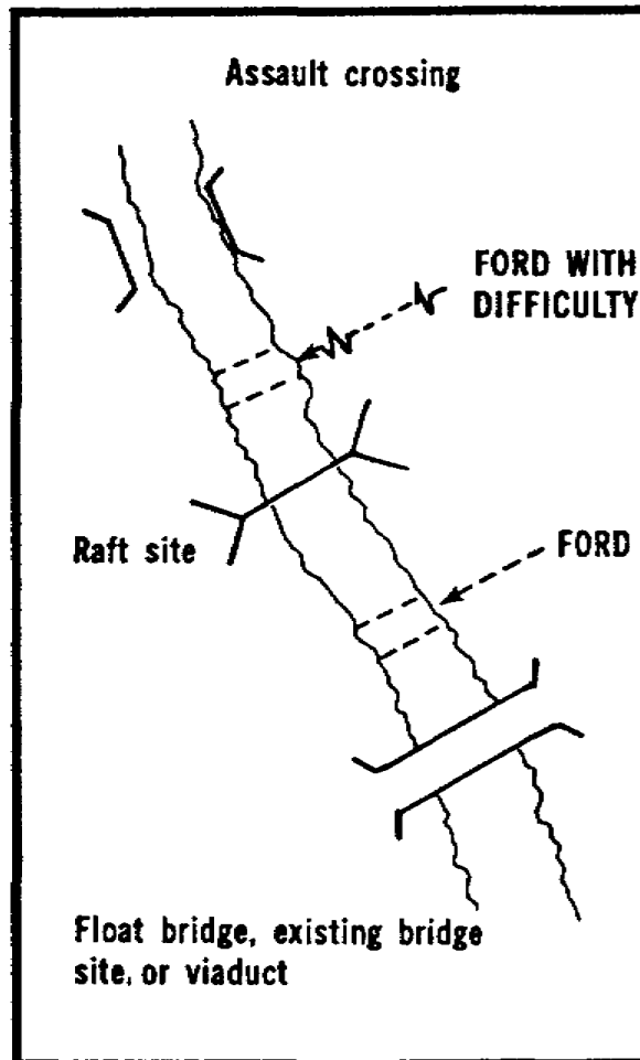
Figure 1-18. Crossing sites
