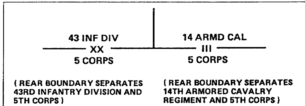
Figure 1-21. Rear boundaries
