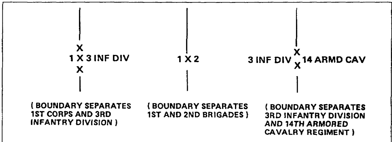
Figure 1-20. Lateral boundaries
