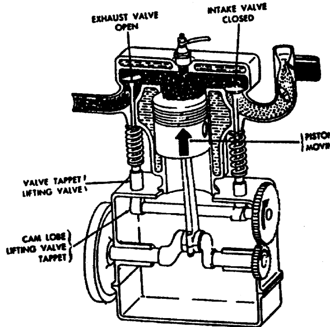
Figure 1-10. Exhaust Stroke.
