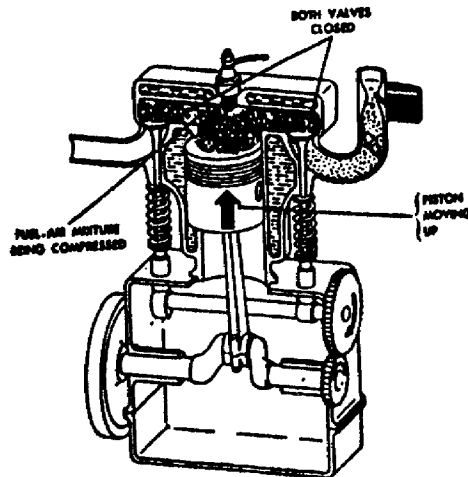
Figure 1-8. Compression Stroke.
