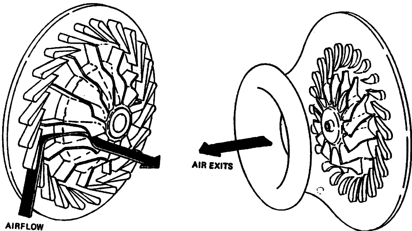
Figure 1-25. Radial Inflow Turbine.
