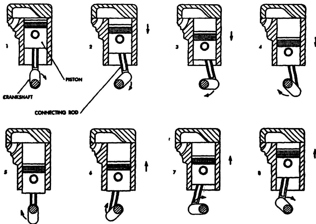
Figure 1-4. Relationship of Piston, Connecting Rod, and Crank on Crankshaft as Crankshaft Turns One Revolution.
