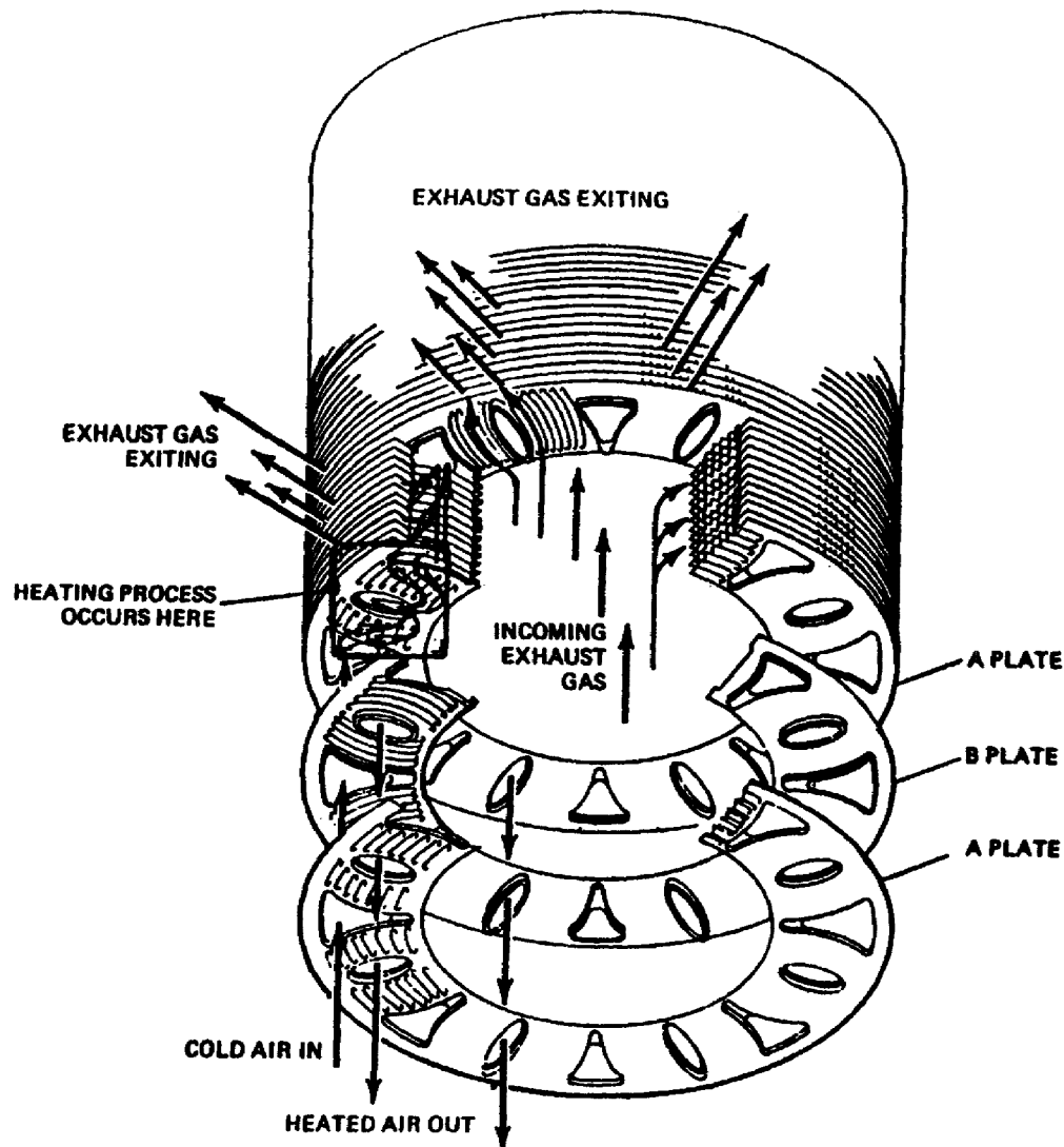
Figure 1-23. Typical Recouperator.
