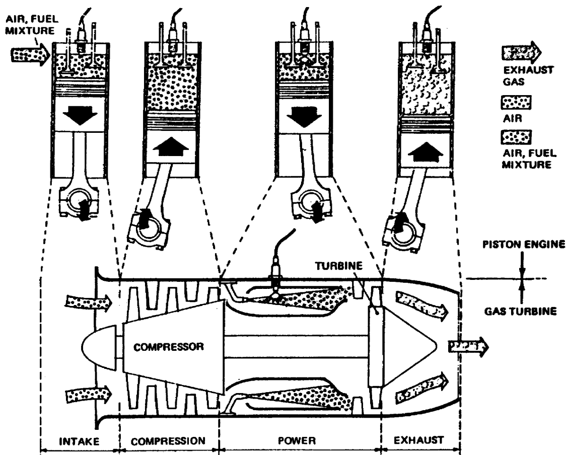
Figure 1-18. Comparison of Piston Engine to Turbine Engine.
