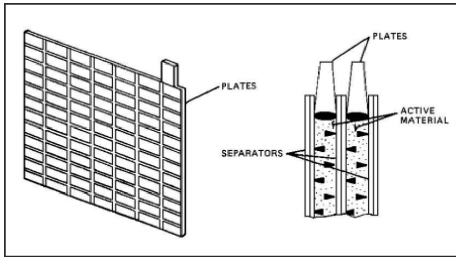
FIGURE 15. PLATE CONSTRUCTION.
