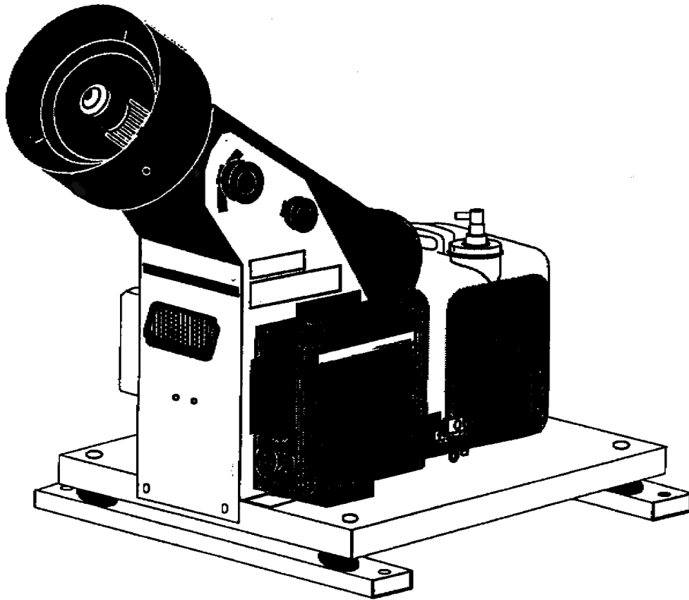
Figure 3-10. Aerosol generated ultra-low volume electric sprayer (AGULVE).
