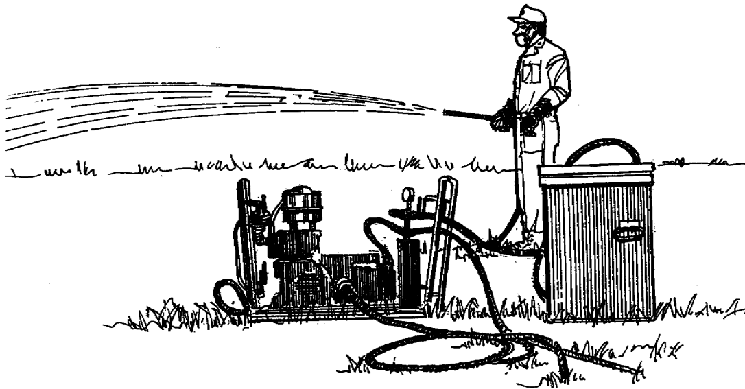
Figure 3-9. Hydraulic sprayer.
