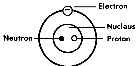
Figure 2-1. Components of the atom.
