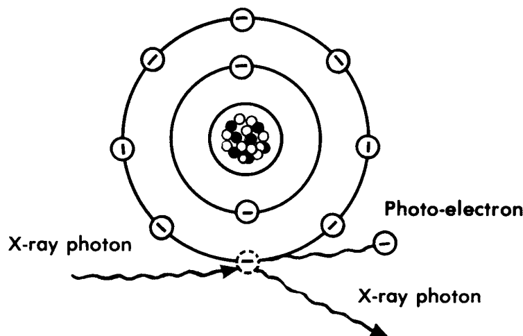
Figure 2-8. Indirect photon hit upon an electron.
