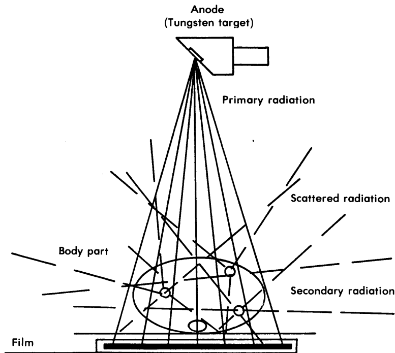
Figure 1-6. Diagram of scattered/secondary radiation.
