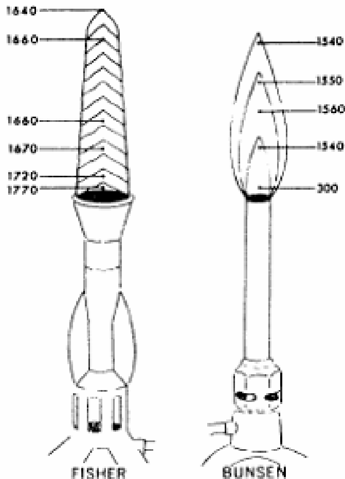
Figure 1-6. Temperature comparison of the Fisher and Bunsen burners.
