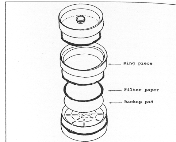
Figure 2-9. Filters.
