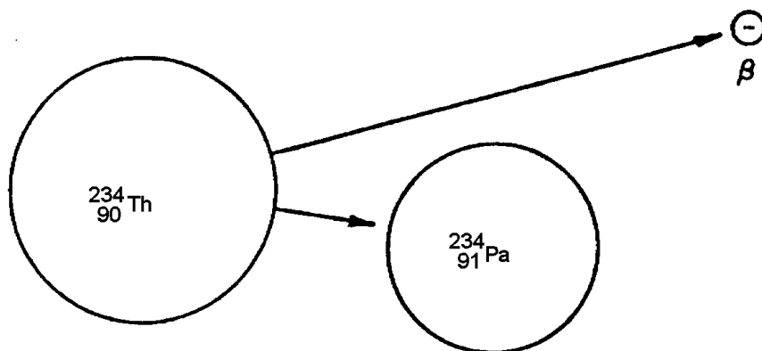
Figure 1-8. Beta emission from Th-234.
