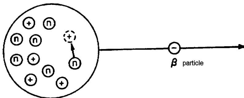
Figure 1-7. Beta emission.
