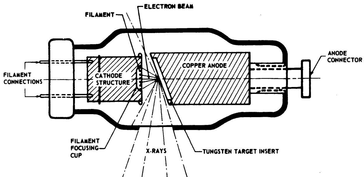
Figure 2-1. X-ray tube.
