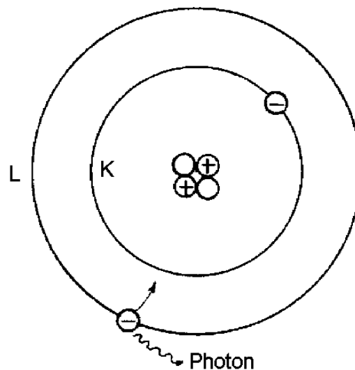
Figure 1-4. Excited atom.
