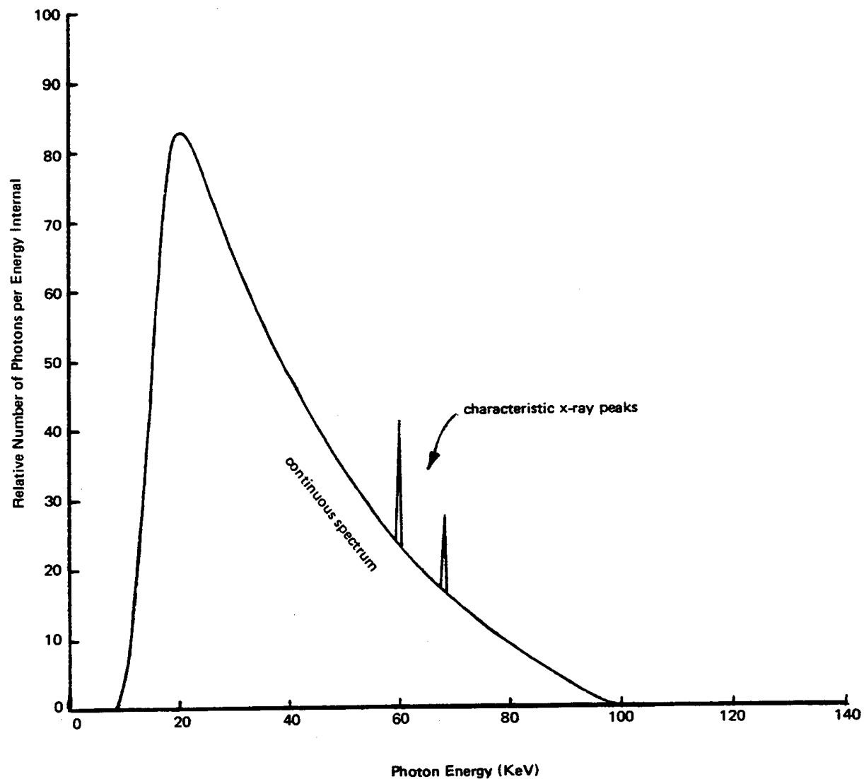
Figure 2-2. X-ray spectrum.
