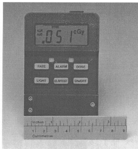
Figure 1-11. Pocket Radiac – AN/UDR-13
