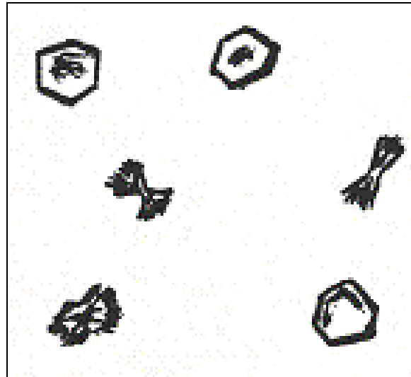
Figure 3-27. Sulfathiazole crystals.
