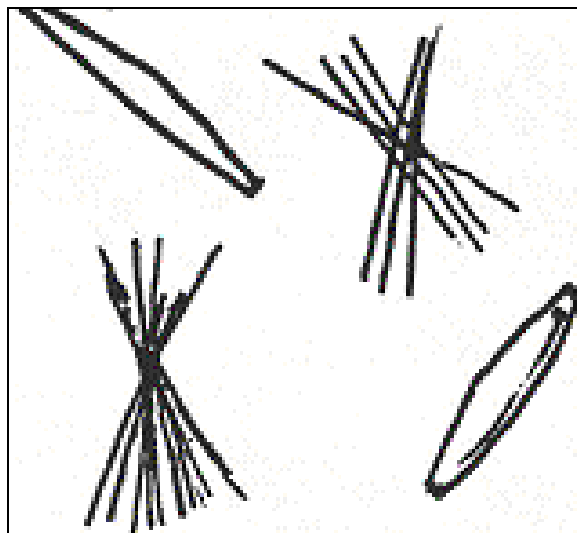
Figure 3-29. Sulfaguanidine crystals.
