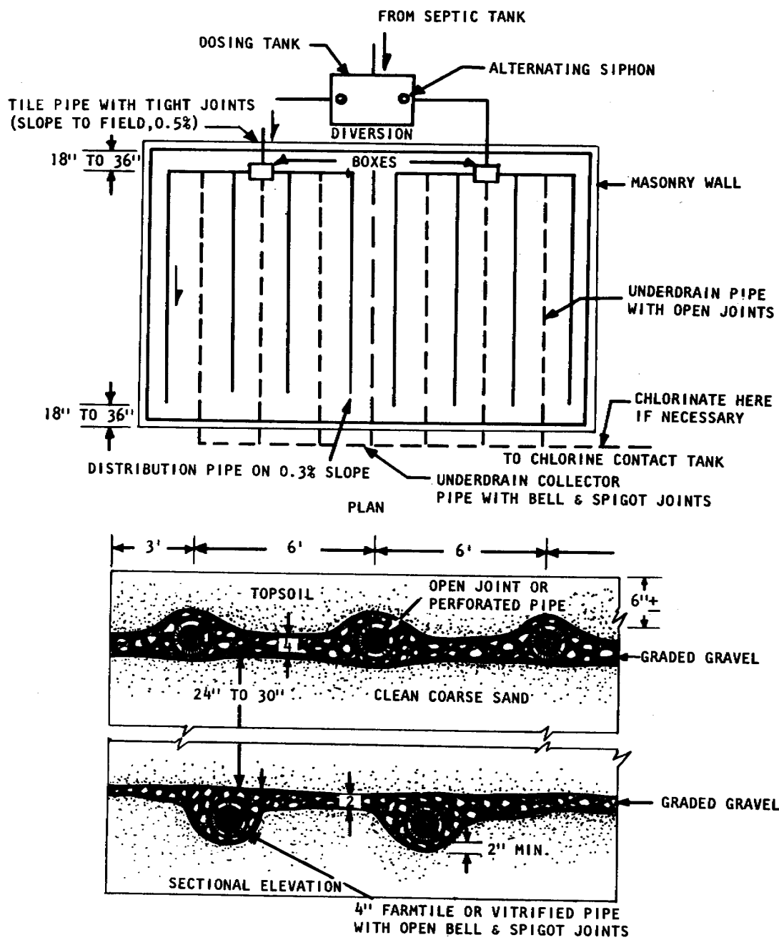
Figure 1-18. Underdrained sand filter trench.
