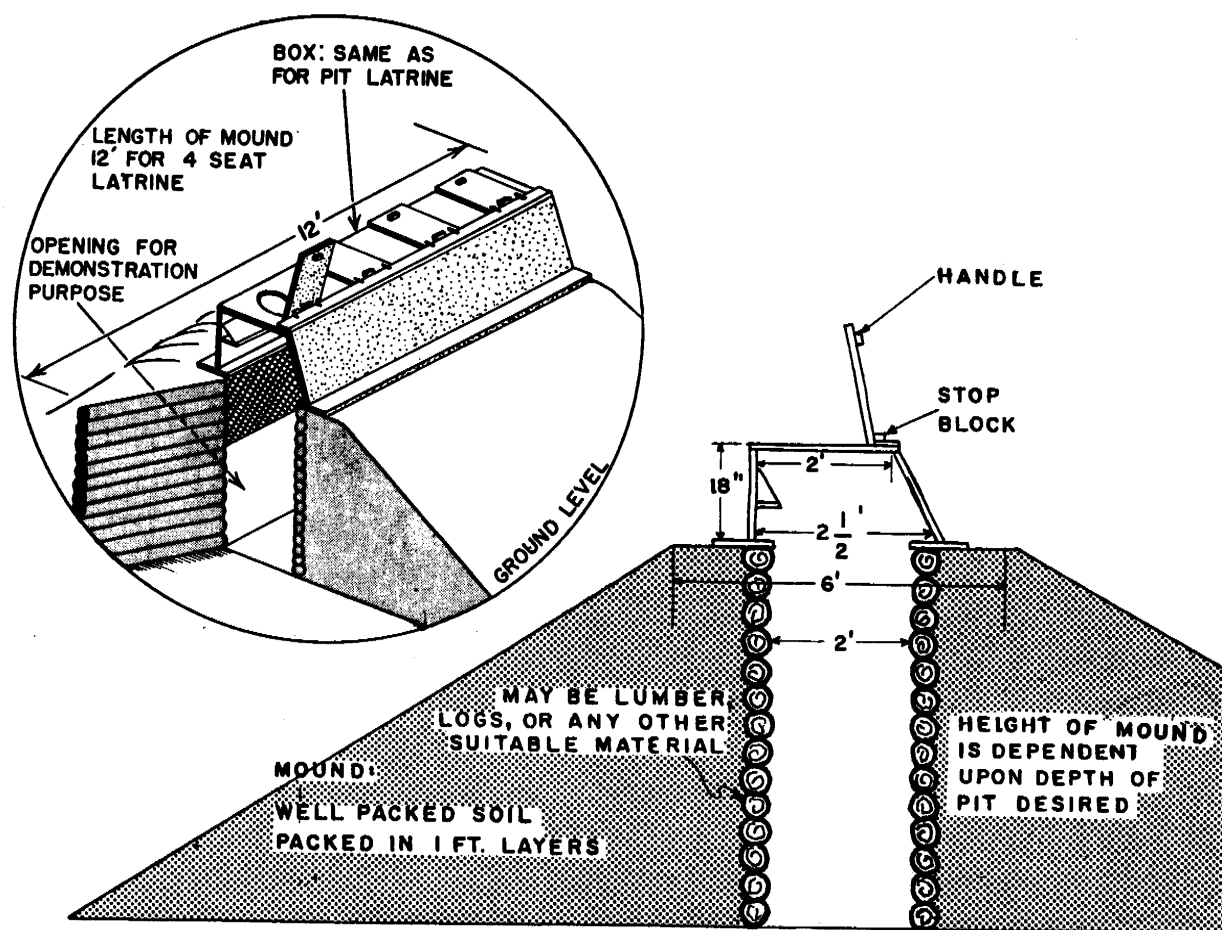
Figure 3-5. Mound latrine.
