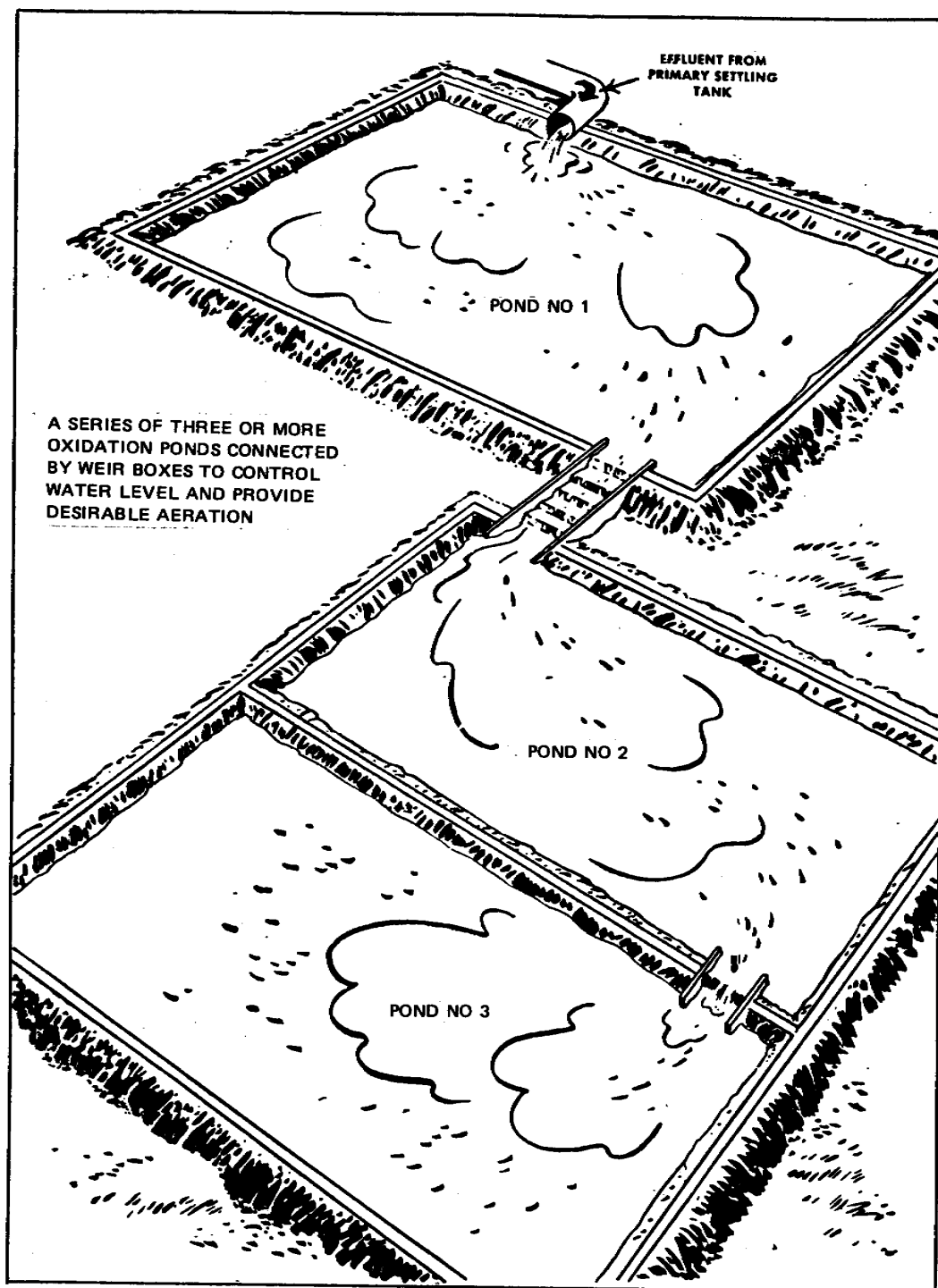
Figure 2-28. Oxidation ponds.
