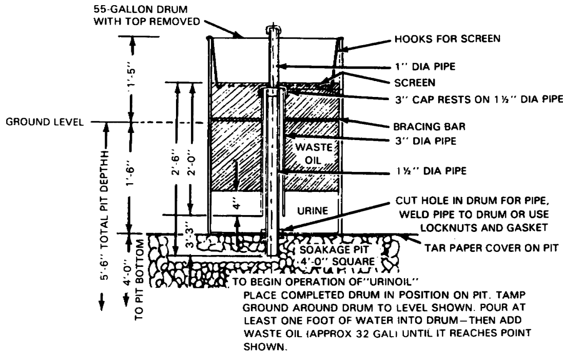
Figure 3-10. Urinoil urinal.
