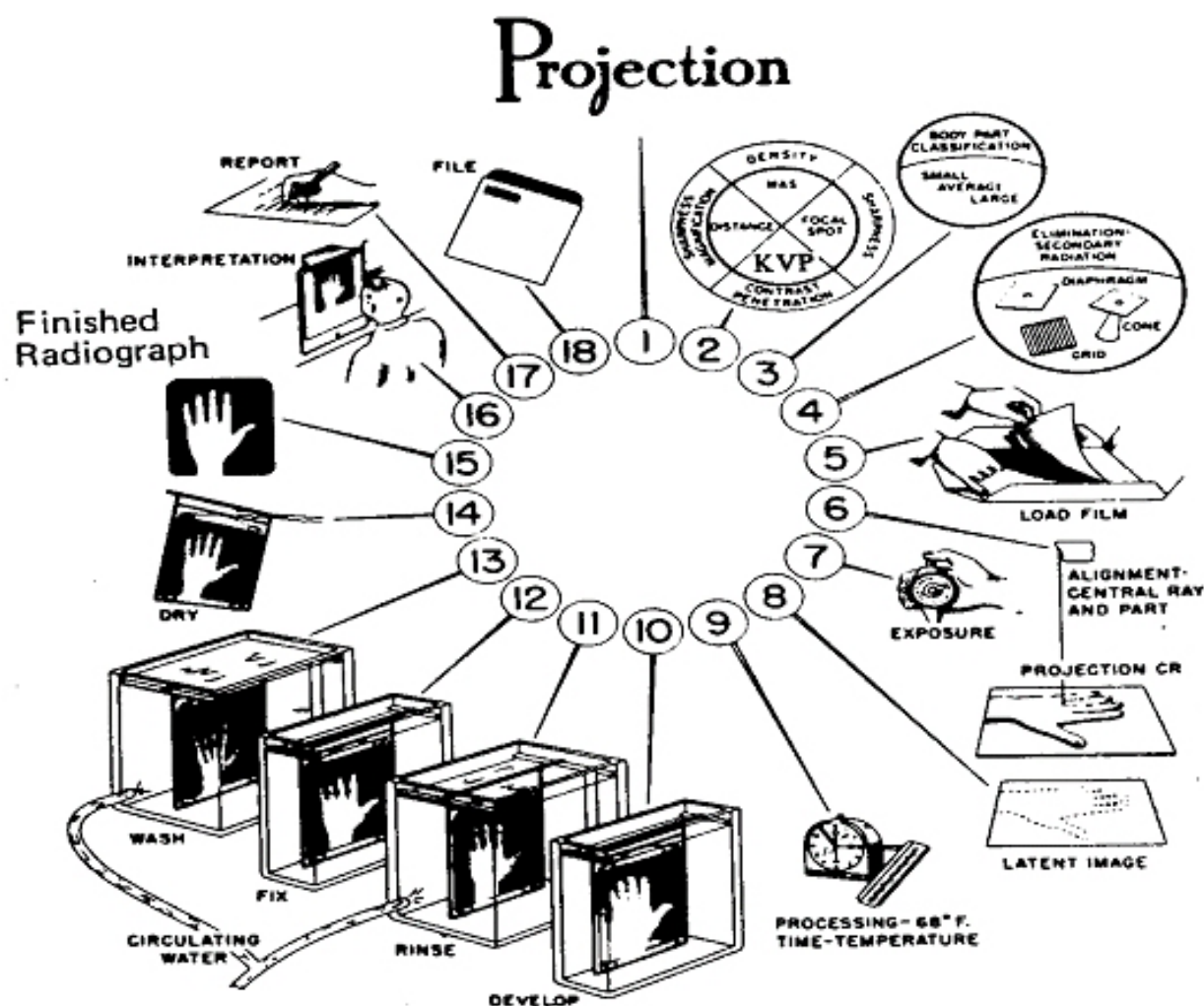
Figure 1-1. Steps in production of a radiograph.
