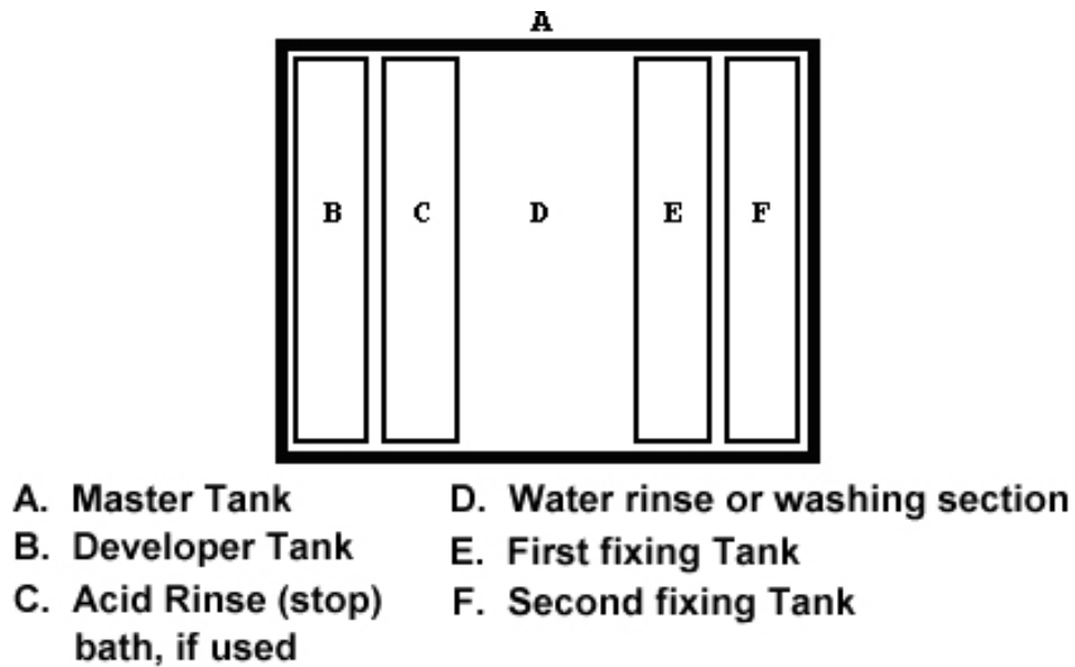
Figure 2-6. Conventional arrangement of a small tank unit (top view).
