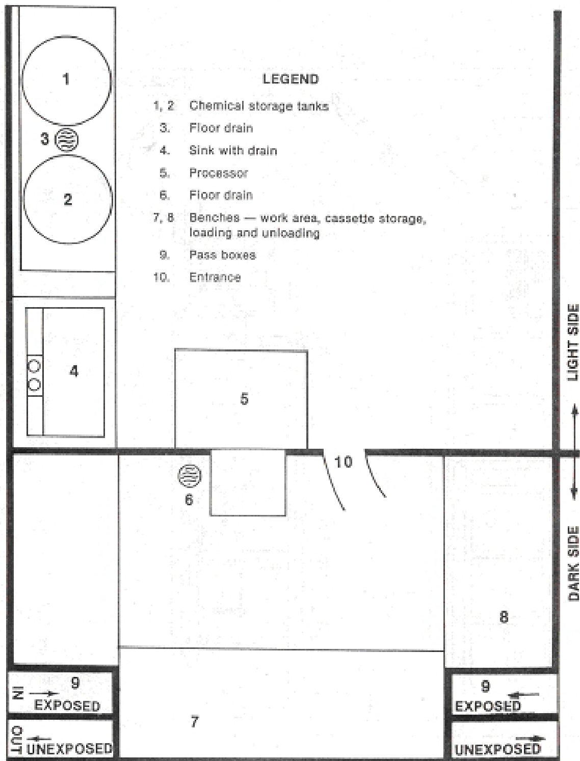
Figure 2-1. A schematic diagram of an automatic processing darkroom and adjacent light room area.
