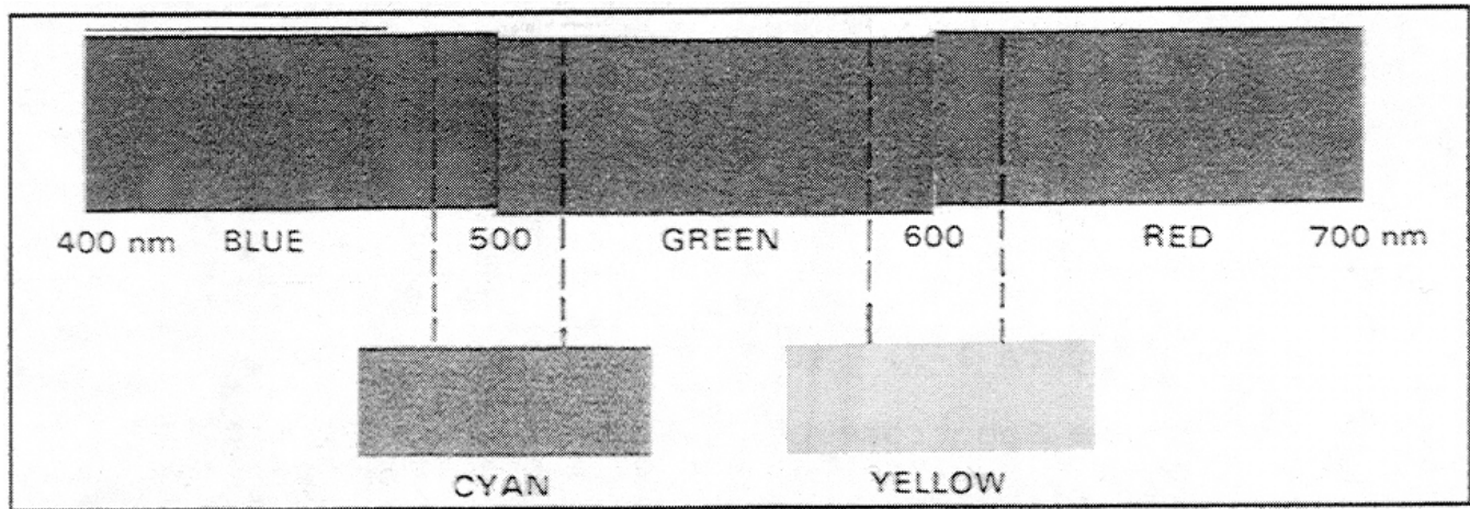
Figure 1-4. Visible spectrum
