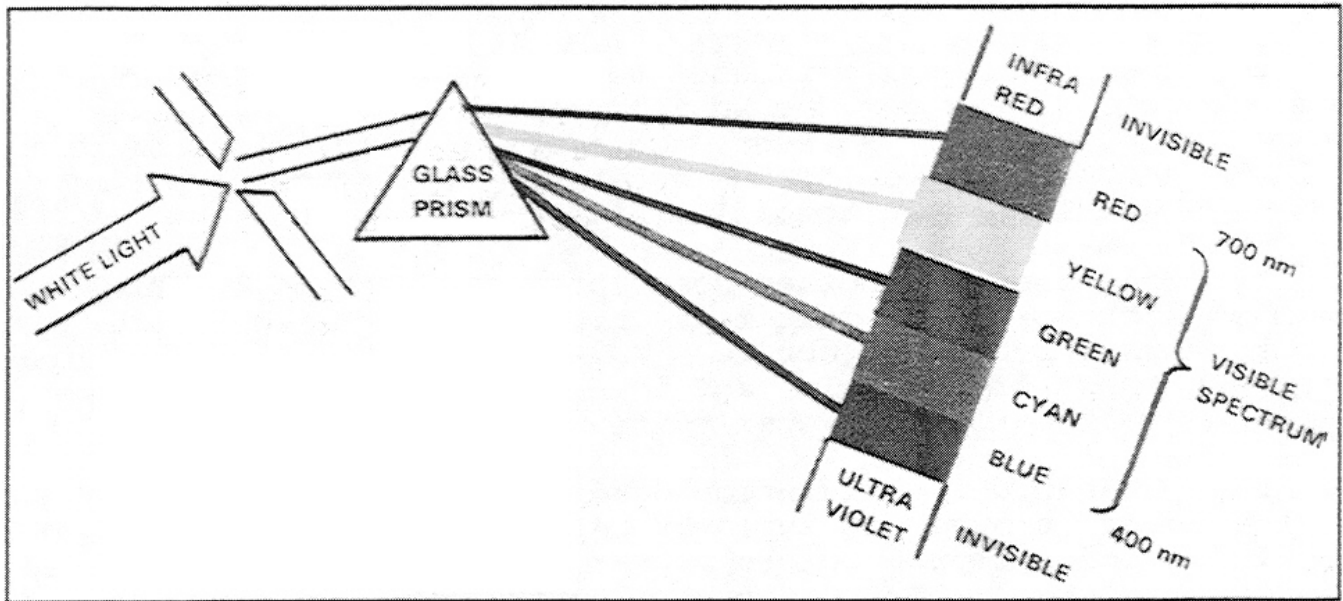
Figure 1-9. Dispersion
