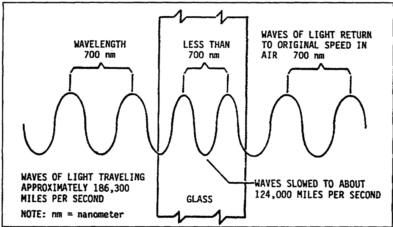
Figure 1-2. Traveling of light waves
