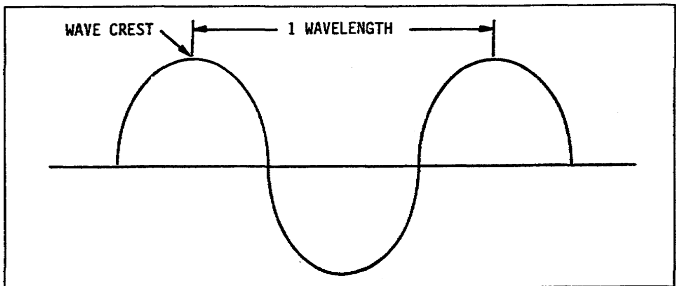
Figure 1-1. A wavelength
