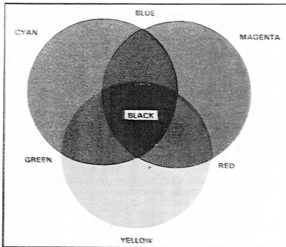
Figure 1-7. Subtractive color process
