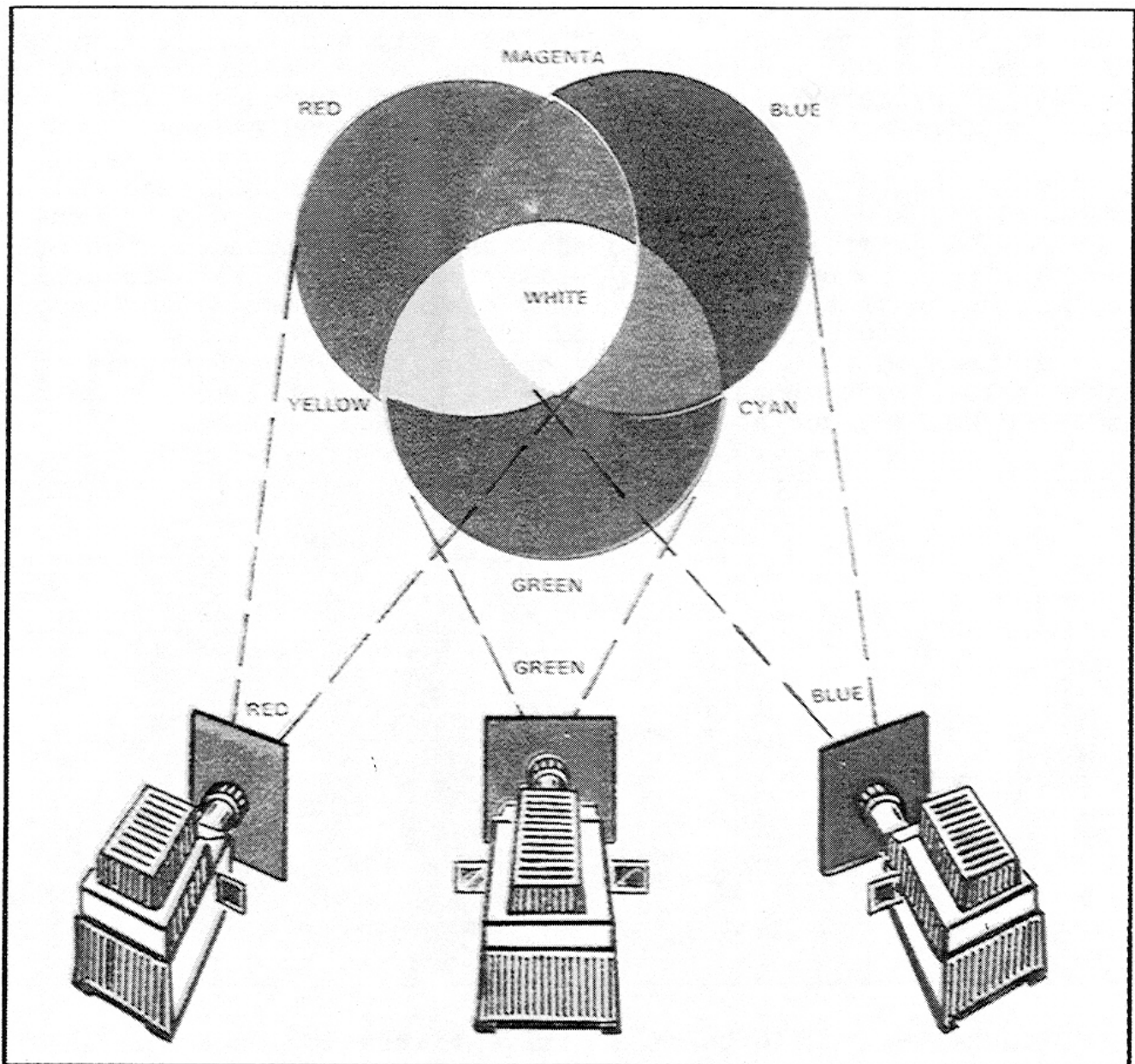
Figure 1-5. Principle and colors of the additive color process
