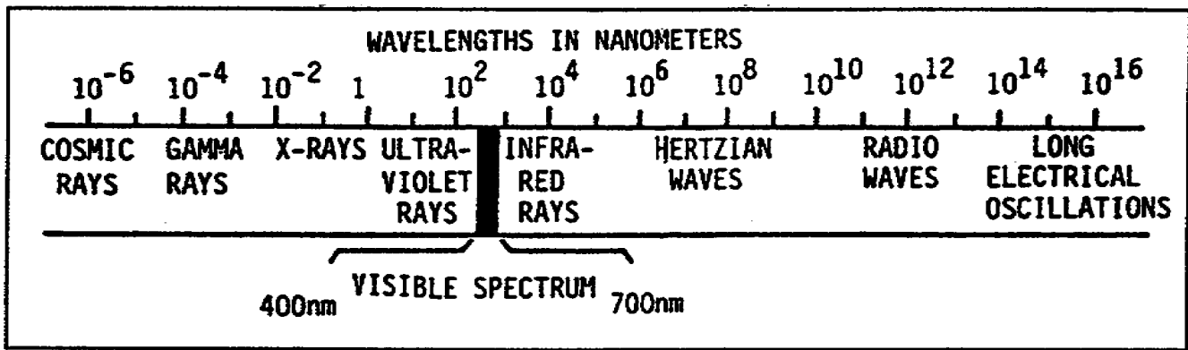
Figure 1-3. Electromagnetic spectrum
