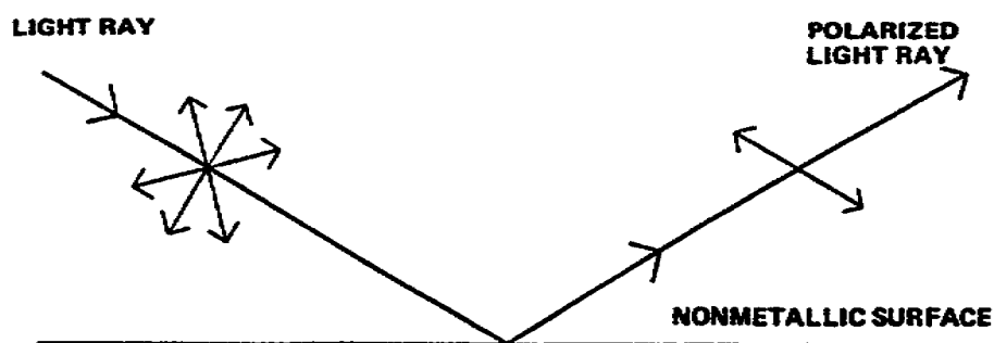
Figure 2-8. Polarized light
