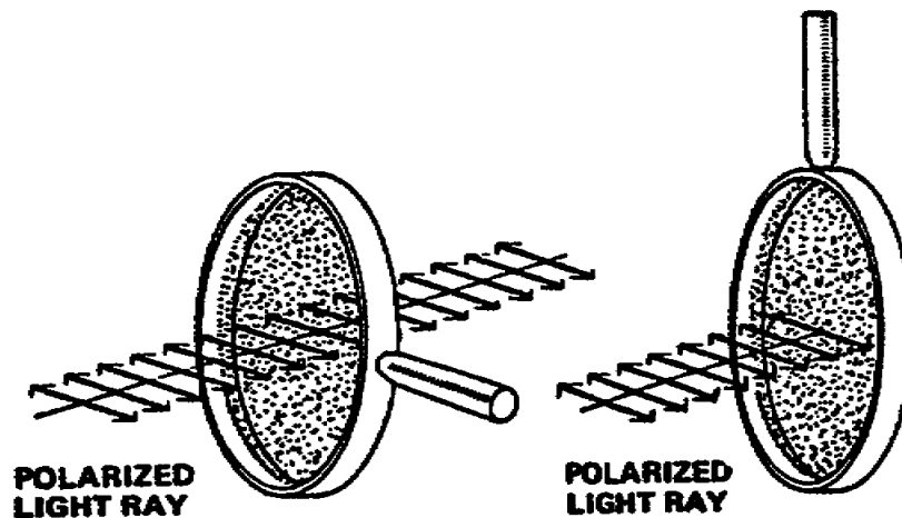
Figure 2-9. Polarized light
