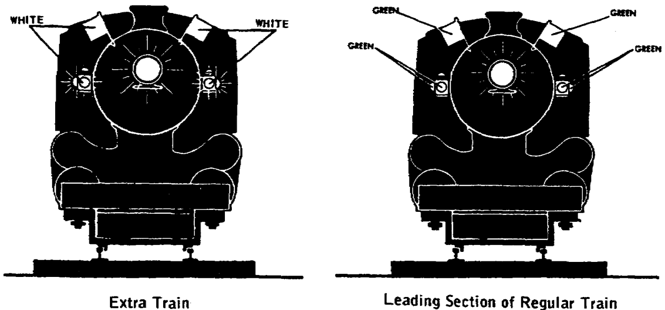
Figure 2.6. Train Classification Signals.
