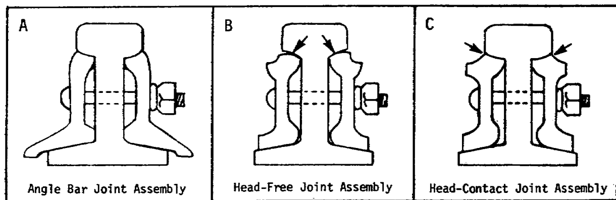
Figure 3.19. Types of Rail Joint Assemblies.
