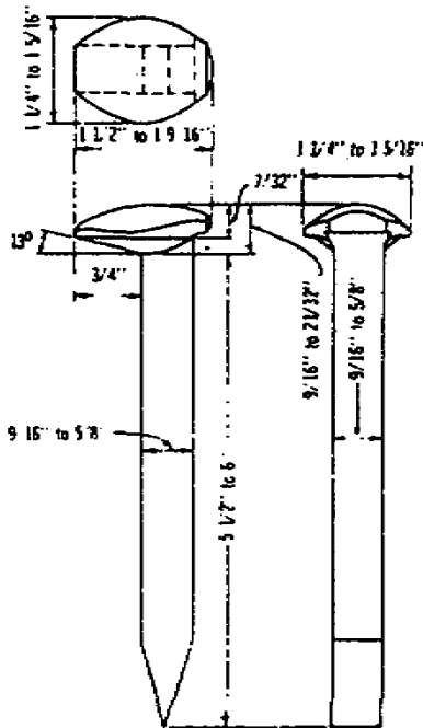
Figure 3.9. Details of Cut Spike.
