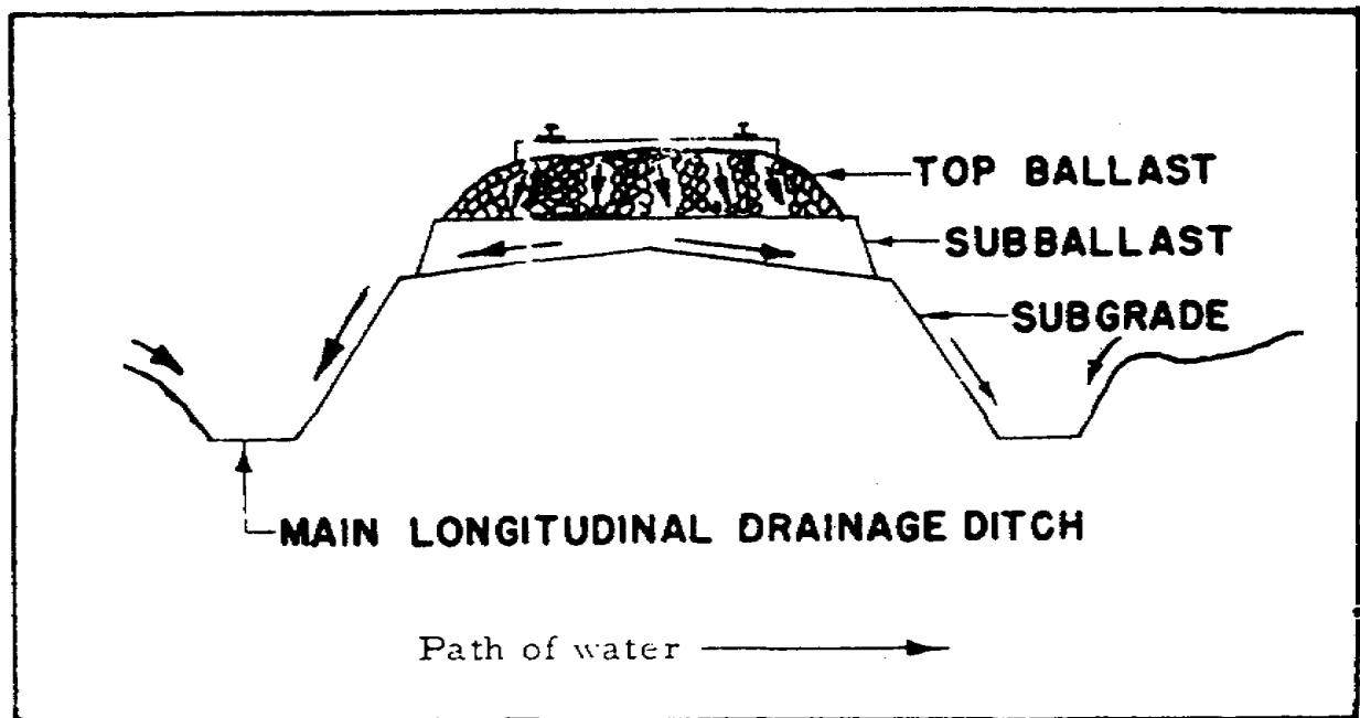
Figure 2.5. Ballast As Drainage Medium.
