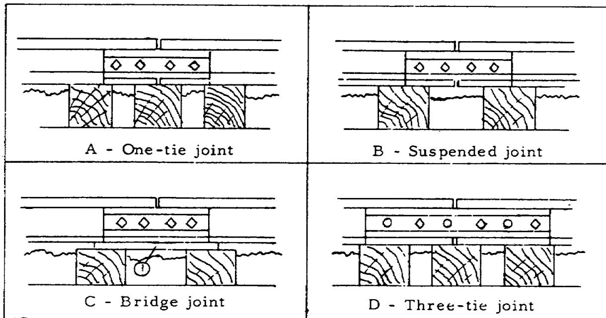
Figure 3.20. Methods of Joint Support .
