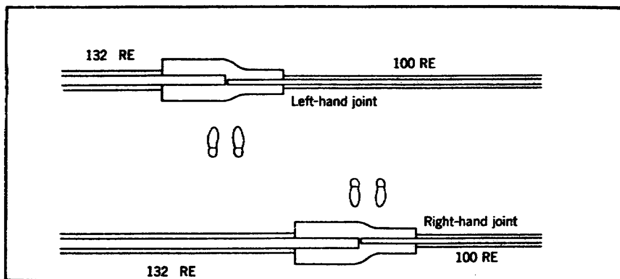
Figure 3.22. Designations of Compromise Bars.
