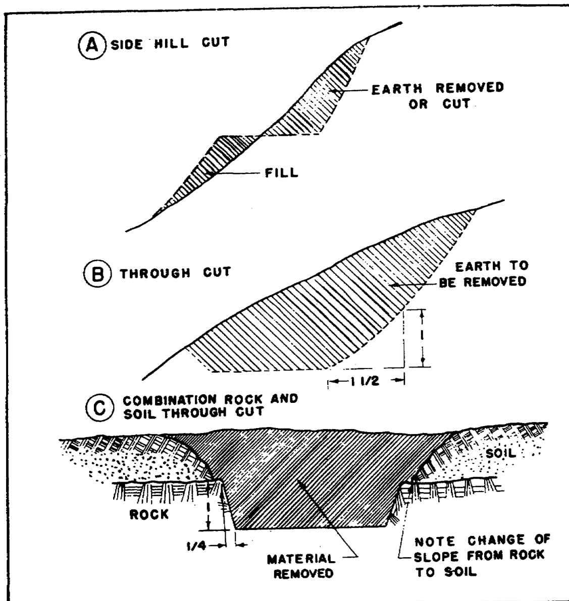
Figure 2.2. Kinds of Cuts.
