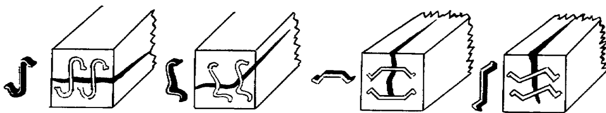
Figure 3.5. Antisplitting Irons.
