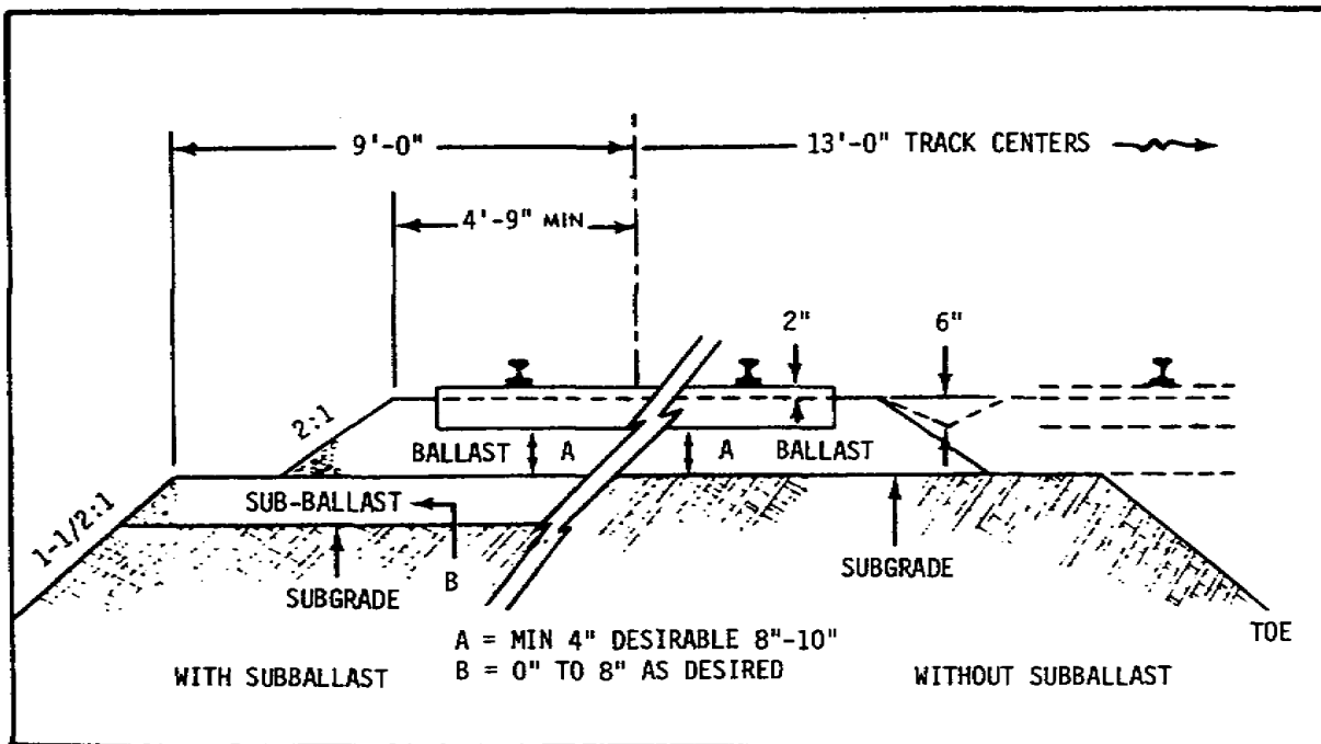
Figure 2.3. Typical Main-Line Ballast Section
