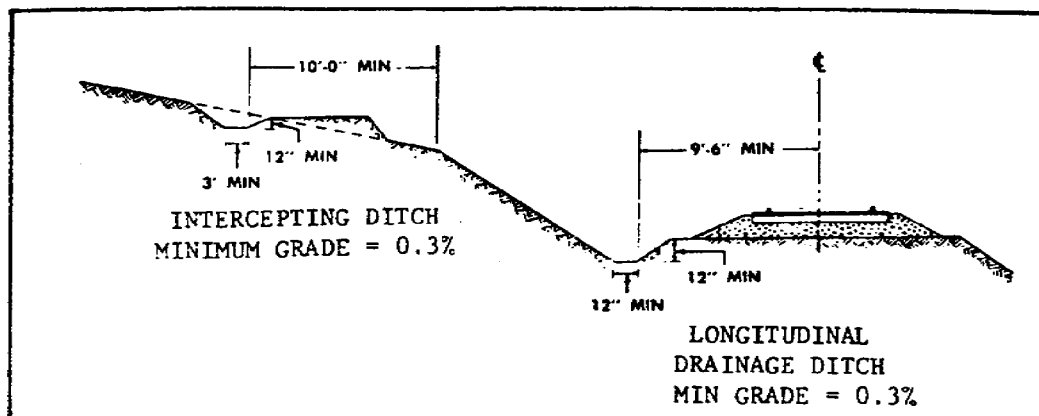
Figure 2.7. Minimum Dimensions and Grades of Intercepting and Longitudinal Ditches.
