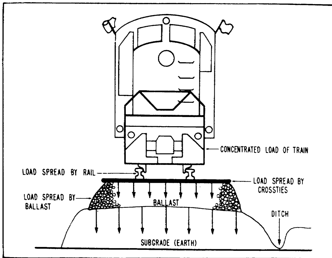
Figure 2.1. Spreading Train Weight to Roadbed.
