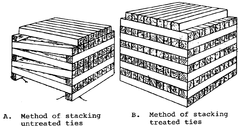
Figure 3.6. Methods of Stacking Ties.
