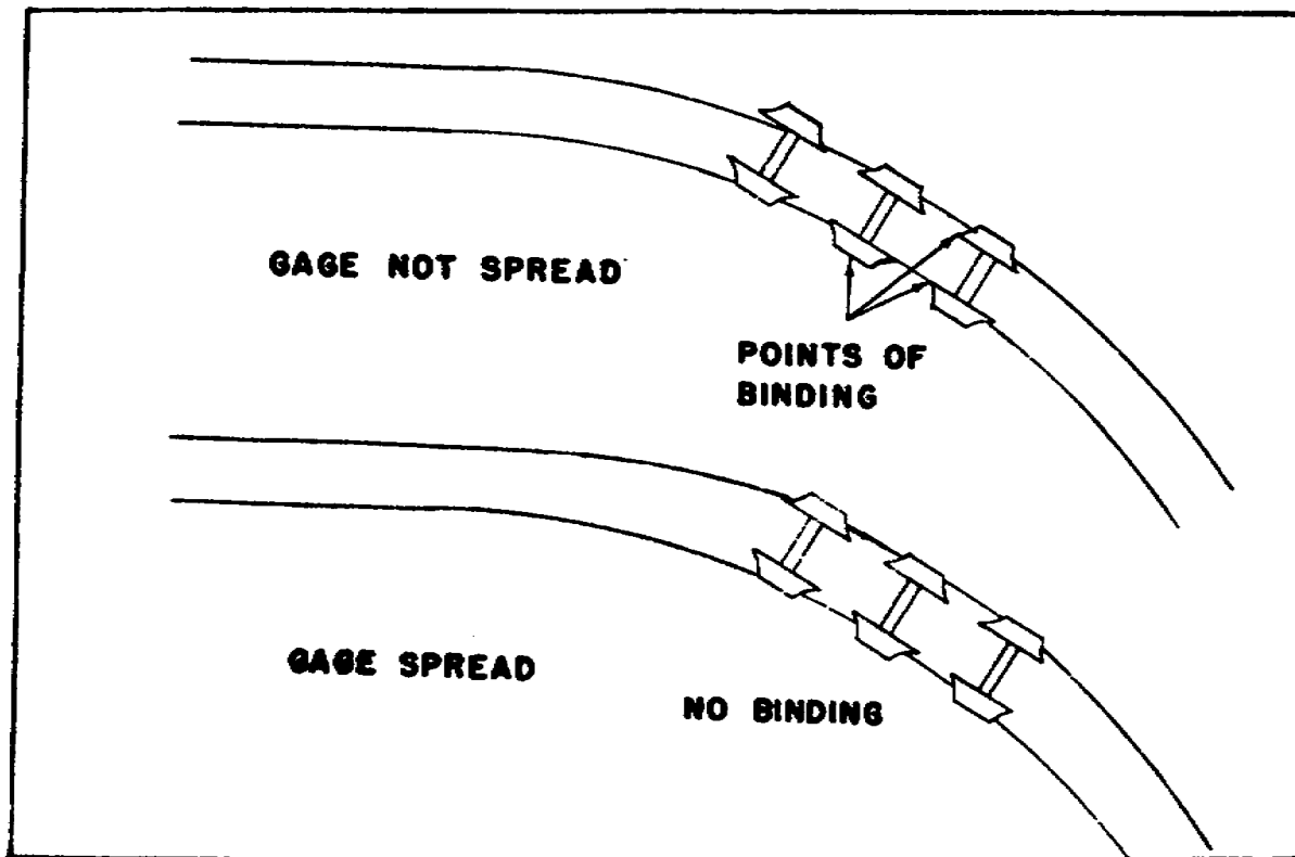
Figure 1.7. Gage on Sharp Curves.
