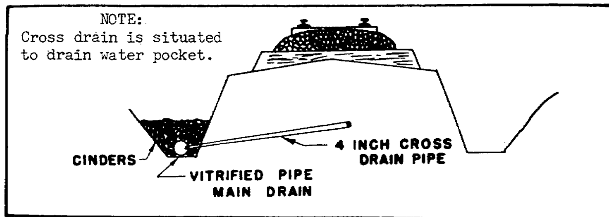
Figure 2.8. Cross Drain Installation With Pipe Drain in Subgrade.
