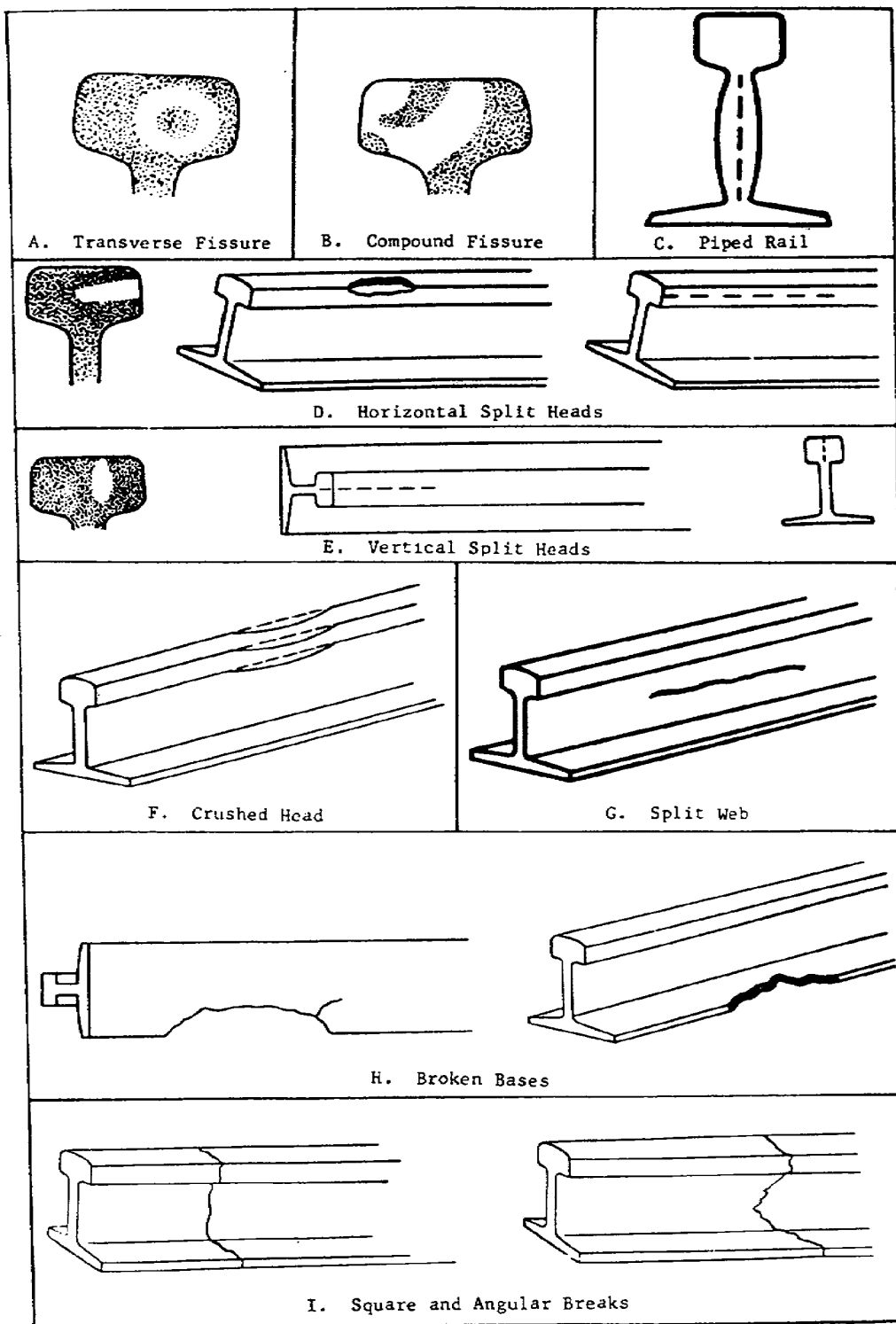
Figure 3.2. Rail Defects.
