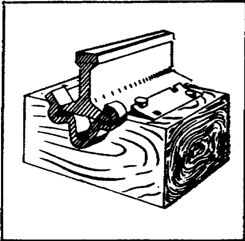
Figure 3.14. Typical Rail Anchor.
