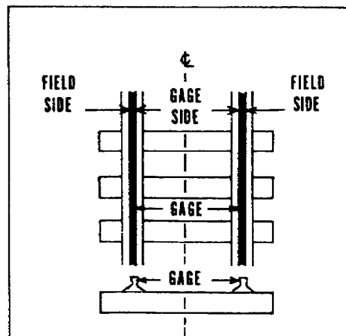
Figure 1.6. Rail Gage.
