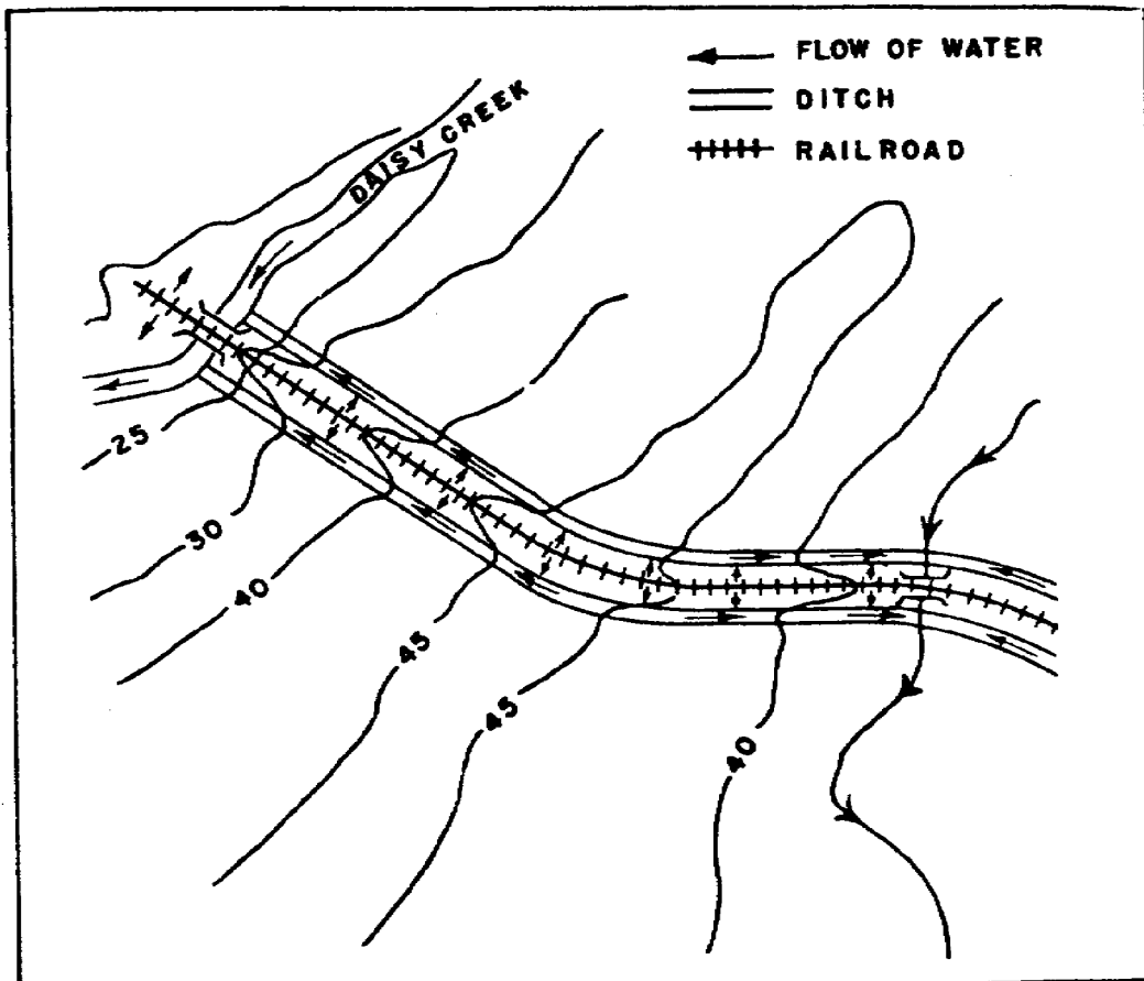
Figure 2.6. Principles of Longitudinal Drainage.
