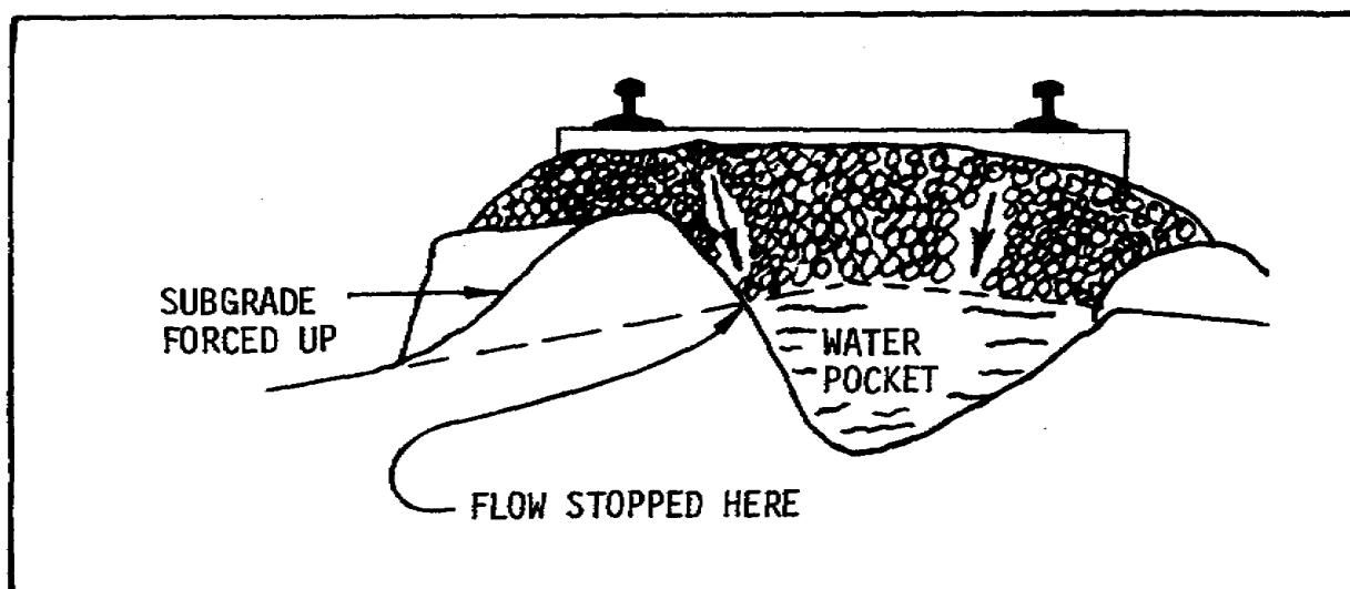
Figure 2.4. Drainage Obstructed When Subsoil Forced Up
