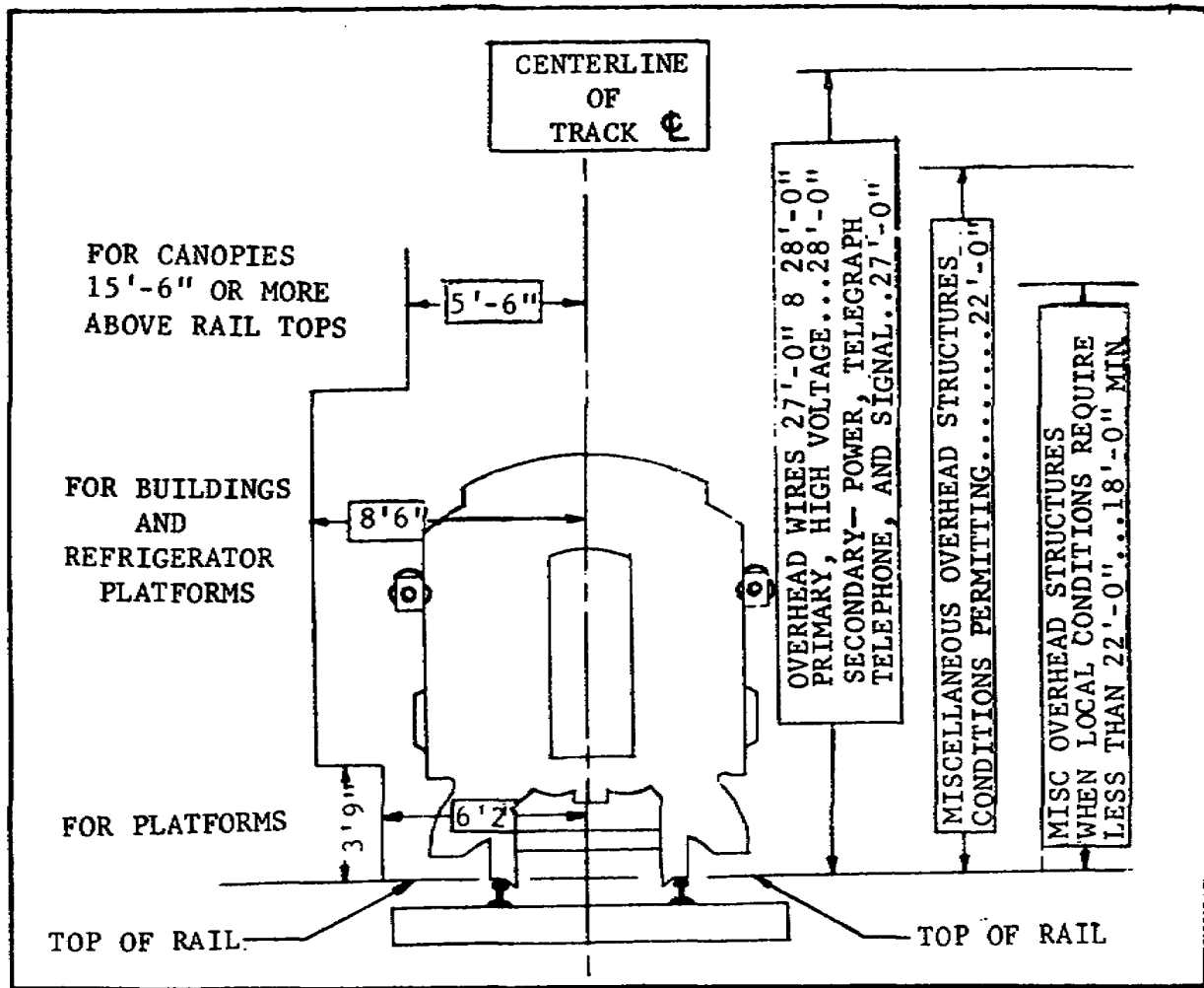
Figure 1.10. Typical Clearances.
