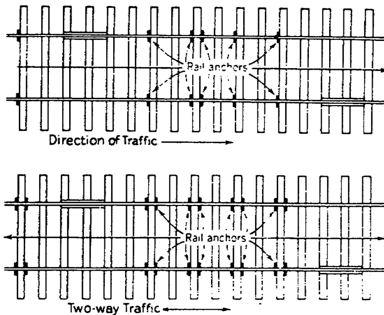
Figure 3.15. Rail Anchors Correctly Located.
