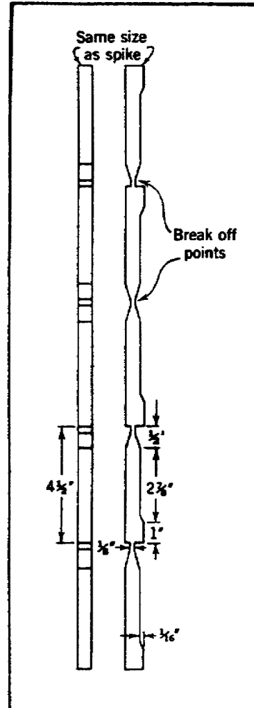
Figure 3.13. Tie Plugs.
