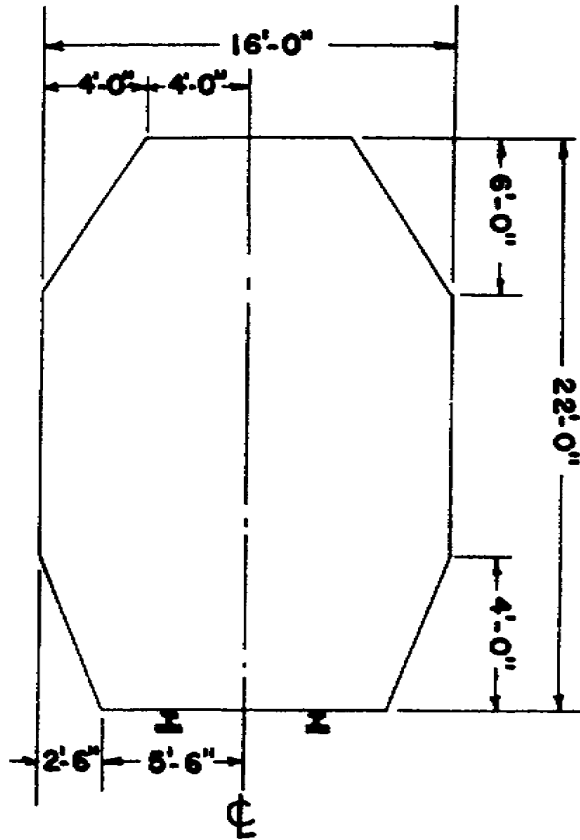
CLEARANCE DIAGRAM FOR RAILWAY BRIDGES
