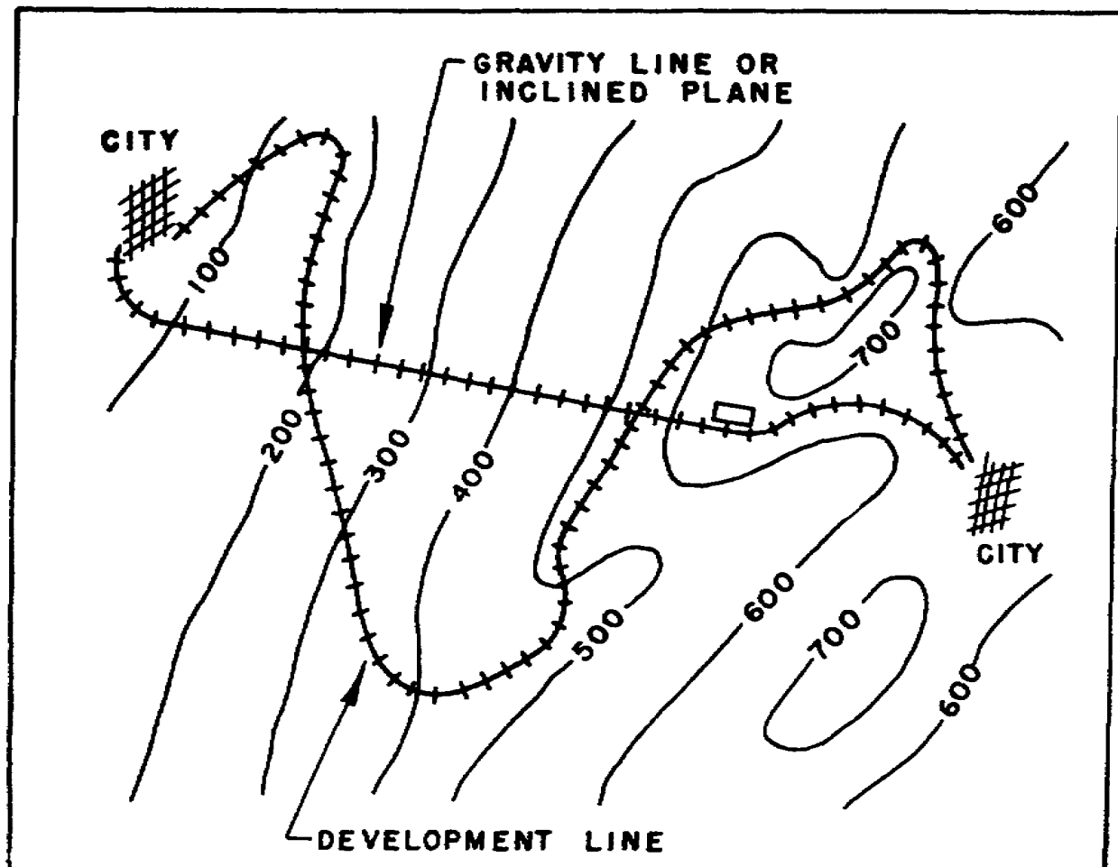
Figure 1.1. Gravity and Development Lines.
