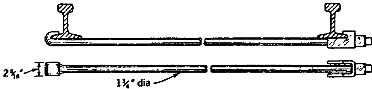
Figure 3.17. Typical Gage Rod.
