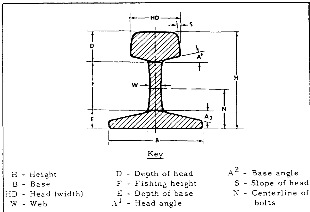
Figure 3.1. Rail Section.
