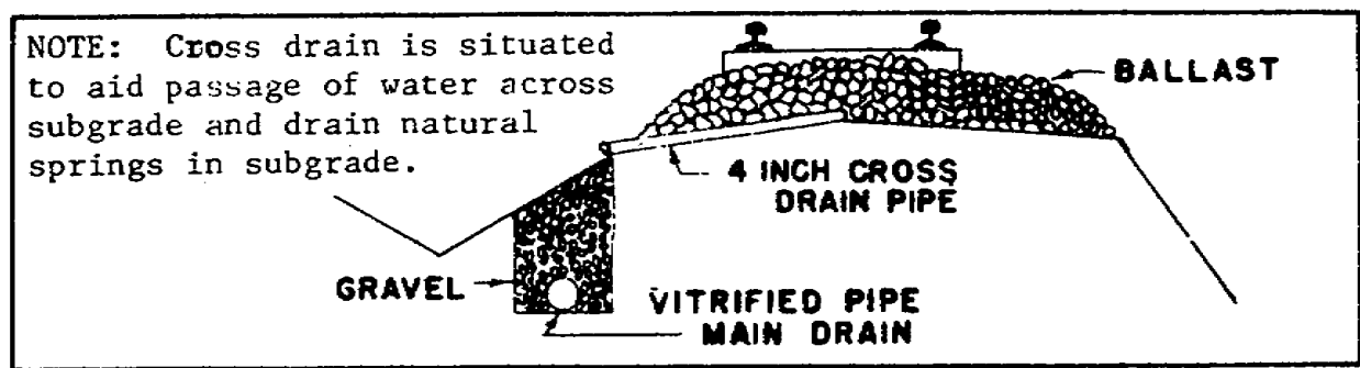
Figure 2.9. Cross Drain Installation With Pipe Drain on Top of Subgrade.
