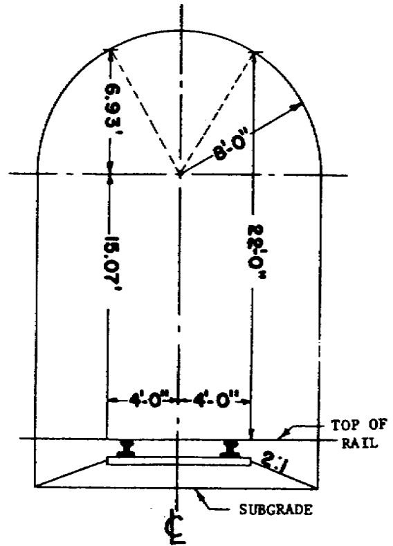
Figure 1.11. AREA Clearance Diagrams.
