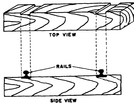
Figure 3.4. Adzed Crosstie.
