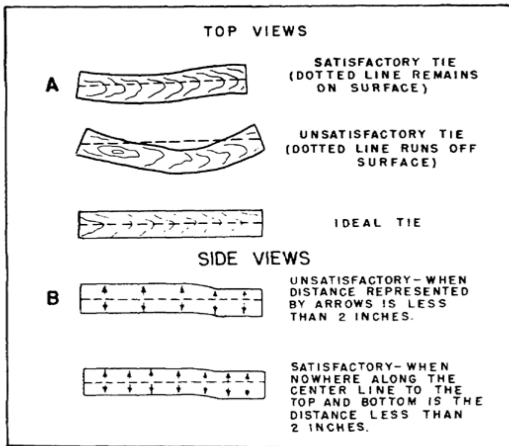
Figure 3.3. Curvature of Crossties.
