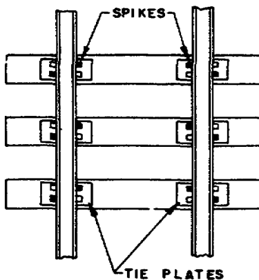
Figure 3.10. Correct Method of Setting Spikes.
