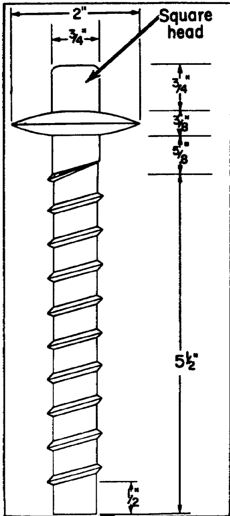
Figure 3.12. Screw Spike.
