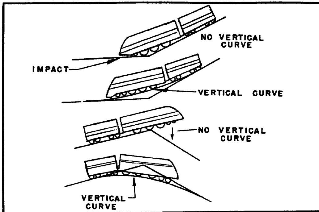
Figure 1.5. Need for Vertical Curves.
