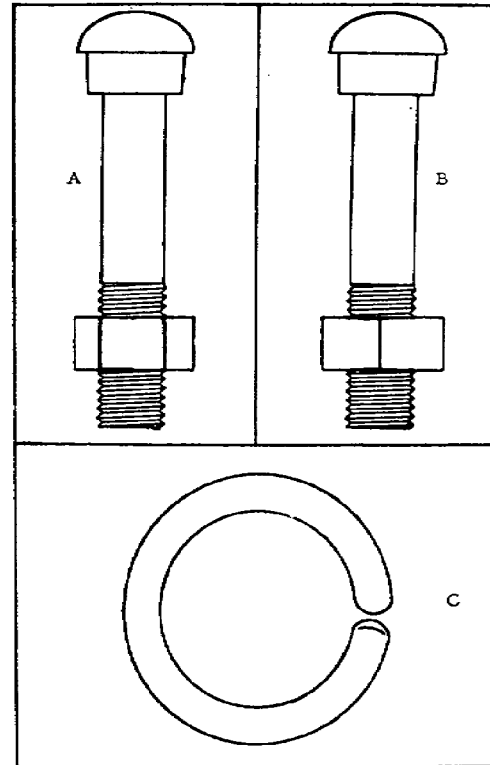
Figure 3.18. Typical Rail Joint Bolts, Nuts, and Spring Lock Washer.
