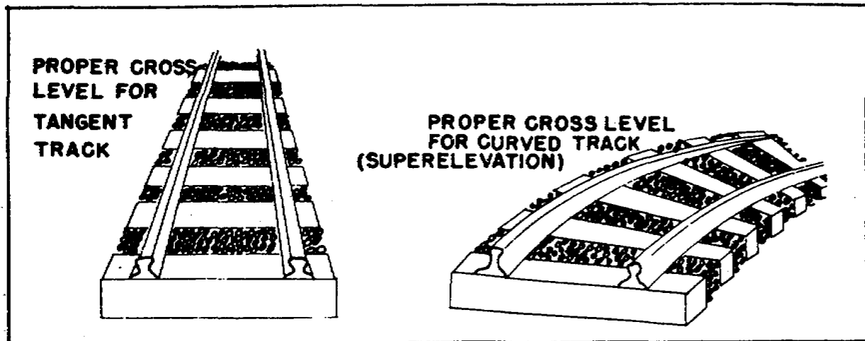
Figure 1.8. Proper Cross Level of Track.
