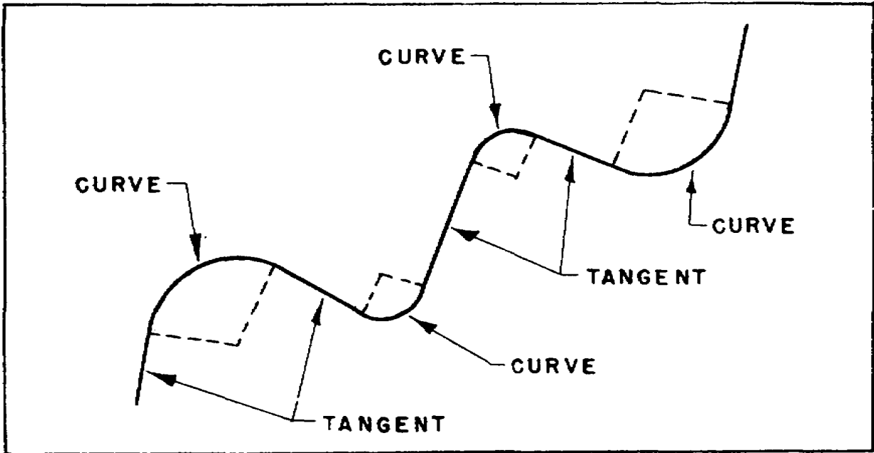
Figure 1.3. Tangents and Curves.
