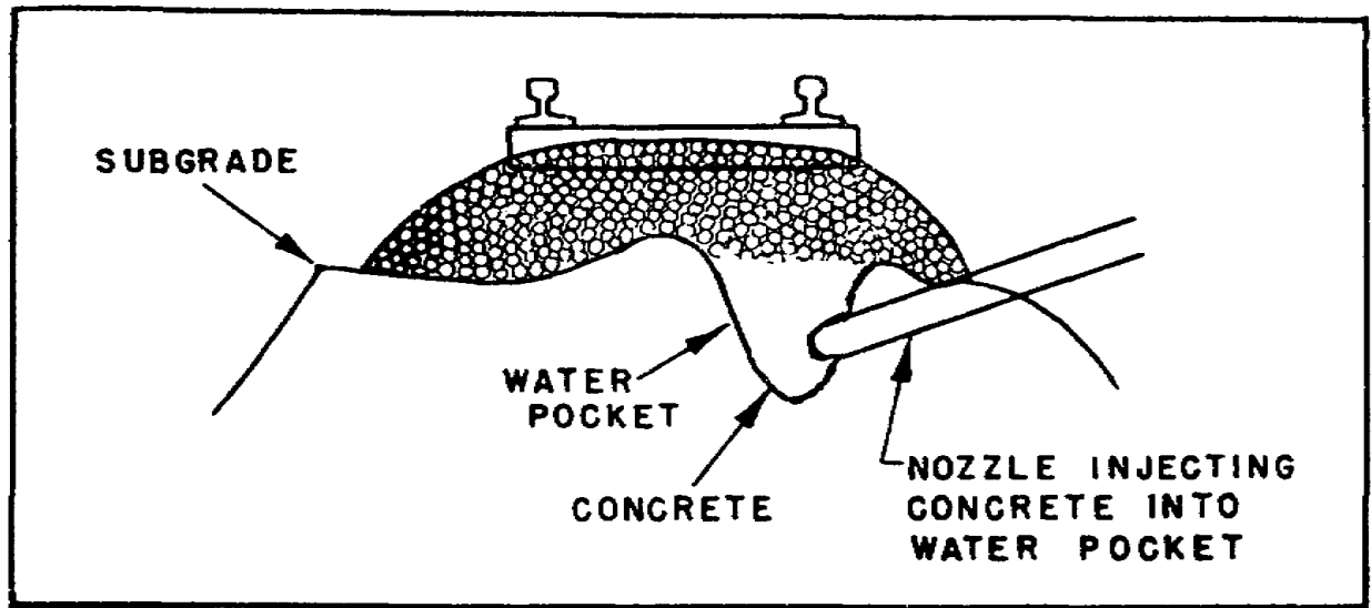
Figure 2.10. Grouting Corrects Water Pocket.
