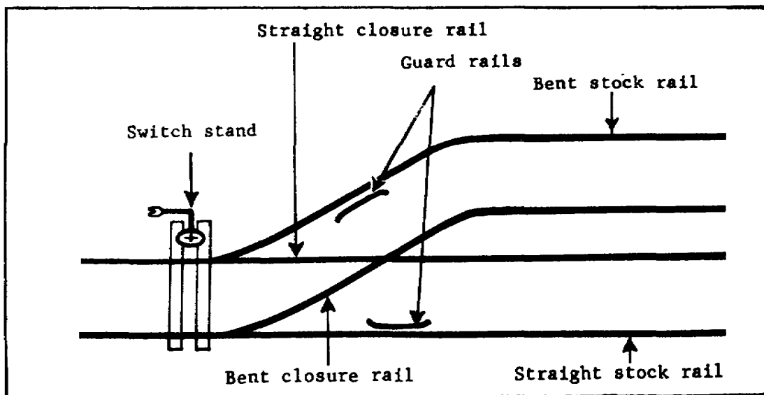
Figure 2.13. Location of Guard, Closure, and Stock Rails.
