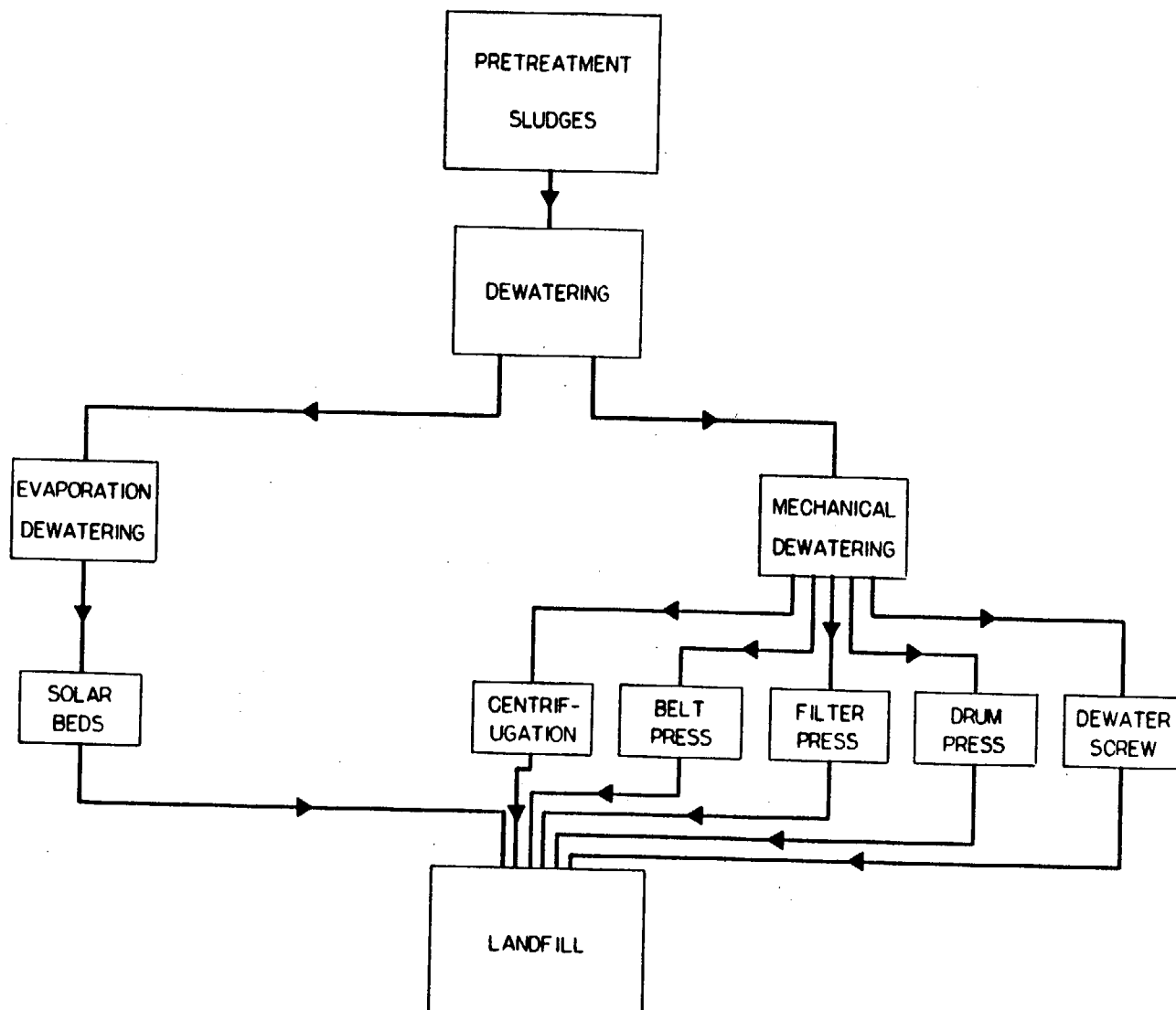
Figure 10-2. Pretreatment sludge disposal.
