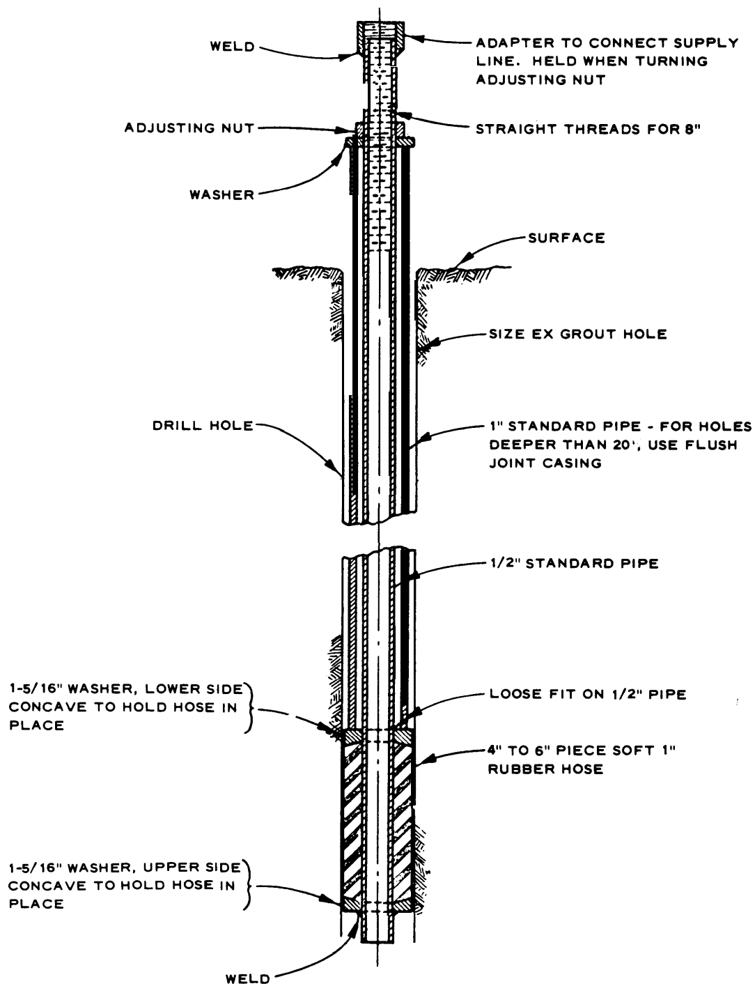
Figure 19. Mechanical packer
