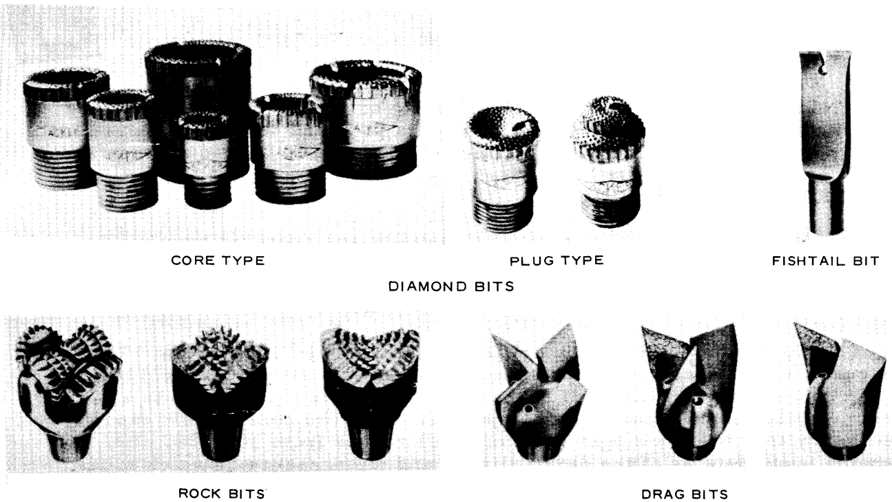
Figure 8. Drill bits
