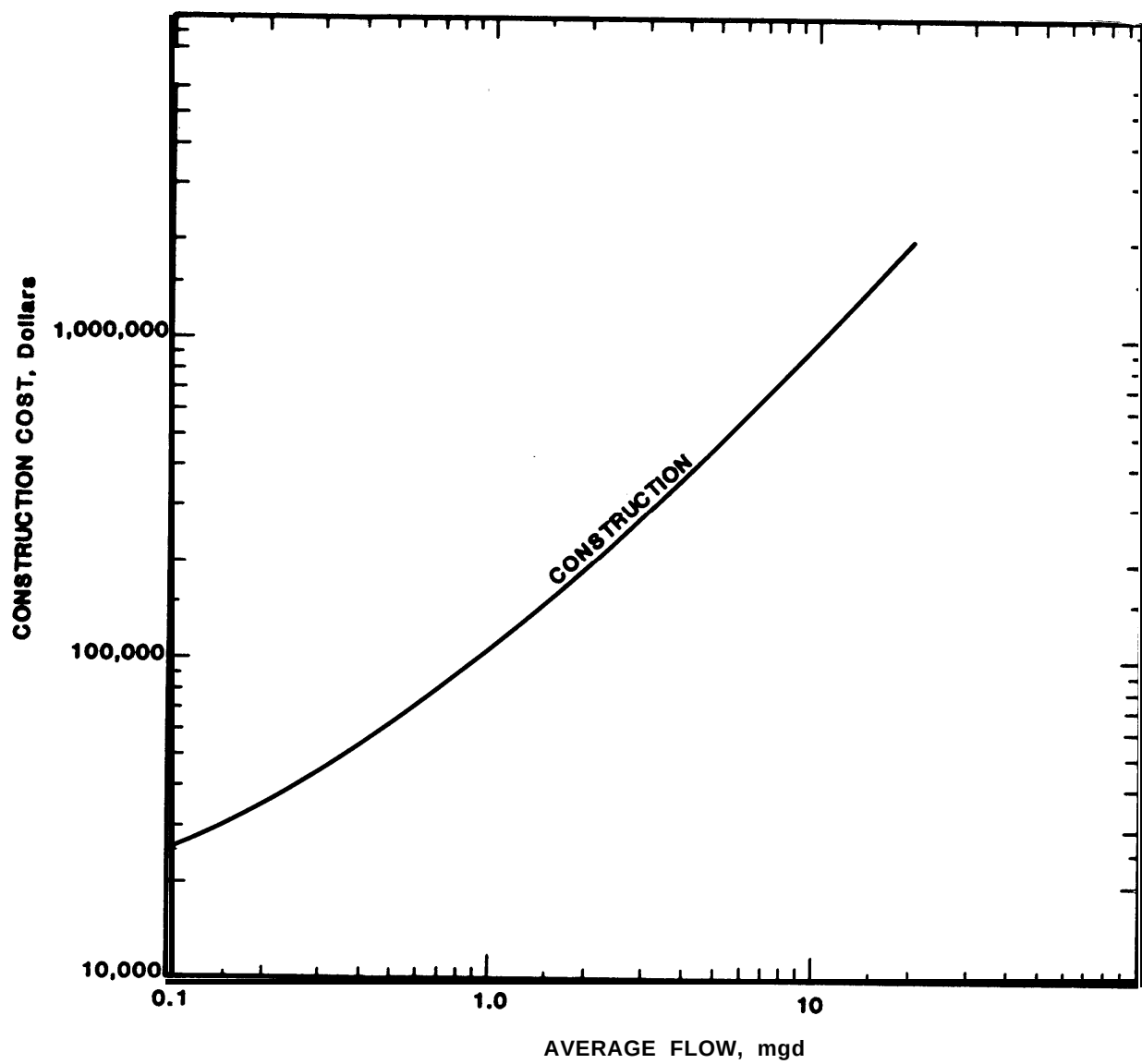
Figure A-15. Cost of sludge drying beds (uncovered).
