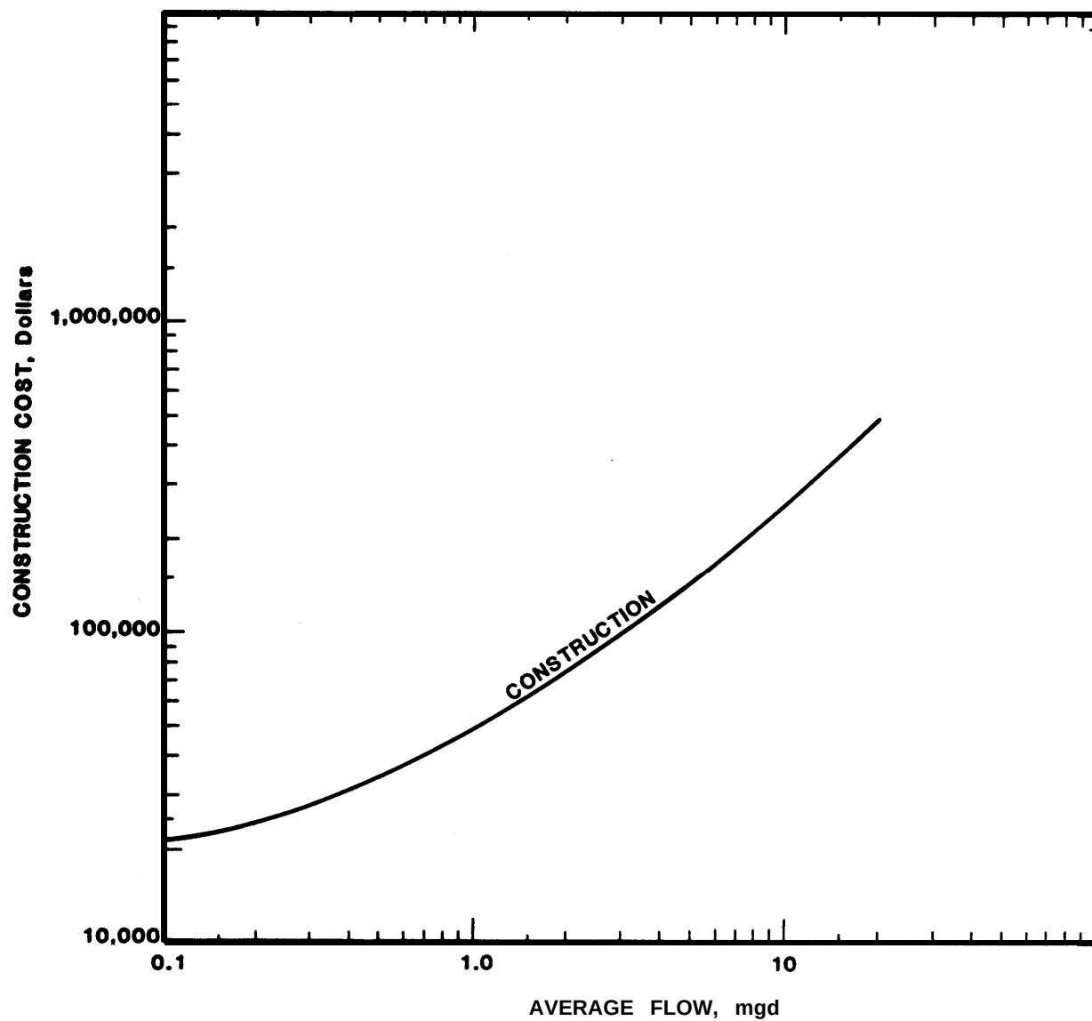
Figure A-4. Cost of \text{FeCl}_3 addition.
