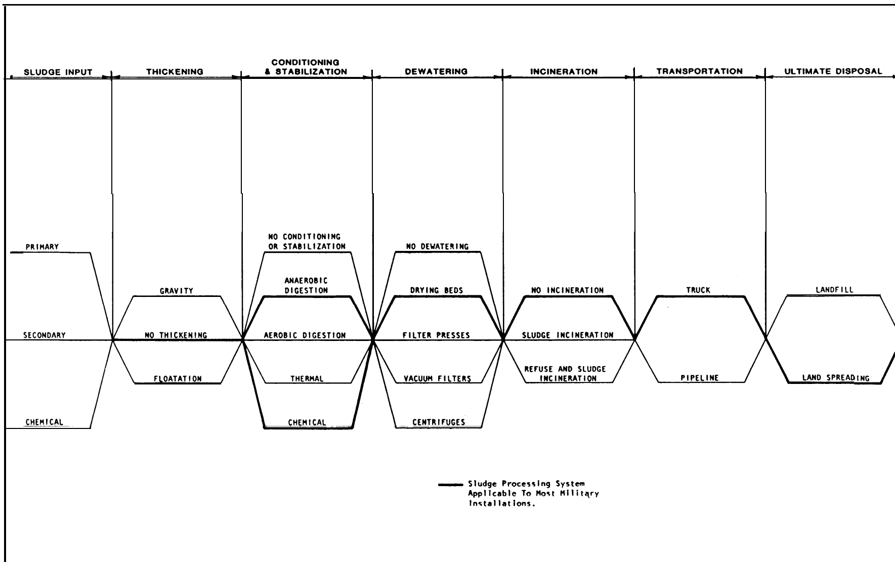
Figure 8-2. Alternative sludge processing systems for military installations.
