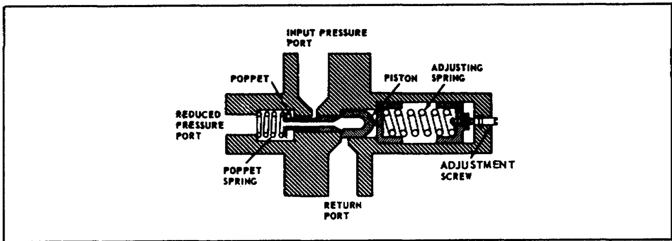
Figure 3-2. Pressure Reducer.
