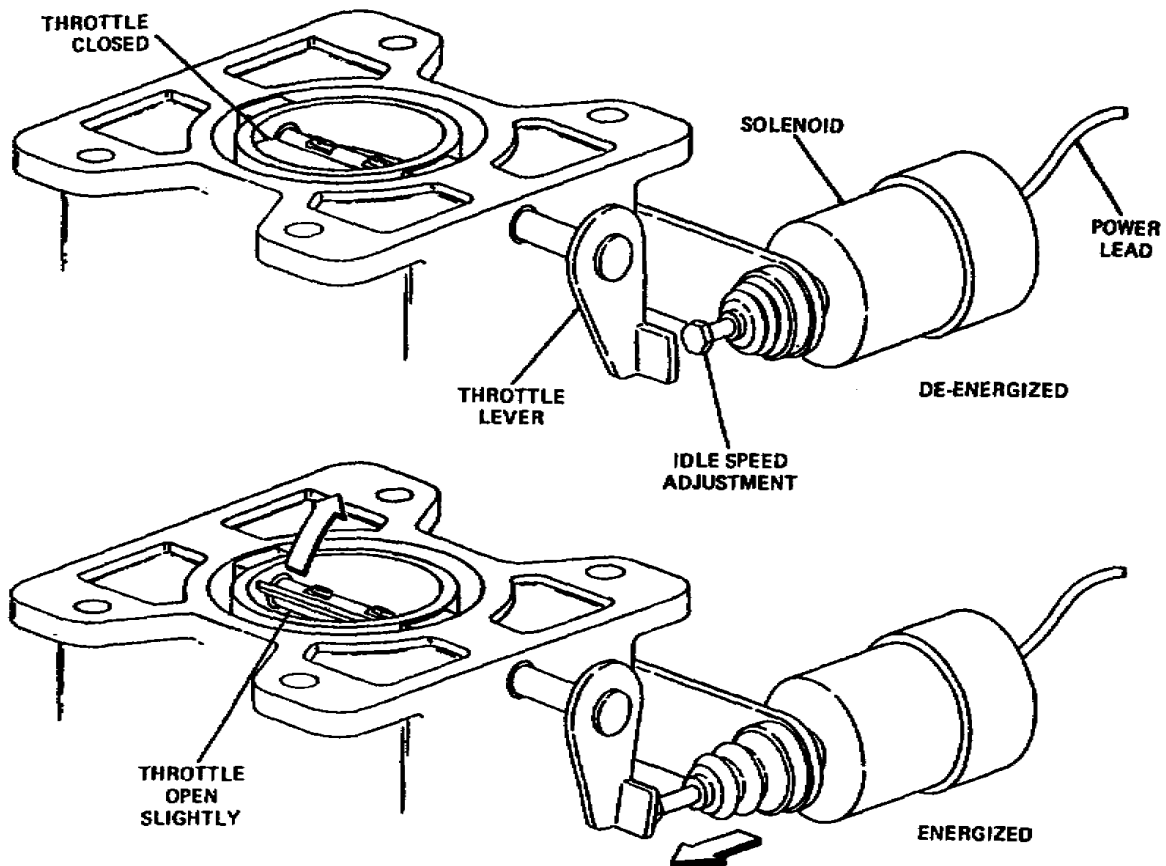
FIGURE 37. ANTIDIESEL/AIR-CONDITIONING SOLENOID OPERATION.
