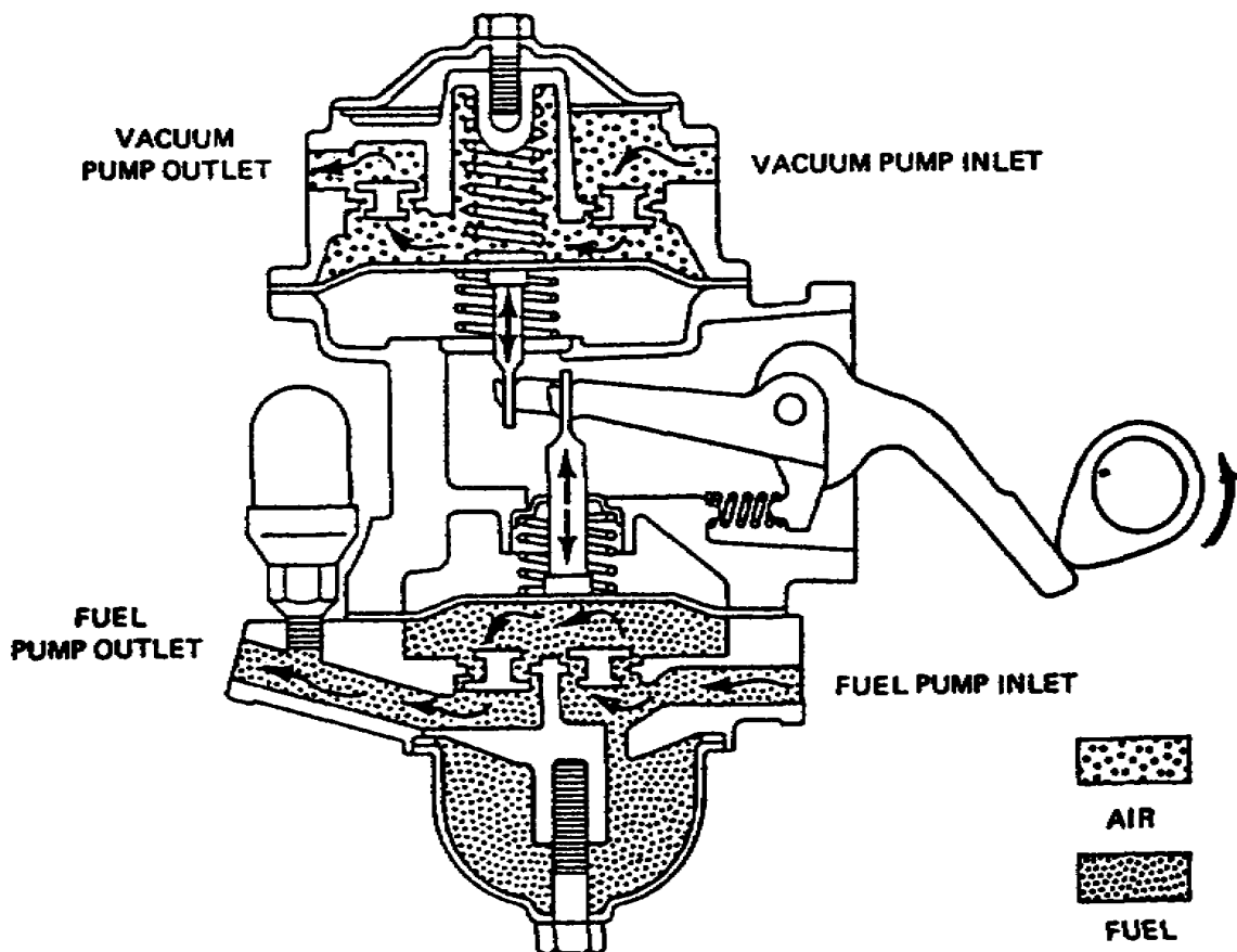
FIGURE 5. DOUBLE ACTION PUMP.
