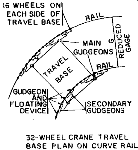
Figure 4 Gage Reduction Diagram (32-Wheel Crane)
