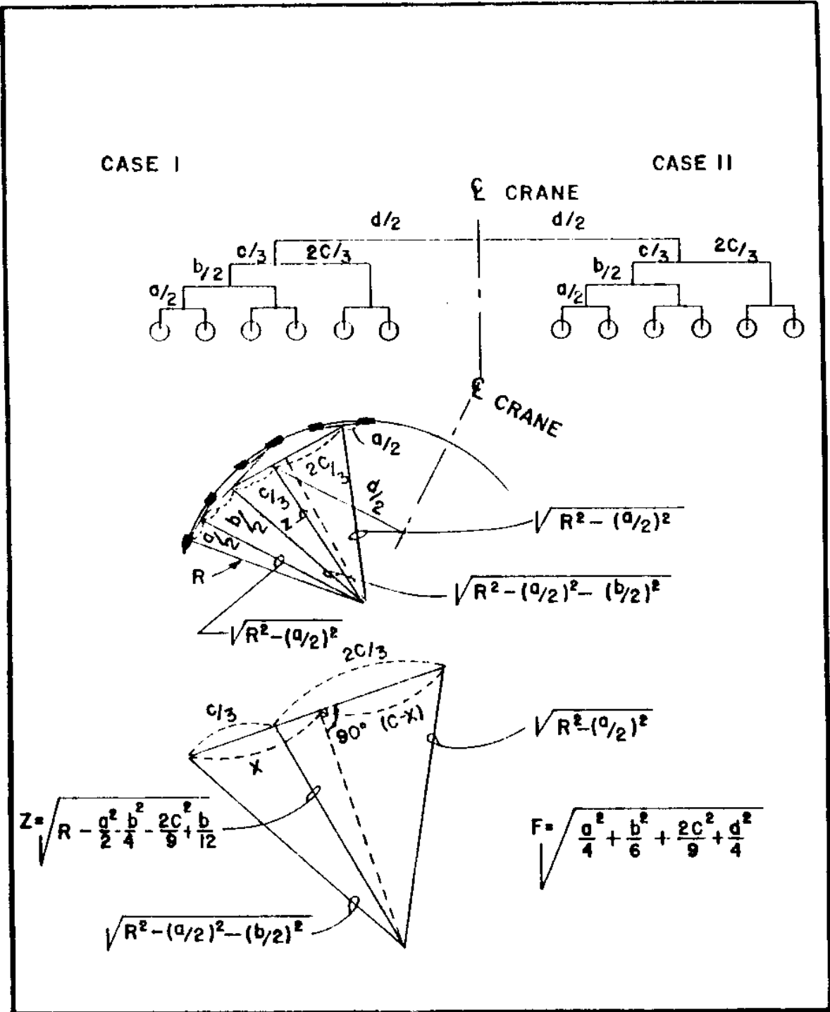
Figure 5 24 Wheel Crane Equivalent Length
