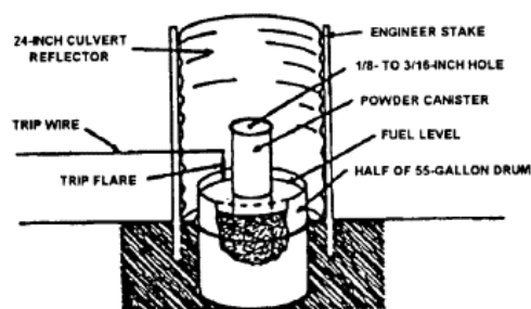
Figure 5-3. Cutaway, showing composition of a Husch flare.
