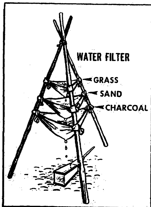
Figure 79. Water filter.
