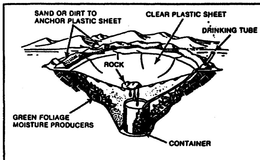
Figure 86. Solar still.
