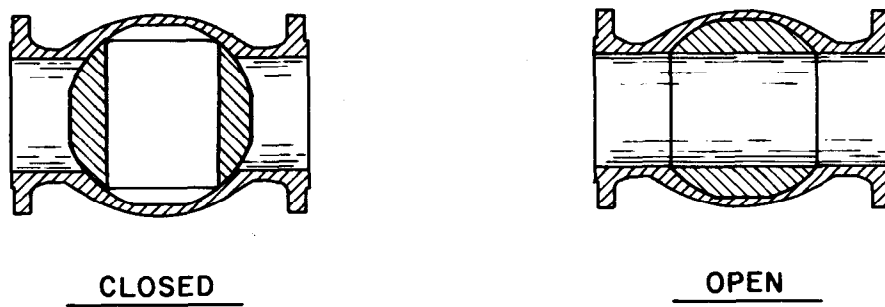
(B) TYPICAL SMALL-DIAMETER BALL VALVE
