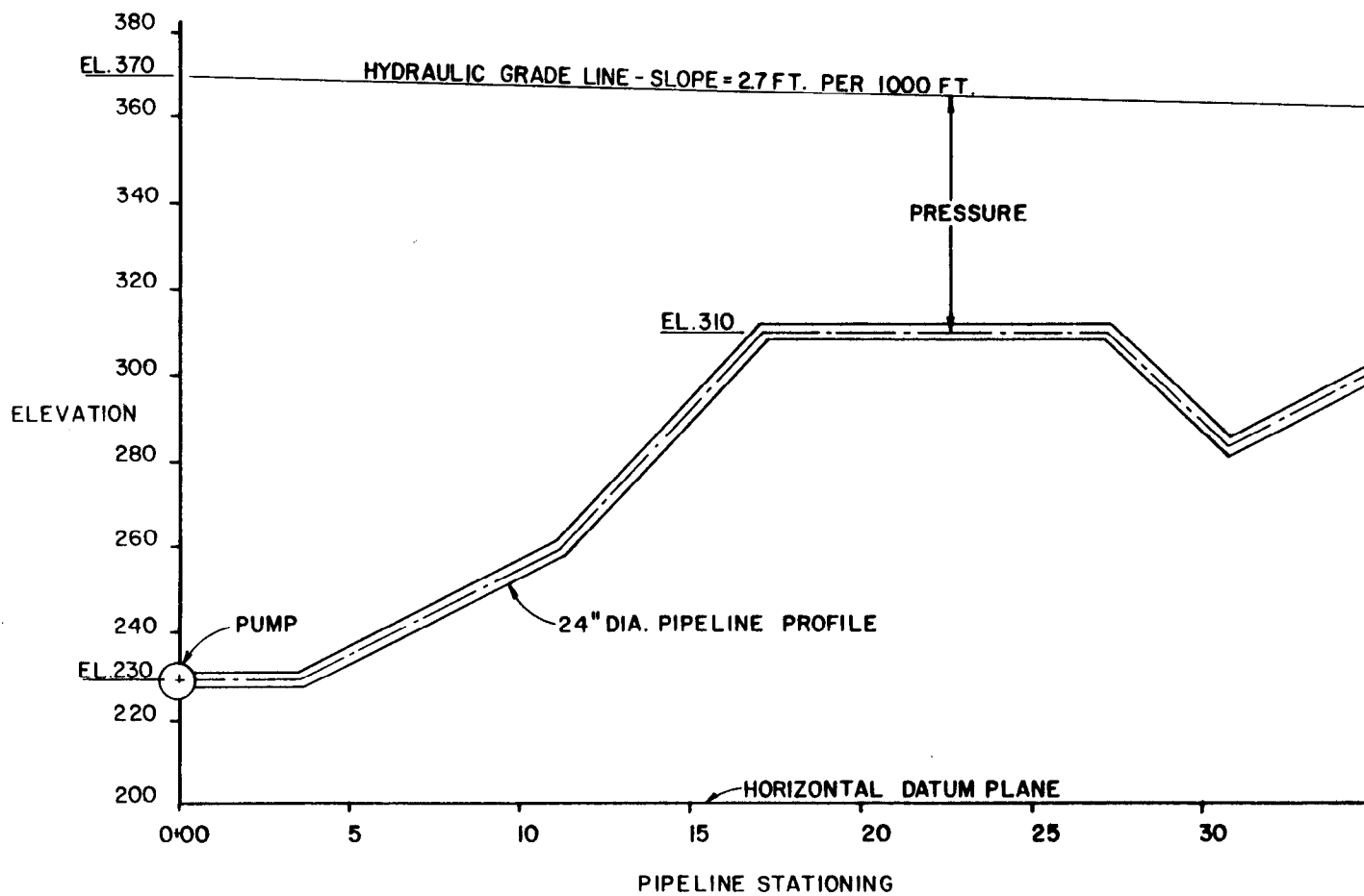
Figure 8-3. Illustration of pipeline pressure.
